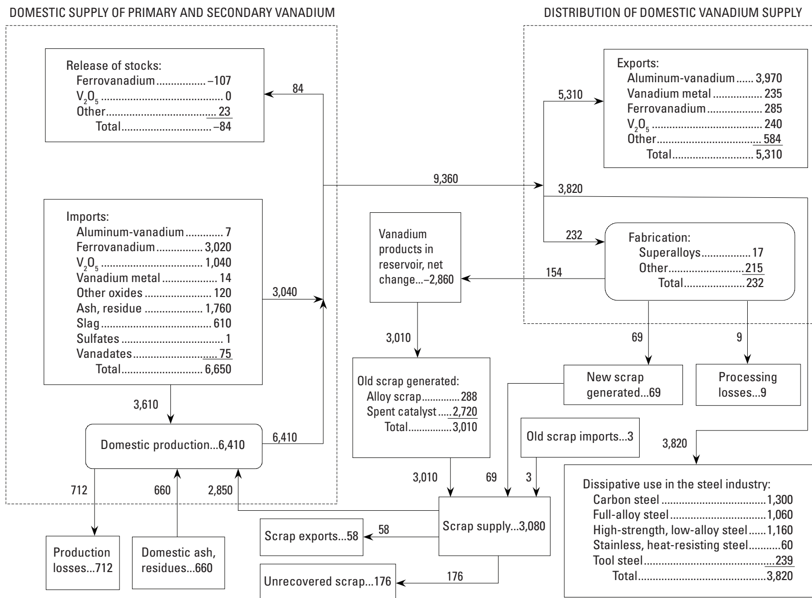
Figure 1. Diagram showing the flow of vanadium contained in various forms in the United States in 2004. Values are in metric tons of contained vanadium. The addition of the parts may not equal the totals owing to independent rounding. Data have been rounded to three significant figures. Stocks refer to producer stocks. There are no Government stocks involved. V 2 O 5 , vanadium pentoxide. Sources: GoldInsider (2006), Matos and Magyar (2006), Magyar (2007b), Vanadium Technology Partnership (2009).
