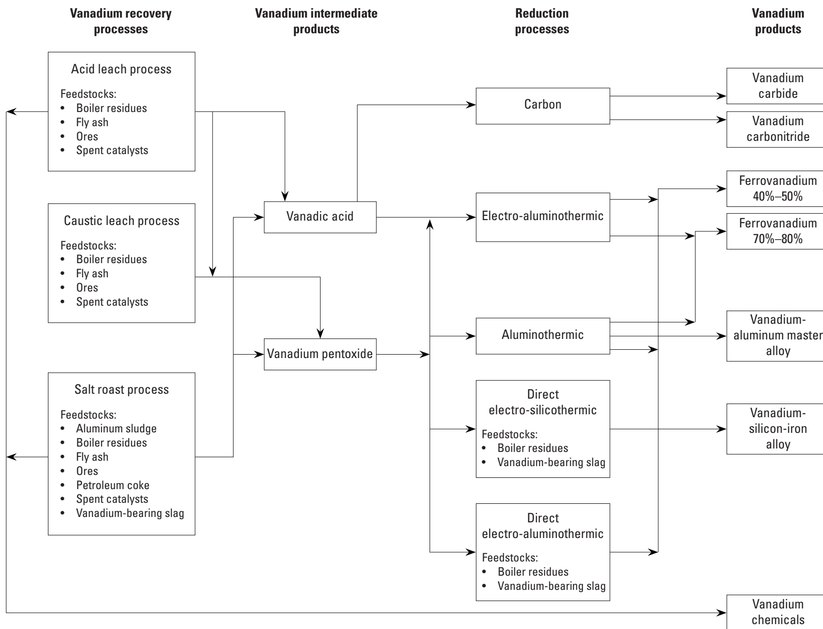
Figure 3. Diagram showing the production flows of vanadium from source through placement into end-use service. Modified from Hilliard (1994, fig. 1).
