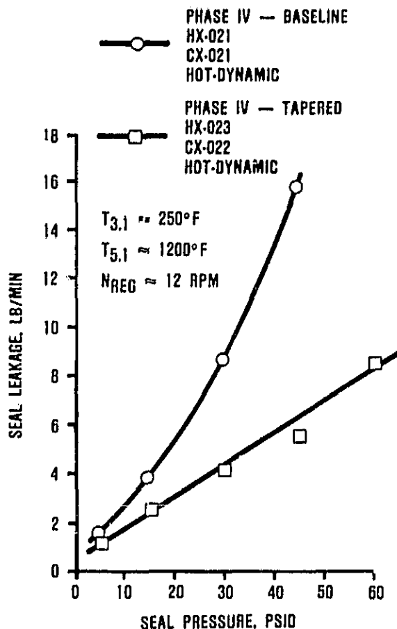
Figure 22. Regenerator Seal Leakage.
