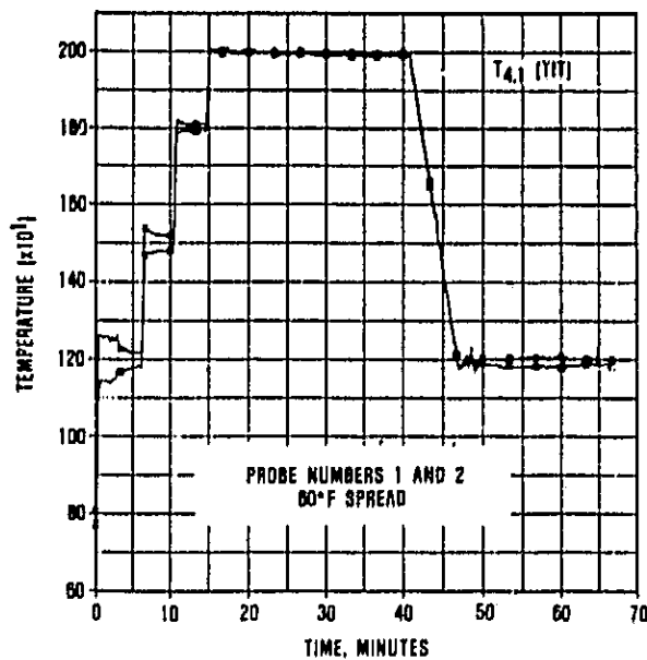
Figure 31. Typical TIT Trace at Idle.
