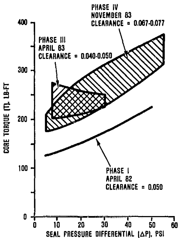
Figure 19. AGT Regenerator Core Torque.
