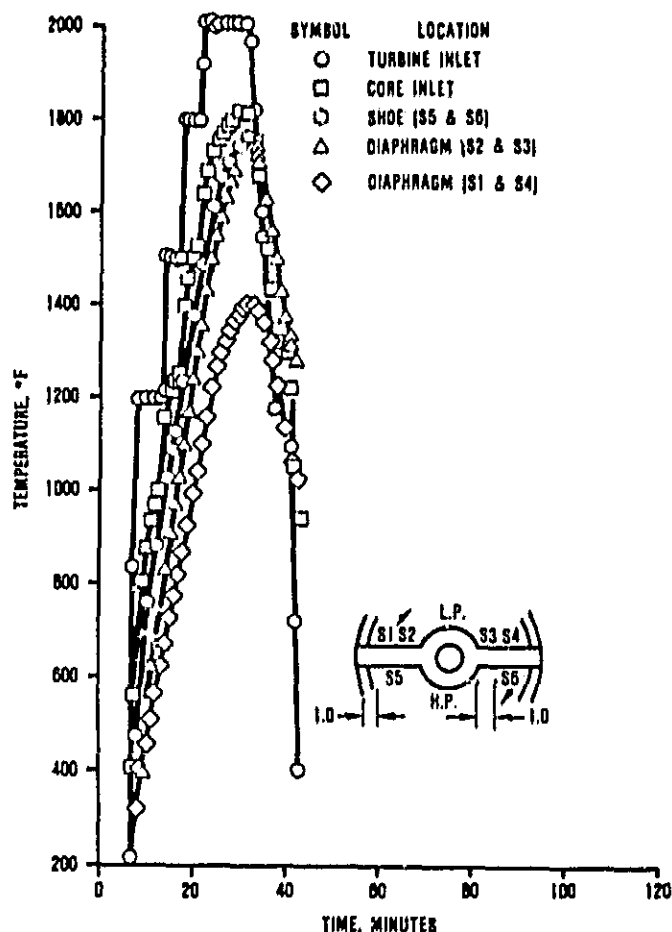
Figure 17. Regenerator Inboard (HOT) Seal Crossarm Temperature.
