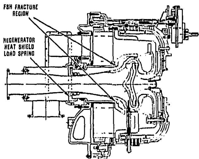
Figure 29. Fracture Region.
