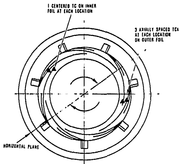
Figure 40. AGT Foil TC Locations.
