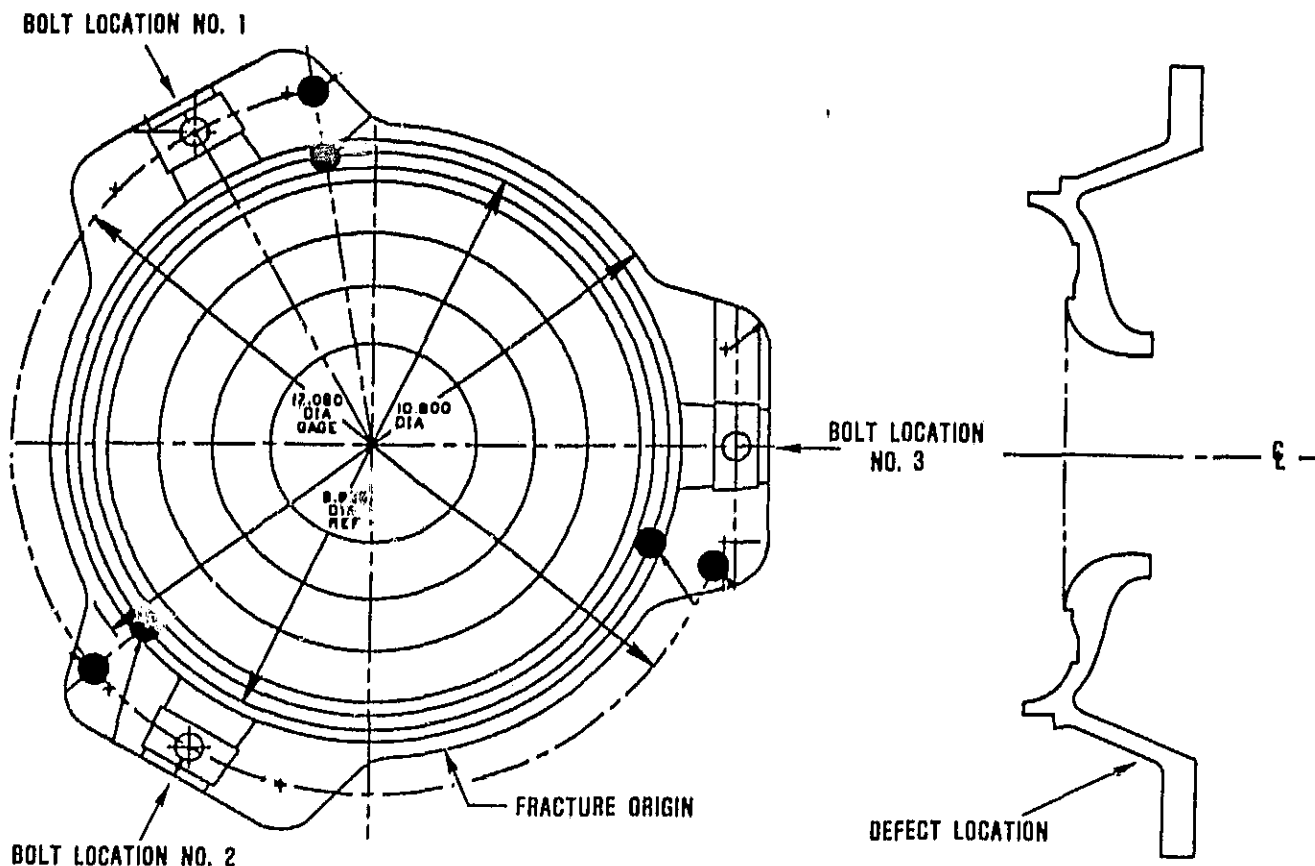
Figure 35. Turbine Shroud Fracture.
