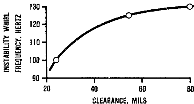
Figure 5. Compressor Backshroud Clearance Effect.
