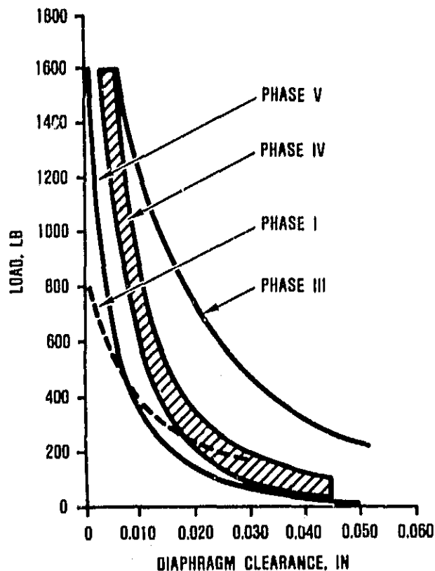
Figure 21. Regenerator Seal Mechanical Load.
