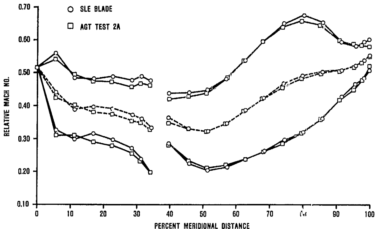
Figure 10. Impeller Blade Loading-Hub.
