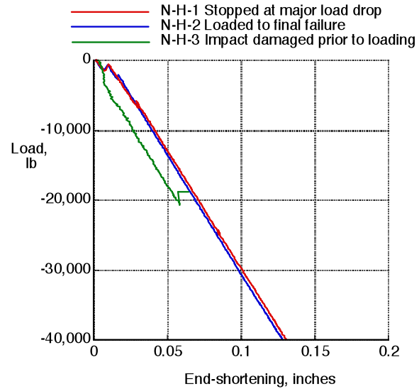
Figure 15. Average axial displacement for struts of type N-H.
