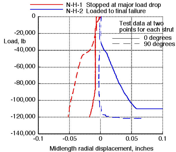
Figure 16. Radial displacement for struts of type N-H.
