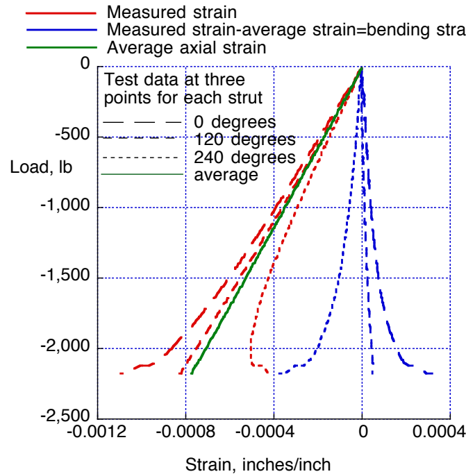
Figure 28. Measured and bending strains for strut N-L-1.
