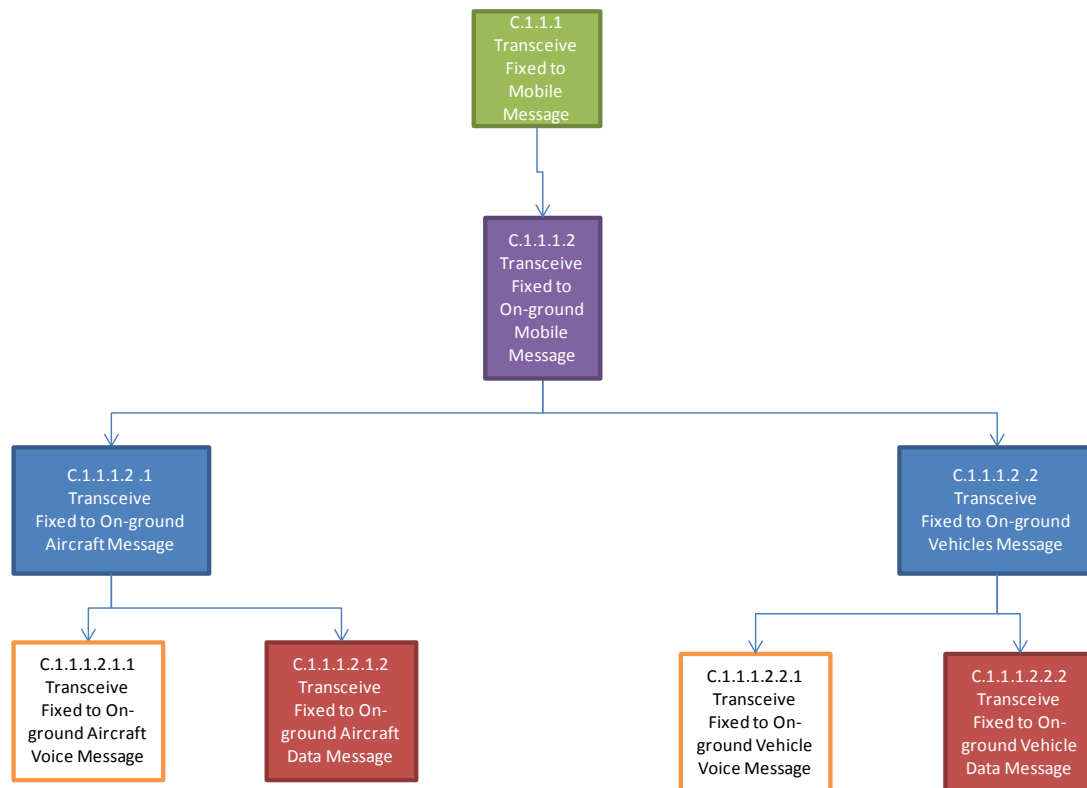
Figure 16.—Decomposition of transceiver fixed-to-mobile message.
