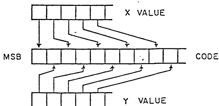
Figure 5b. Bitwise interleaving of x and y coordinates to form the address
