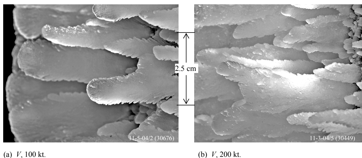
Figure 4.—Evaluating the effect of velocity on feather appearance. MVD , 185 to 190 \mu\text{m} ; n_0 , 0.50.
