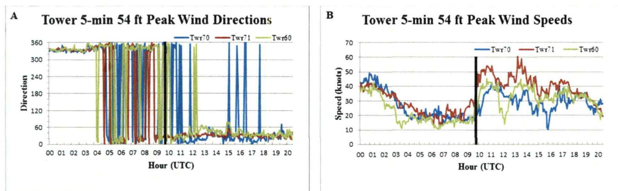
Figure 7. The peak wind direction (A) and speed (B) on 21 October 2007. The black vertical line in both charts highlights the first northeast \geq 35 kt peak wind occurrence from Tower 71. The earlier peak wind speeds between 0000-0230 UTC were associated with the cold front that had moved through VAFB.
