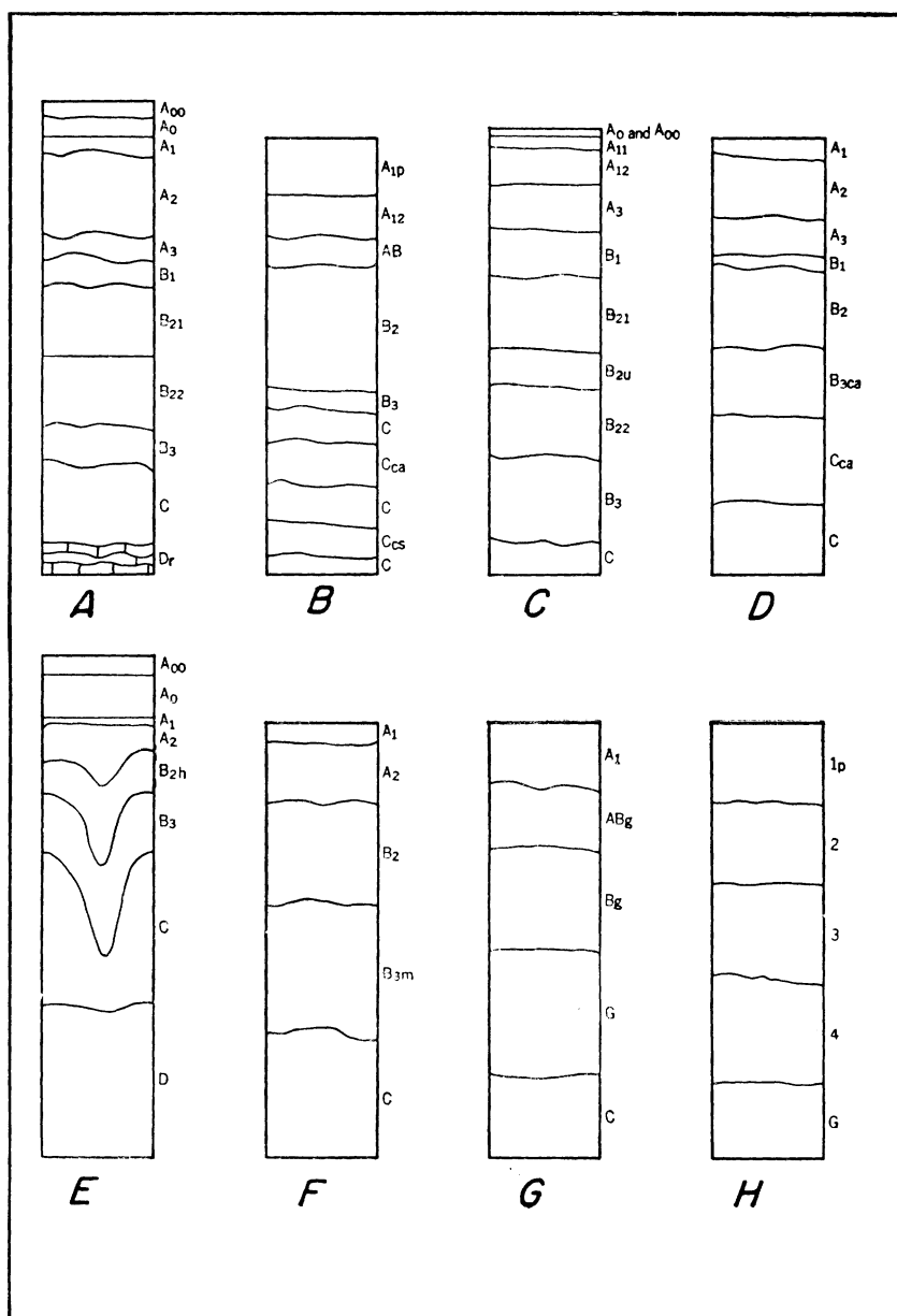
FIGURE 28.—Hypothetical profiles to illustrate a few horizon designations: A, Gray-Brown Podzolic; B, Chernozem (cultivated); C, Latosol; D, solodized-Solonetz; E, Podzol; F, Planosol; G, Humic Gley (Wiesenboden); H, Bog.
