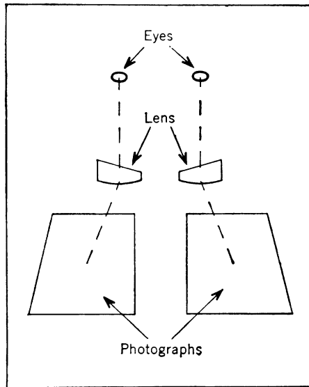
FIGURE 13.—Sketch showing the essentials of the design of a lens stereoscope. The thin edges of the lenses are inside.
