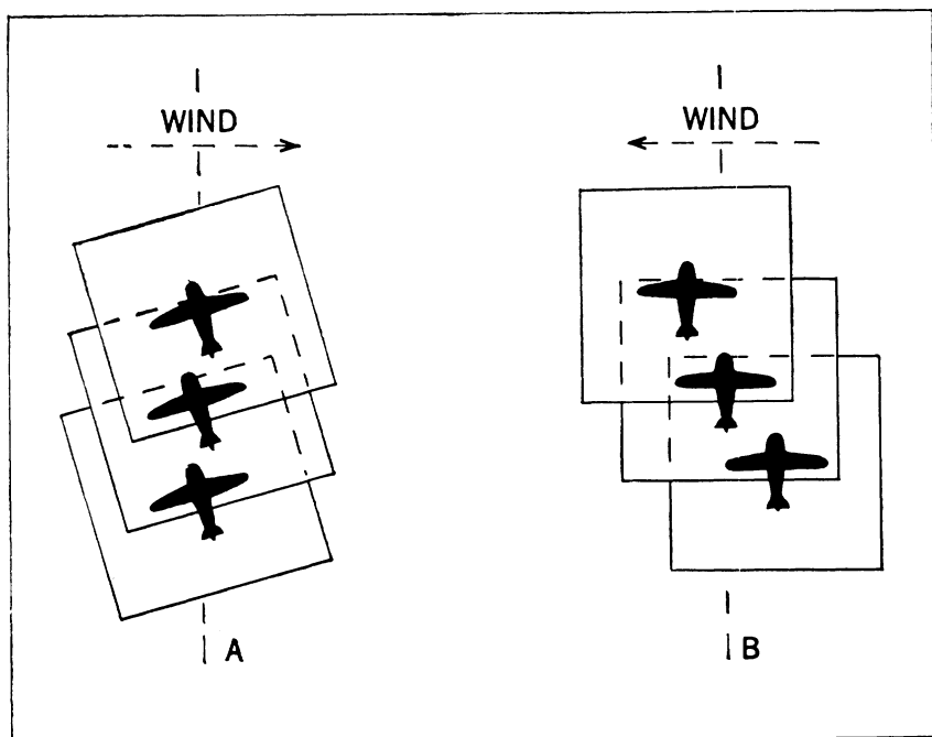
FIGURE 10.—Sketches showing irregularities in aerial photographs: A, from crabbing; B, from drift.
