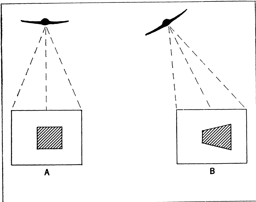
FIGURE 8.—Sketches showing distortion of a square in an aerial photograph because of tilt: A, normal; B, with tilt.
