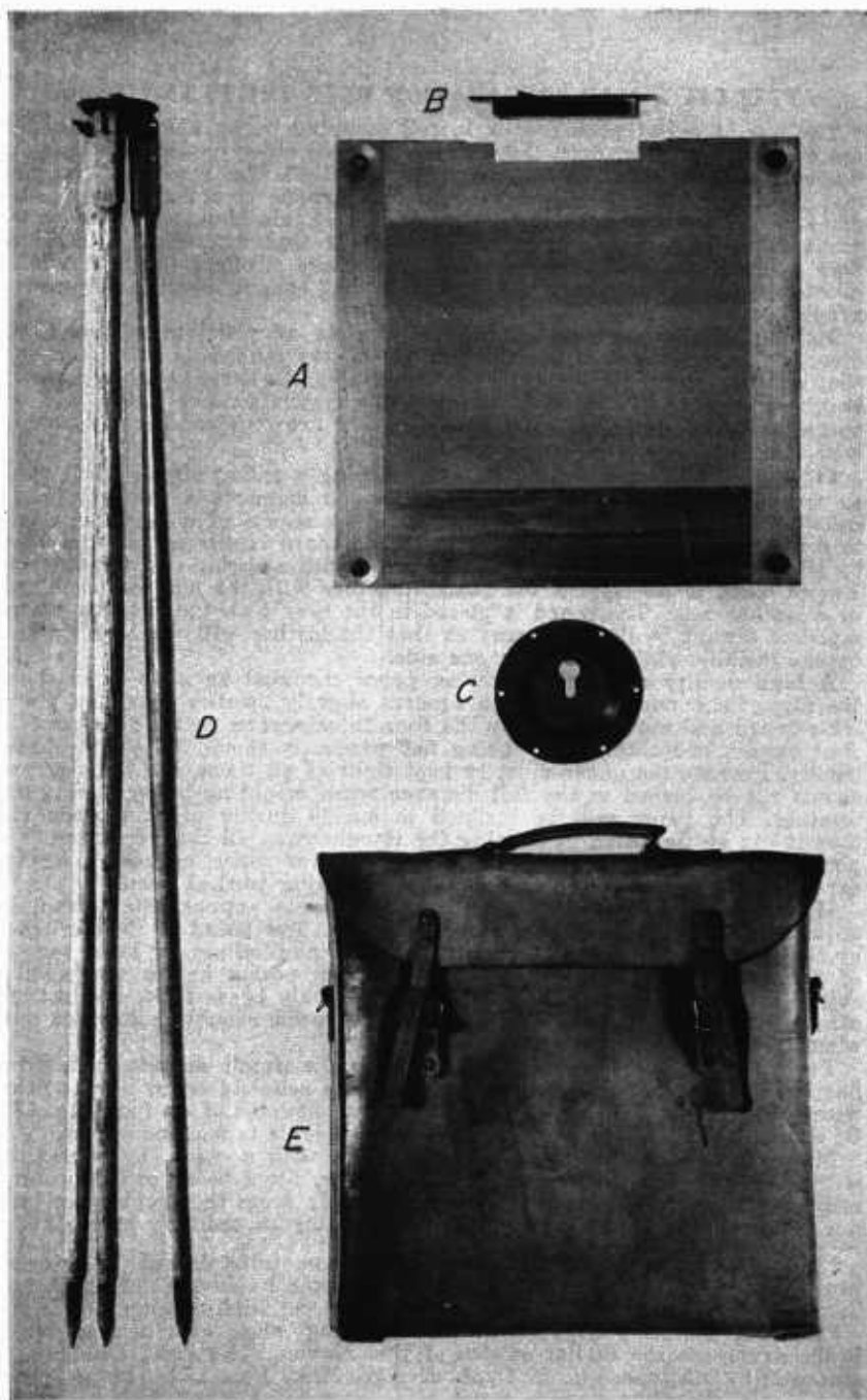
FIGURE 56.—Plane table, unassembled: A , Board; B , compass; C , head; D , tripod; and E , case.
