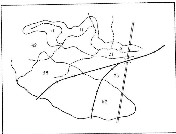
FIGURE 20.—The omission of soil boundaries causes serious errors.
