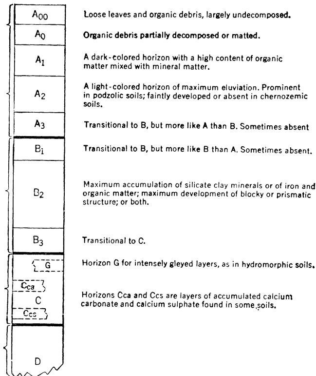
FIGURE 27.—A hypothetical soil profile having all the principal horizons. It will be noted that horizon B may or may not have an accumulation of clay. Horizons designated as C ca usually appear between B 2 and C. The G may appear directly beneath the A.
