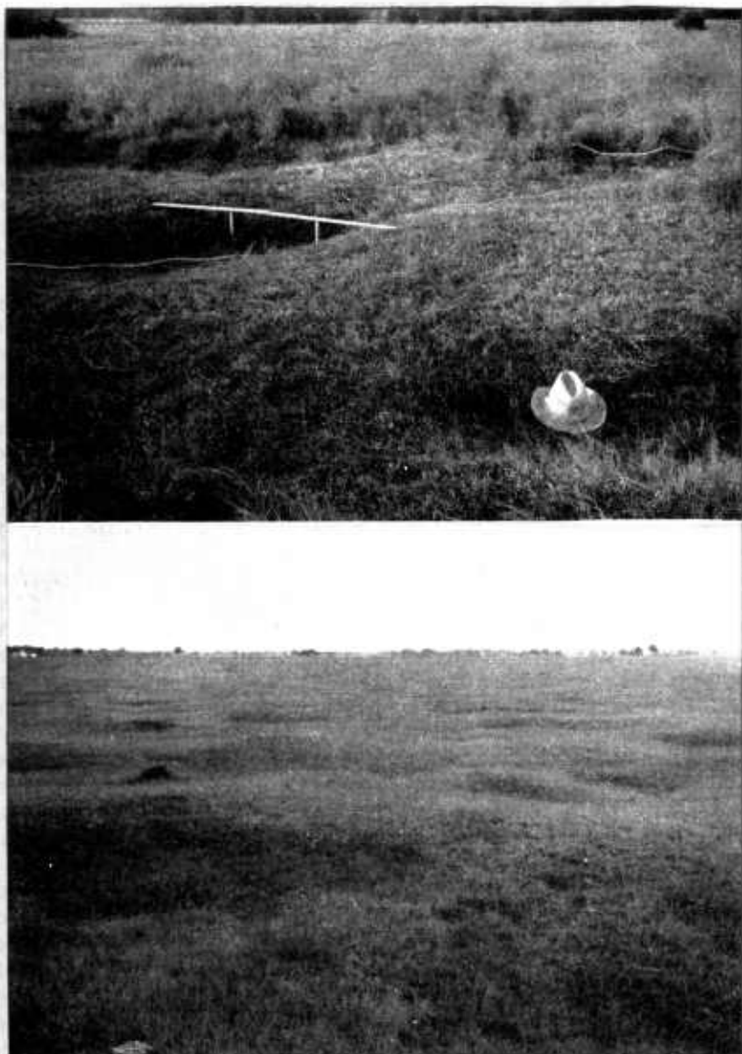
FIGURE 24.—Characteristic microrelief of the gilgai type: Upper, on Irving clay near Millican, Tex.; and lower, on Bell clay 15 miles southwest of College Station, Tex.
