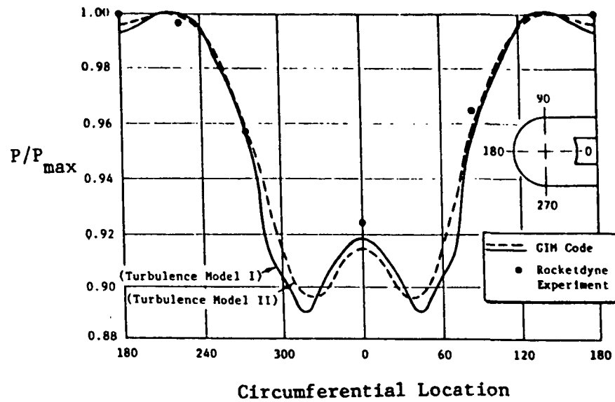
Fig. 49 Comparison of Computed Static Pressures to Measured Static Pressures in Bowl
