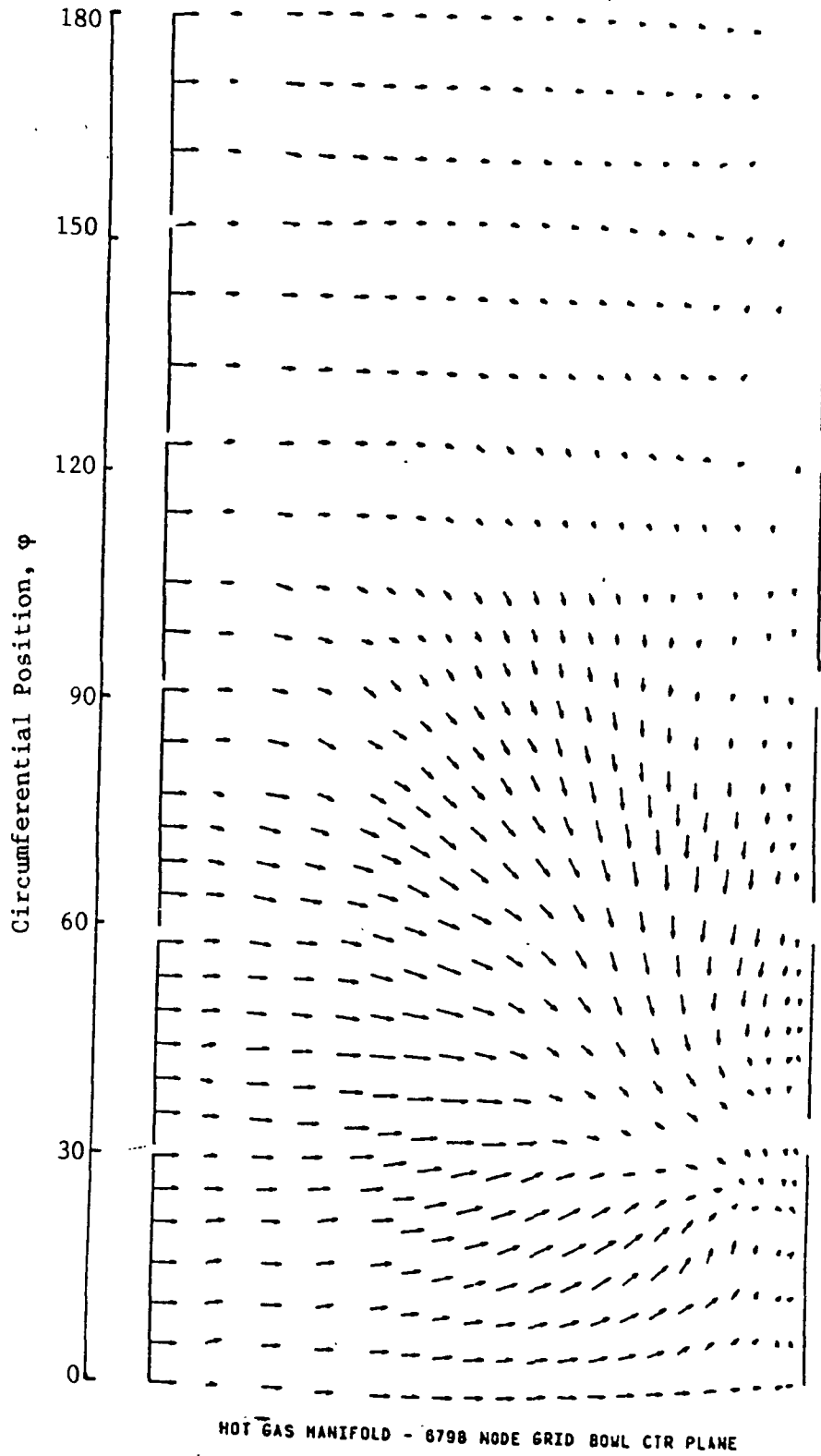
Fig. 46 HGM Bowl Center Plane Velocity Field
