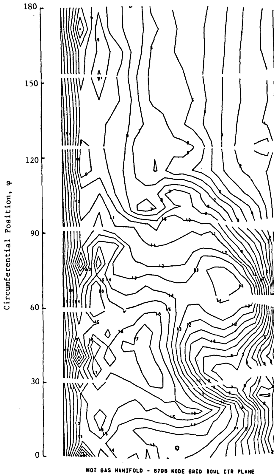
Fig. 48 HGM Bowl Center Plane Mach Number Contours
