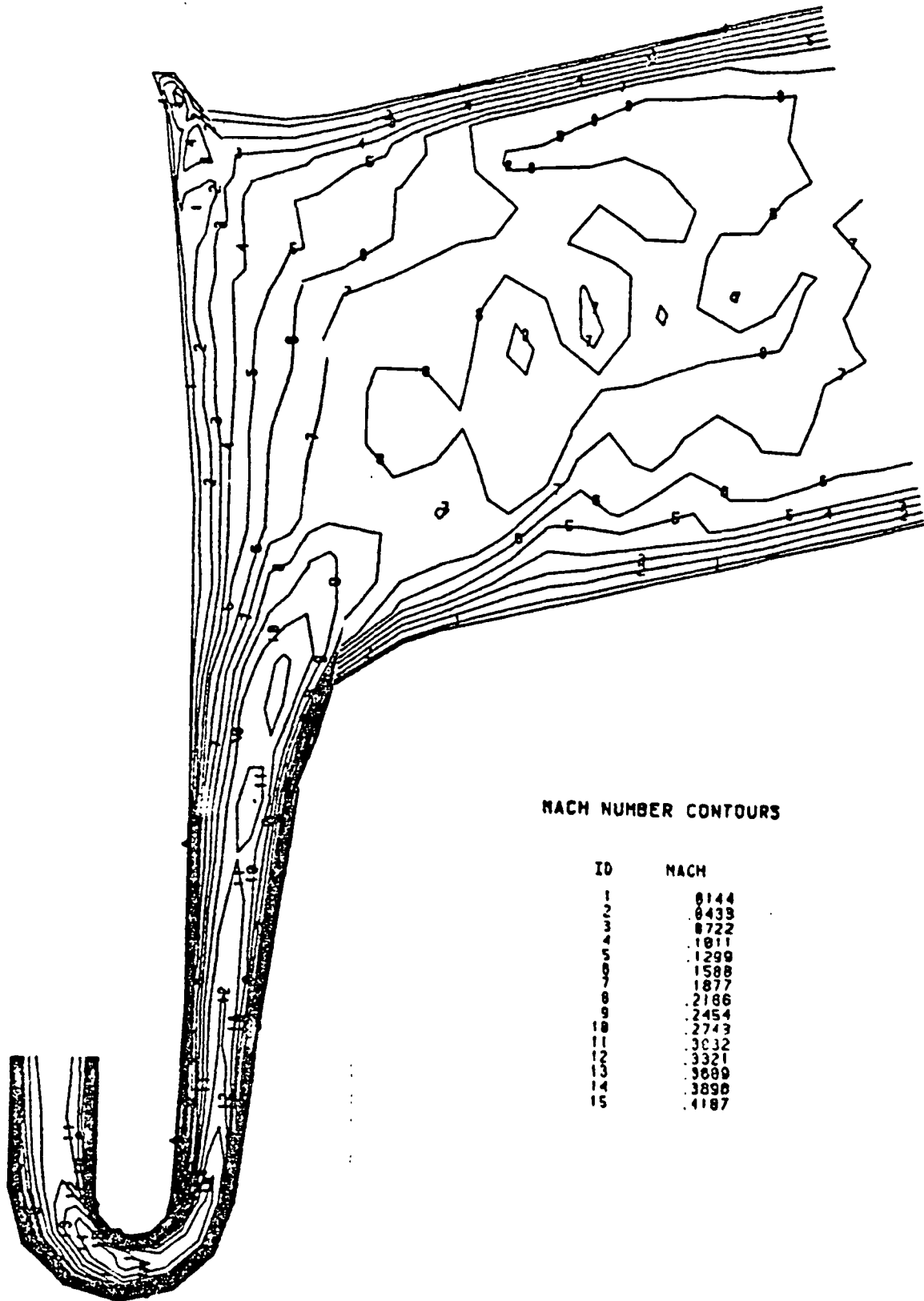
Fig. 57 DFNUS HGM Nominal Configuration Mach Number Contours
