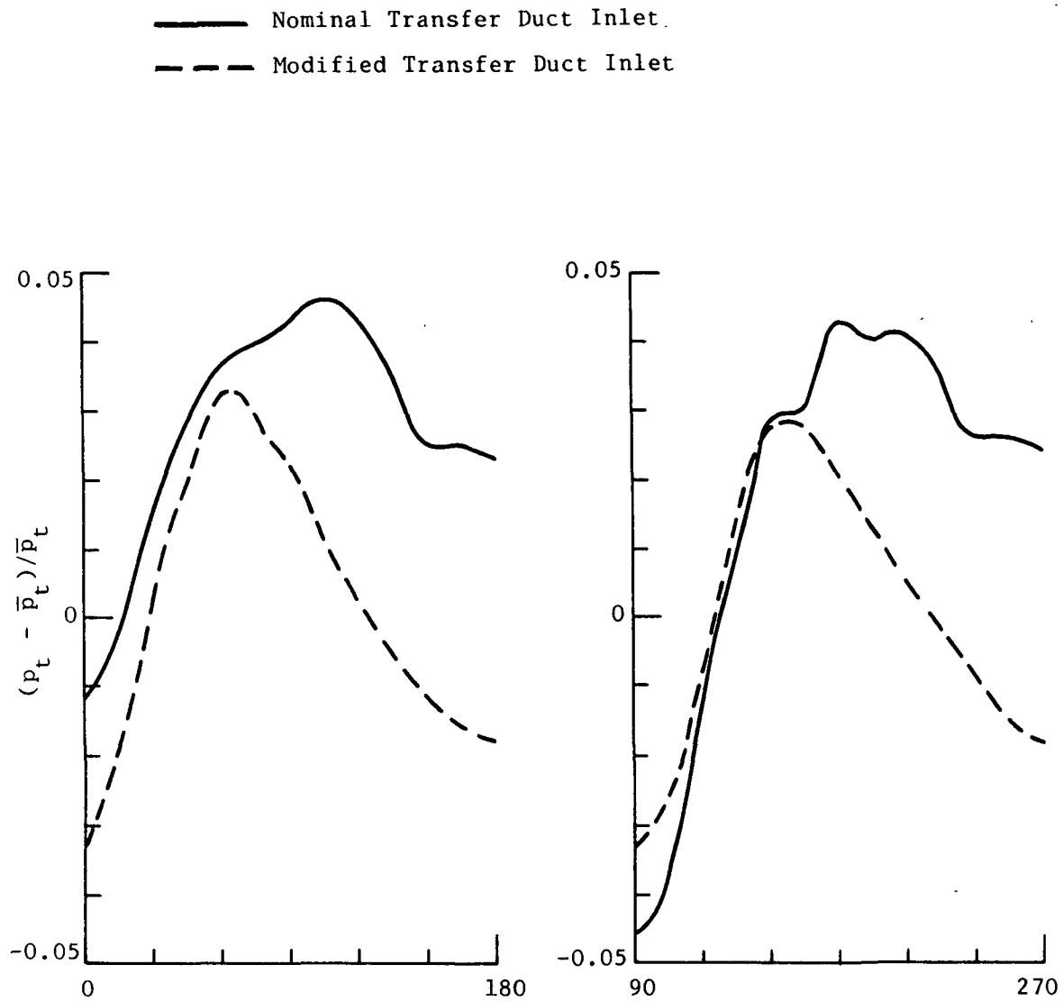
Fig. 75 Transfer Duct Exit Total Pressure Profile
