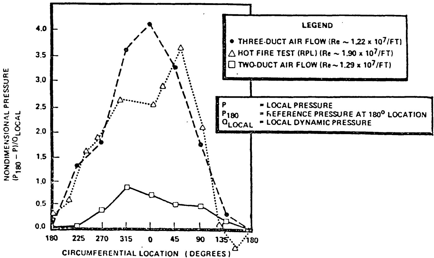
Fig. 10 Static Pressure Variation Downstream of 180-deg Turn
