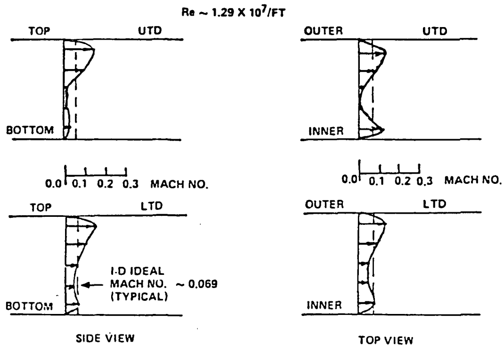
Fig. 14 Engine-Scaled Two-Duct Manifold Mach Number Profiles Along Duct Major Axes (100 Percent Power Level Condition)
