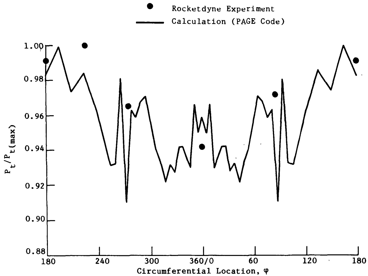
Fig. 67 DFNUH HGM, Bowl Inlet Total Pressure
