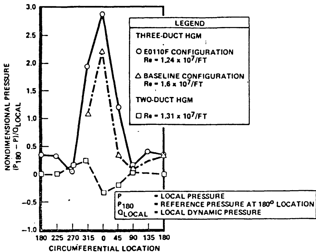
Fig. 11 Total Pressure Variation Downstream of Turnaround Duct 180-deg Turn
