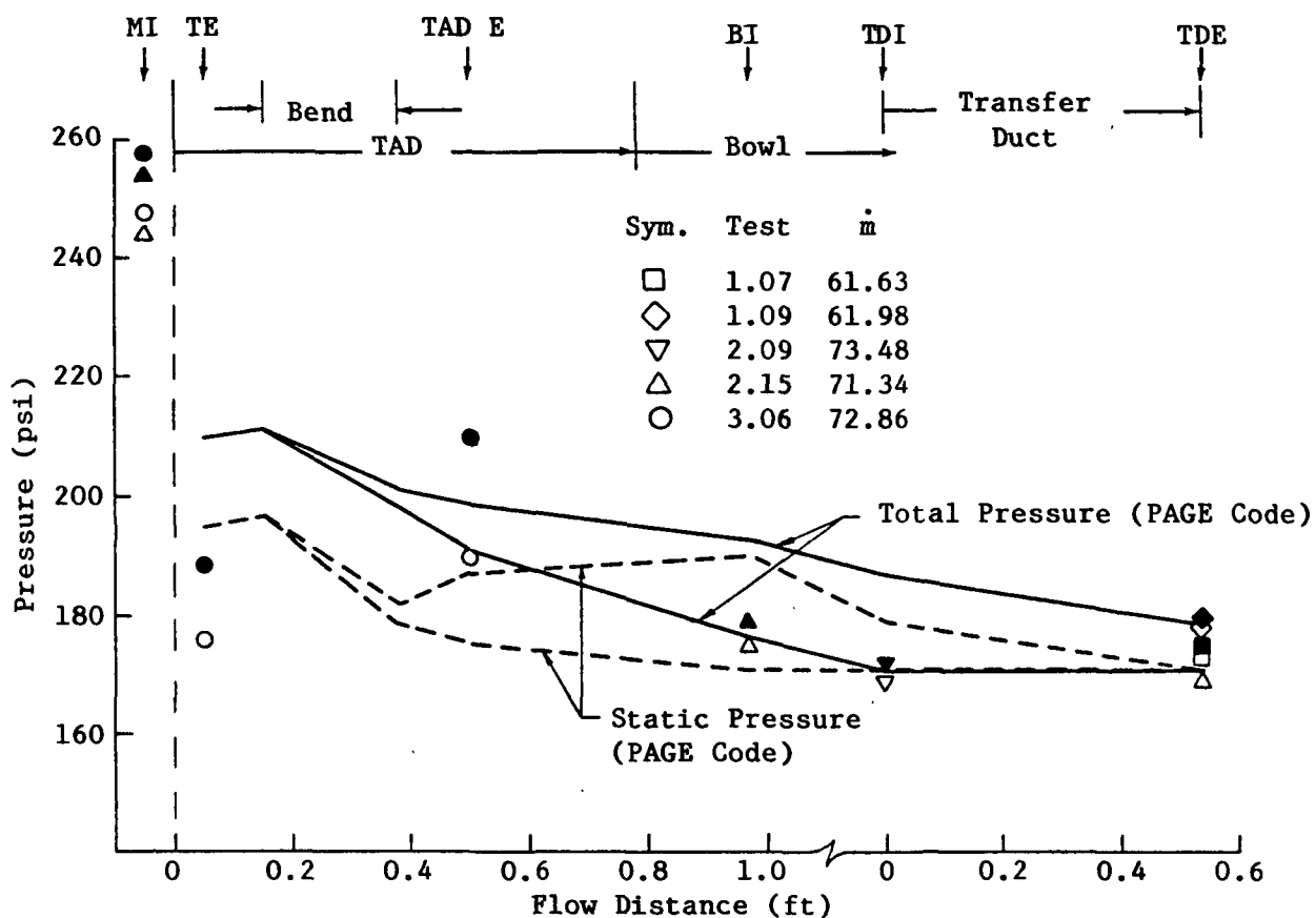
Fig. 63 DFNUH HGM Averaged Pressure Along Flow (Open symbols indicate static pressure; solid symbols indicate total pressure).
