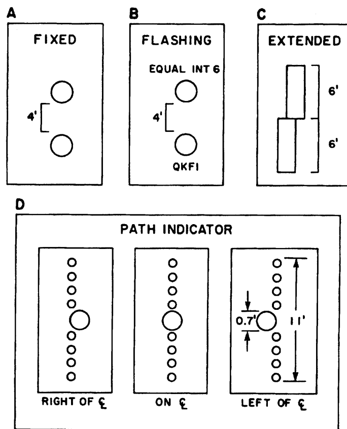
Fig. 2. Four parallax range light configurations.
