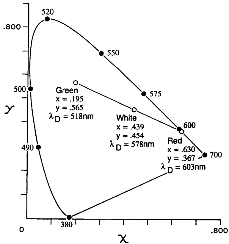
Fig. 13. The CIE Chromaticity Diagram showing the locus of stimuli displayed by the variable light beam. The fixed beam displayed only the white reference stimulus.
