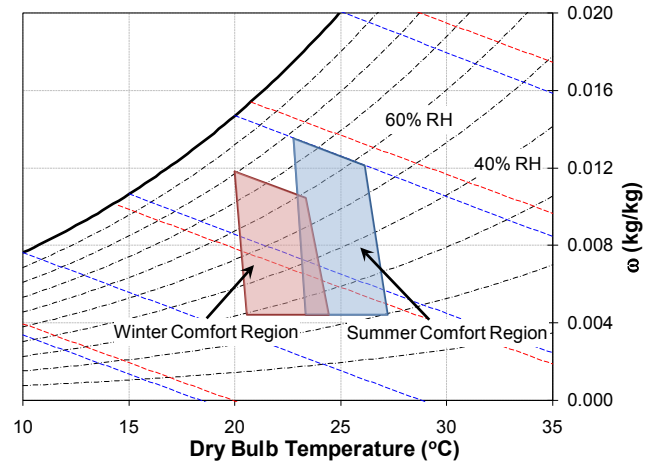
Figure 4: Psychrometric chart with seasonal comfort regions (ASHRAE, 2009)
