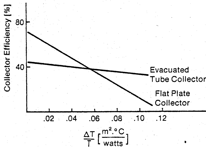
Figure 2-4. Collector Performance Curves.
