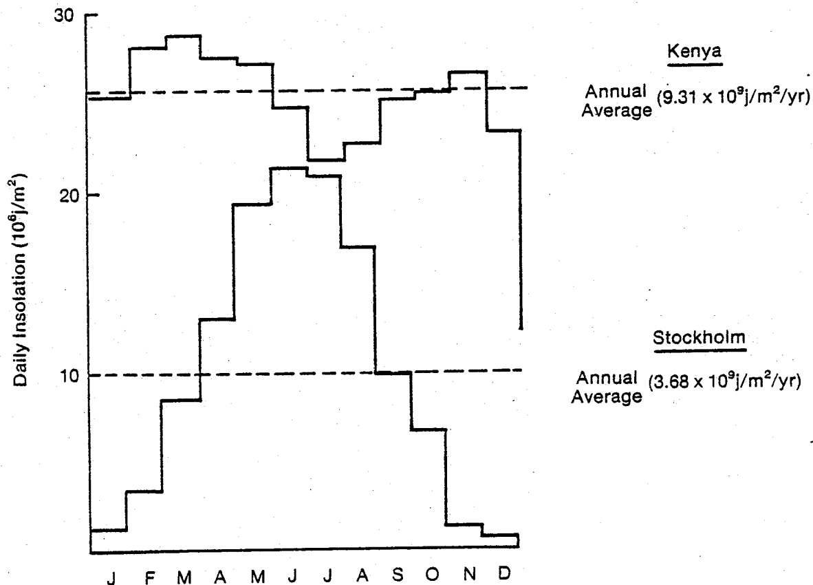
Figure 1-4. Average Daily Horizontal Insolation by Month for Stockholm and Kenya.
