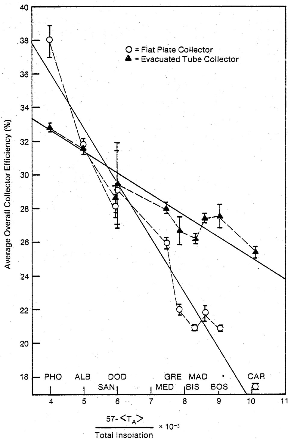
Figure 3-9. Average Overall Collector Efficiency versus \frac{57 - \langle T_A \rangle}{\text{Total Insolation}} (Tilt = Latitude + 10)
