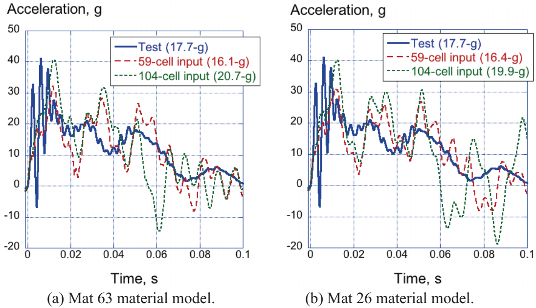
Figure 78. Test-analysis results for sand impact (left center block).
