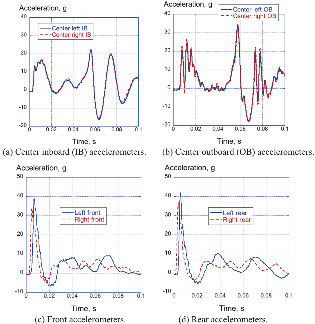
Figure 32. Acceleration time histories from the water impact test.
