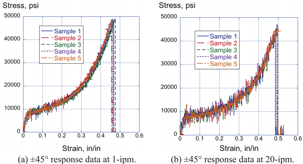
Figure 10. Tensile stress-strain responses of \pm 45^\circ Kevlar®-129 fabric/epoxy coupons tested at two different displacement rates.
