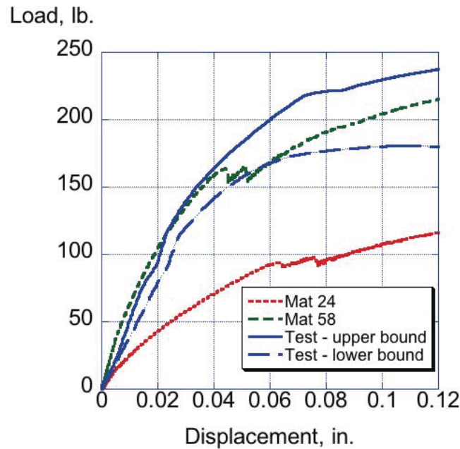
Figure 47. Test/analysis correlation of single cell using Mat 58 and Mat 24 models in LS-DYNA.
