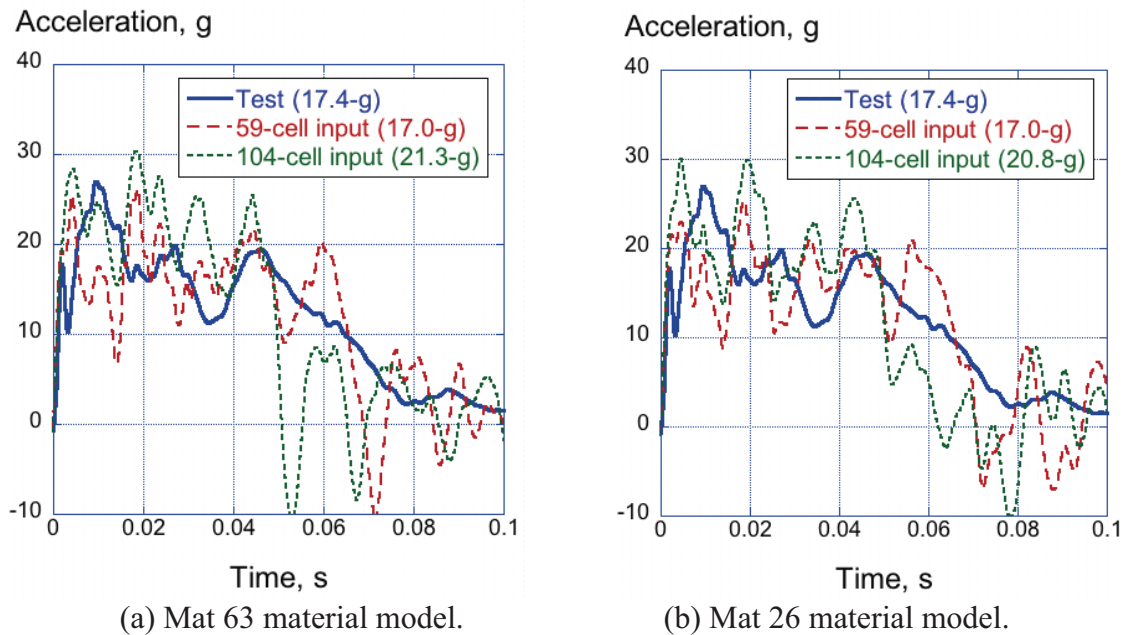
Figure 79. Test-analysis results for sand impact (right center block).
