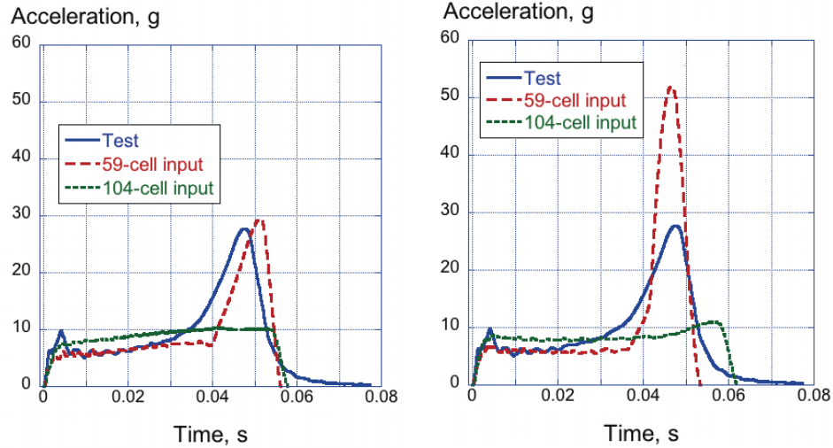
(a) Model executed using Mat 63.
