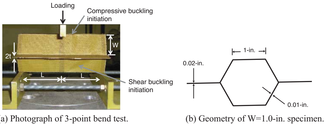
Figure 12. Three-point-bend set-up for single cell tests.
