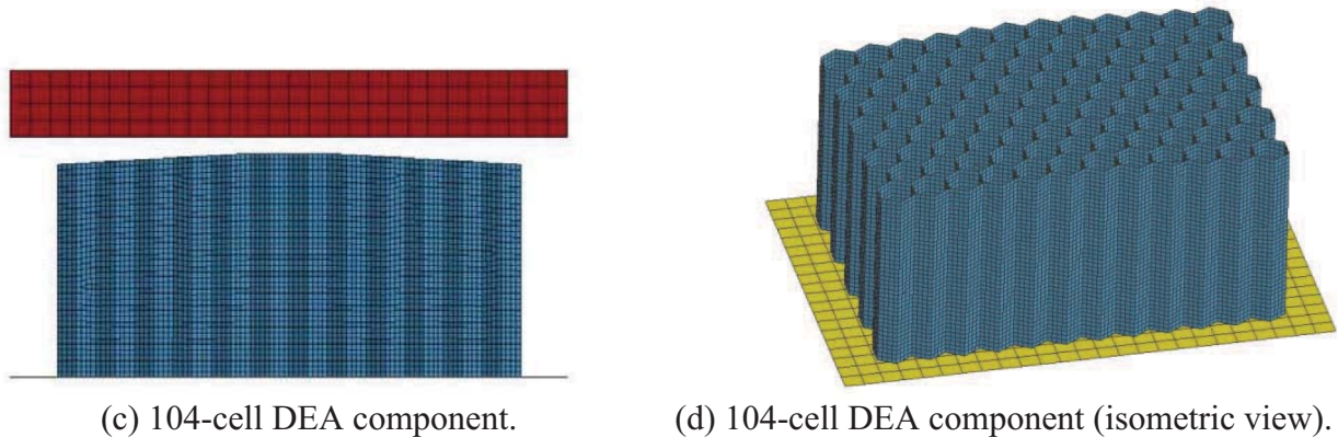
Figure 48. Pictures of the shell element DEA component models.
