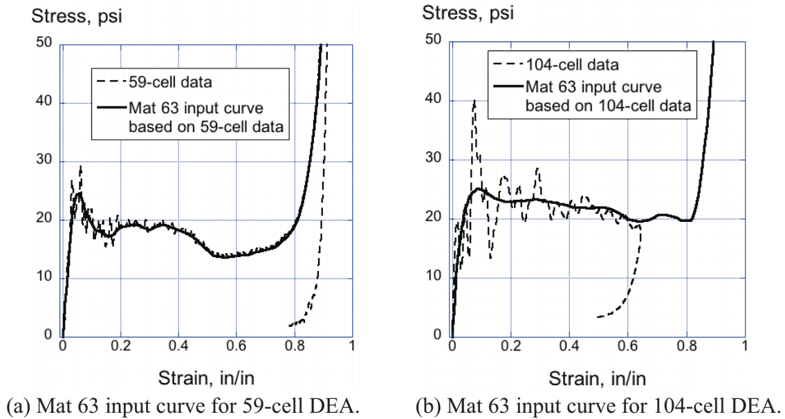
Figure 59. Mat 63 input load curves derived from the 59- and 104-cell DEA test data.
