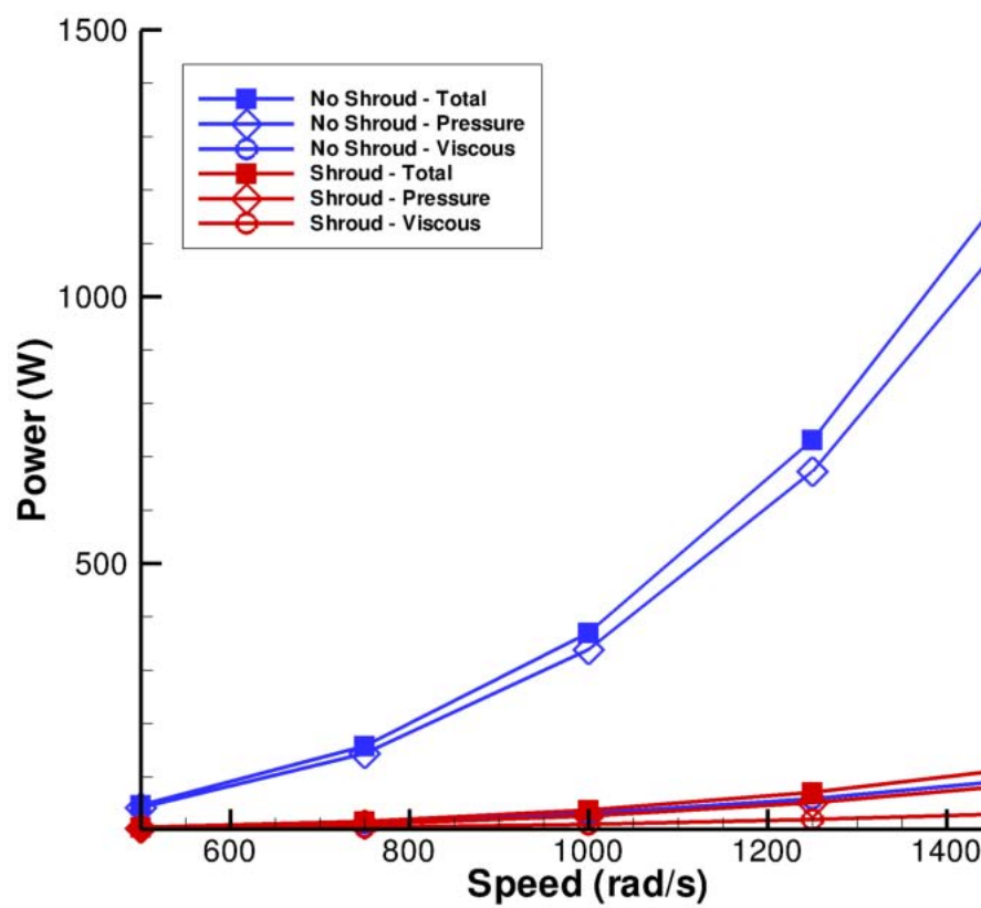
Figure 4.55. Breakdown of pressure and viscous windage power losses for Bell 51-tooth helical gear.
