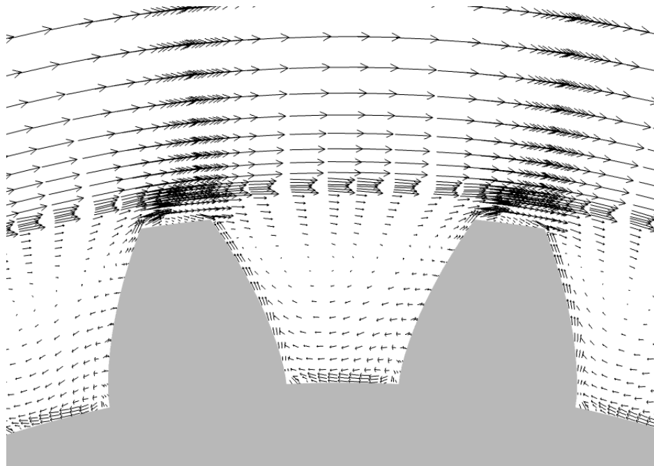
Figure 3.8. Secondary flows within the gear teeth.
