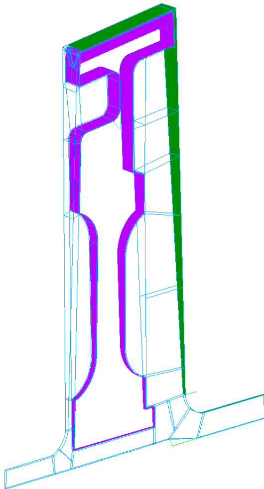
Figure 4.52. Shrouded Bell 139-tooth helical gear grid domain.
