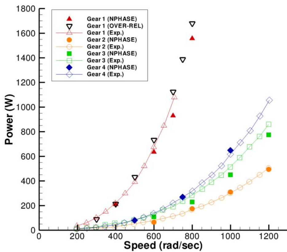
Figure 3.13. Experimental, NPHASE-PSU, and OVER-REL results for Diab Gears 1-4.
