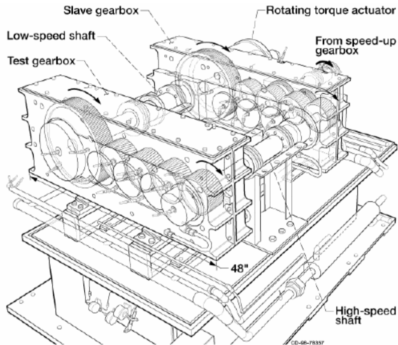
Figure 1.5. NASA High-Speed Helical Gear Train Facility. [5]
