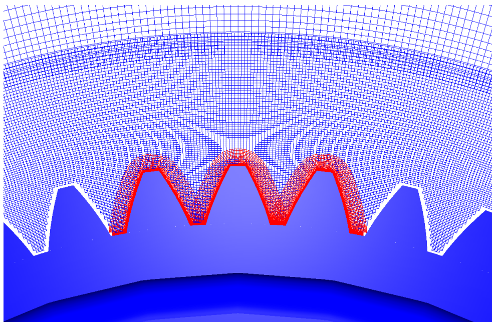
Figure 4.35. Overset mesh topology of the NASA Glenn 13-inch spur gear.
