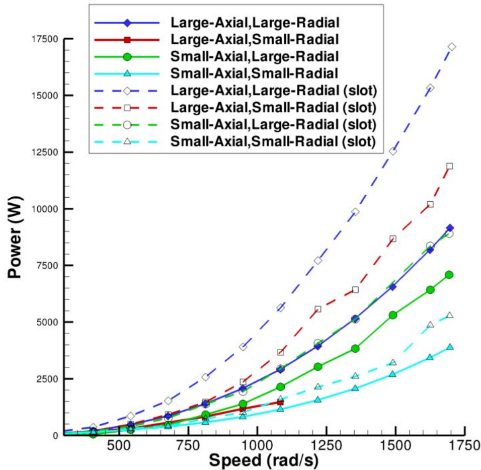
Figure 4.33. NASA experimental gear windage power loss data for 13-inch spur gear for only the shrouded configurations. [7]
