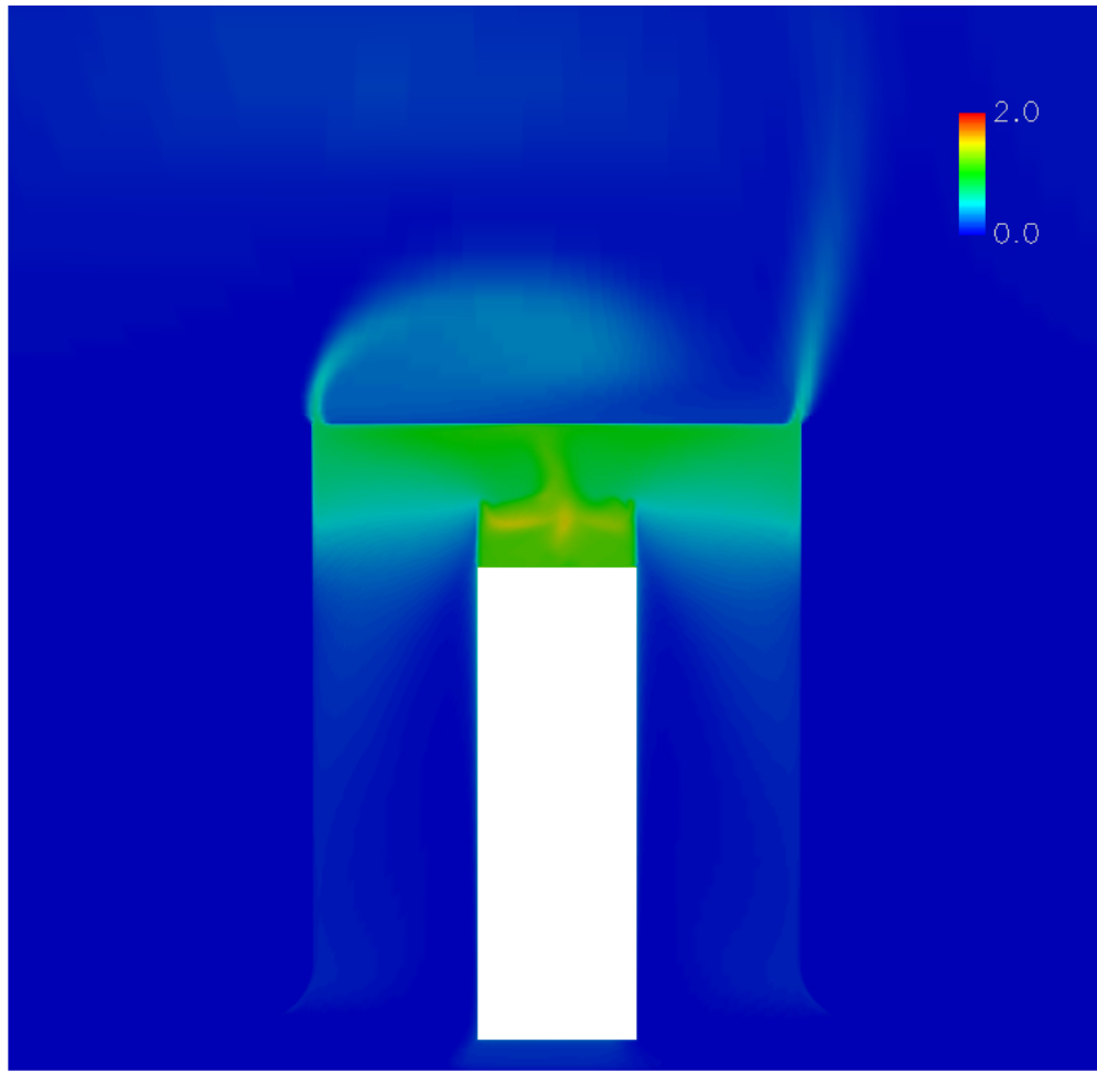
Figure 4.20. Contour plot of tangential velocity for the Large-Axial-Large-Radial shroud with corner slots at 700 rad/s.
