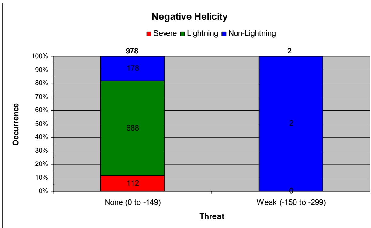
Figure 25. Stacked column graph of negative helicity value thresholds. The numbers of severe days are in red, lightning days without severe weather in green, and non-lightning days in blue. The Melbourne NWS threat criteria are on the x-axis. The cumulative frequency of occurrence of each type of day is shown on the y-axis. The bold numbers at the top of each column indicate the total number of days in that threat range and the numbers within each colored portion of a column indicate the number of days of that type.
