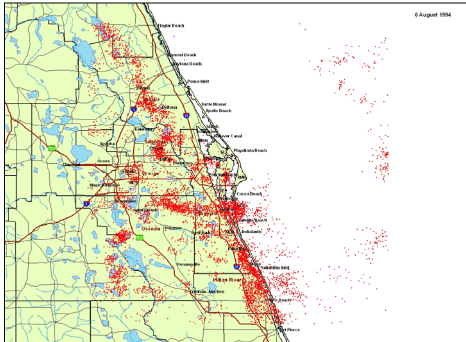
Figure 6. Example of a CGLSS plot from 6 August 1994. Each red dot represents one lightning strike as observed by the CGLSS.
