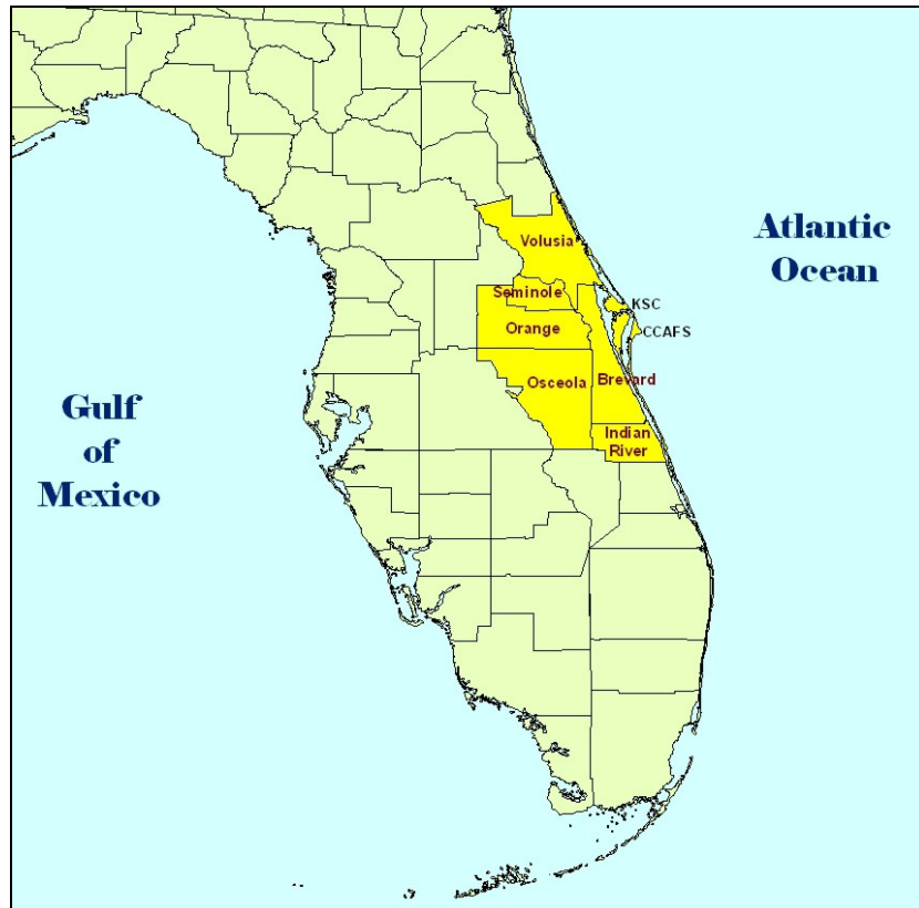
Figure 1. Map of Florida showing the six counties (shaded in yellow) included in the severe weather events database. The location of KSC and CCAFS are shown on the map and both reside in Brevard County.
