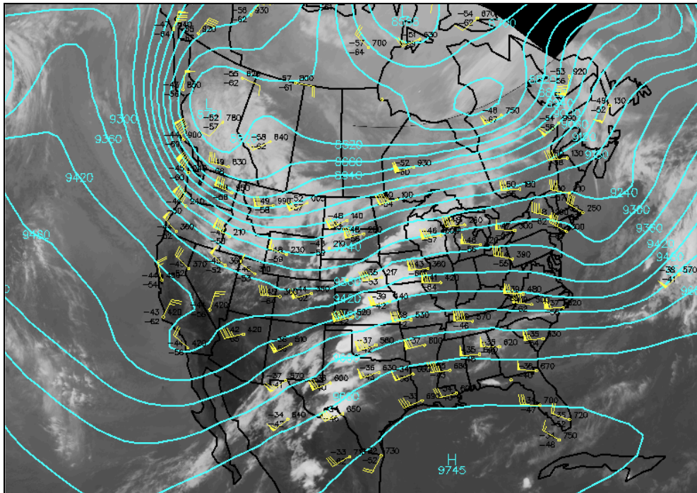
Figure 10. Example of a 300 mb upper air chart used to determine flow aloft over east central Florida.
