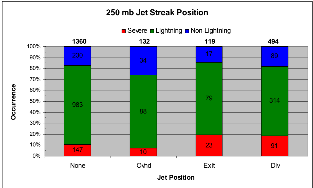
Figure 27. Stacked column graph of 250 mb jet streak position categories. The numbers of severe days are in red, lightning without severe weather days in green, and non-lightning days in blue. The position of the jet streak is on the x-axis. The cumulative frequency of occurrence of each type of day is shown on the y-axis. The bold numbers at the top of each column indicate the total number of days in that threat range and the numbers within each colored portion of a column indicate the number of days of that type.
