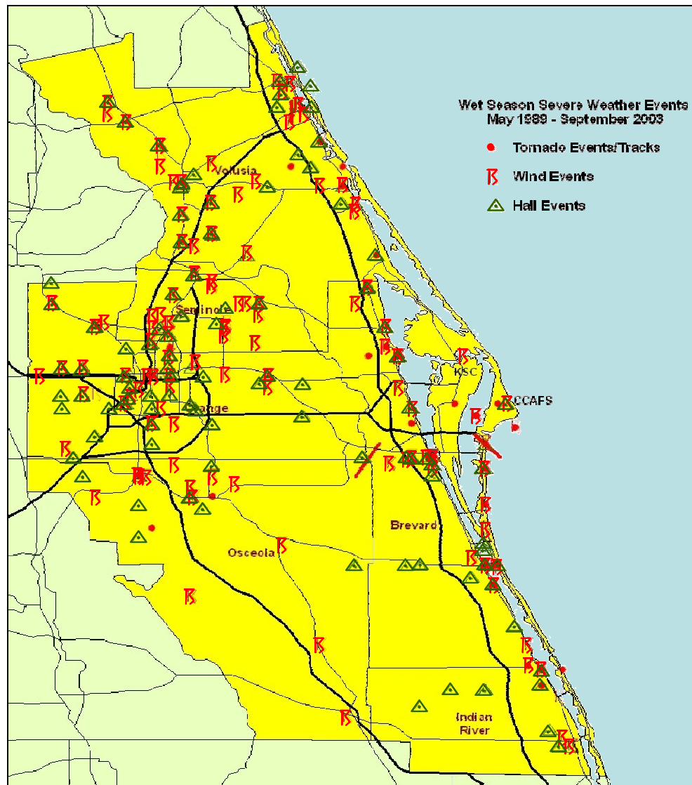
Figure 4. Interstate highways (thick black lines) and major roads (thin black lines) superimposed on the severe weather events map.
