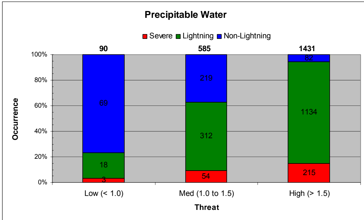
Figure 17. Stacked column graph of PW value thresholds. The numbers of severe days are in red, lightning days without severe weather in green, and non-lightning days in blue. The local forecast rules threat criteria are on the x-axis. The cumulative frequency of occurrence of each type of day is shown on the y-axis. The bold numbers at the top of each column indicate the total number of days in that threat range and the numbers within each colored portion of a column indicate the number of days of that type.
