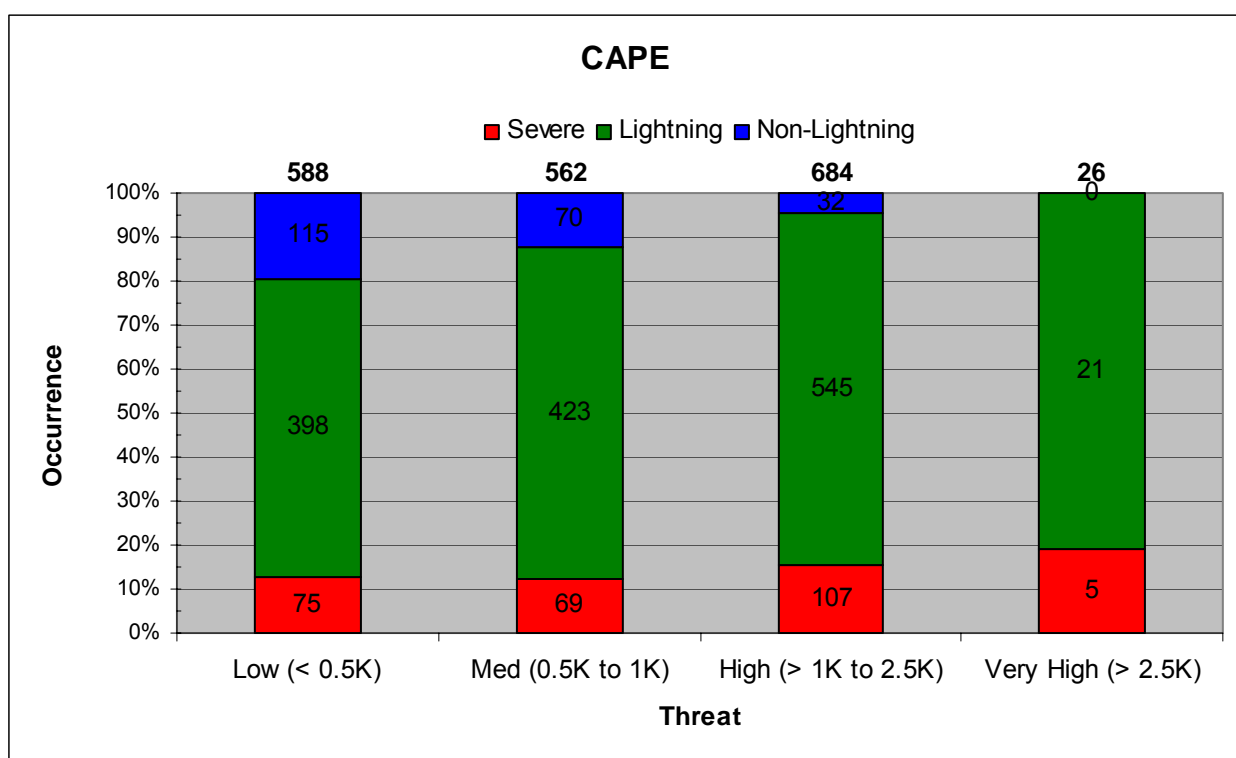
Figure 20. Stacked column graph of CAPE value thresholds. The numbers of severe days are in red, lightning days without severe weather in green, and non-lightning days in blue. The Jacksonville NWS threat criteria are on the x-axis. The cumulative frequency of occurrence of each type of day is shown on the y-axis. The bold numbers at the top of each column indicate the total number of days in that threat range and the numbers within each colored portion of a column indicate the number of days of that type.
