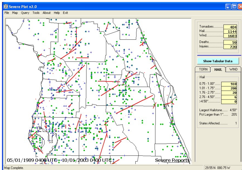
Figure 2. Screen capture from the SPC SeverePlot graphical database program. All reports of tornadoes, hail \geq 0.75 inches and convective surface winds \geq 50 knots from 5/1/89 – 10/1/03 over central Florida are shown. Tornadoes are represented by the red dots, tornado tracks by the red lines, hail by the green dots, and convective wind events by the blue plus signs.
