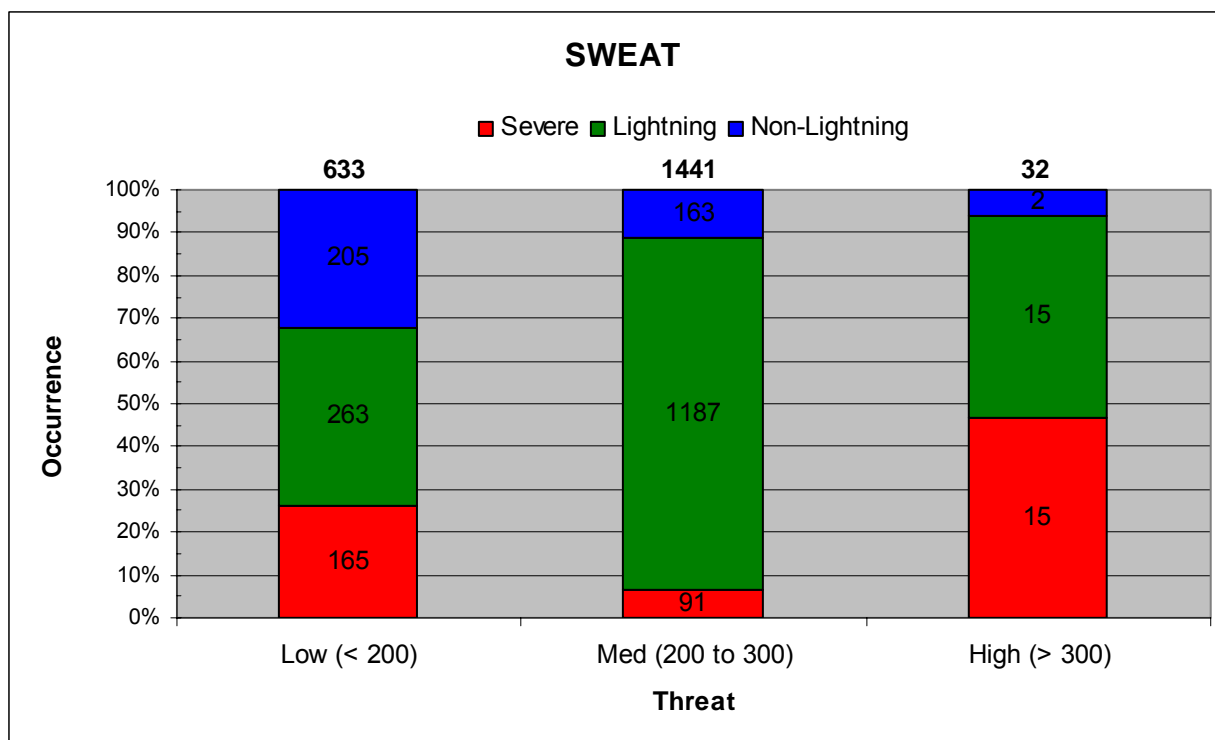
Figure 16. Stacked column graph of SWEAT value thresholds. The numbers of severe days are in red, lightning days without severe weather in green, and non-lightning days in blue. The modified Jacksonville NWS threat criteria are on the x-axis. The cumulative frequency of occurrence of each type of day is shown on the y-axis. The bold numbers at the top of each column indicate the total number of days in that threat range and the numbers within each colored portion of a column indicate the number of days of that type.
