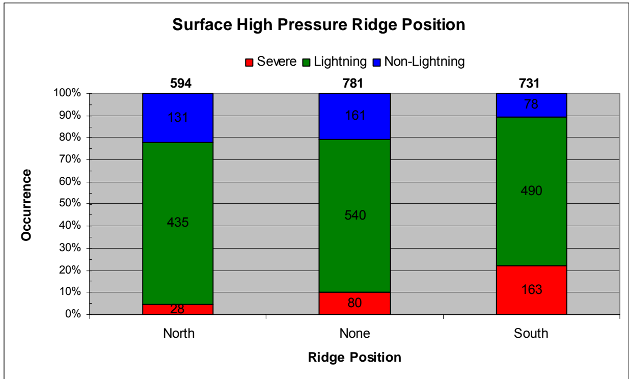
Figure 28. Stacked column graph of surface high pressure ridge position. The numbers of severe days are in red, lightning without severe weather days in green, and non-lightning days in blue. The position of the surface ridge is on the x-axis. The cumulative frequency of occurrence of each type of day is shown on the y-axis. The bold numbers at the top of each column indicate the total number of days in that threat range and the numbers within each colored portion of a column indicate the number of days of that type.
