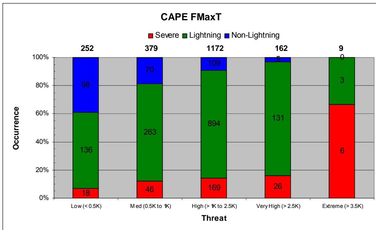
Figure 22. Stacked column graph of CAPE FMaxT value thresholds. The numbers of severe days are in red, lightning days without severe weather in green, and non-lightning days in blue. The Jacksonville NWS threat criteria are on the x-axis. The cumulative frequency of occurrence of each type of day is shown on the y-axis. The bold numbers at the top of each column indicate the total number of days in that threat range and the numbers within each colored portion of a column indicate the number of days of that type.
