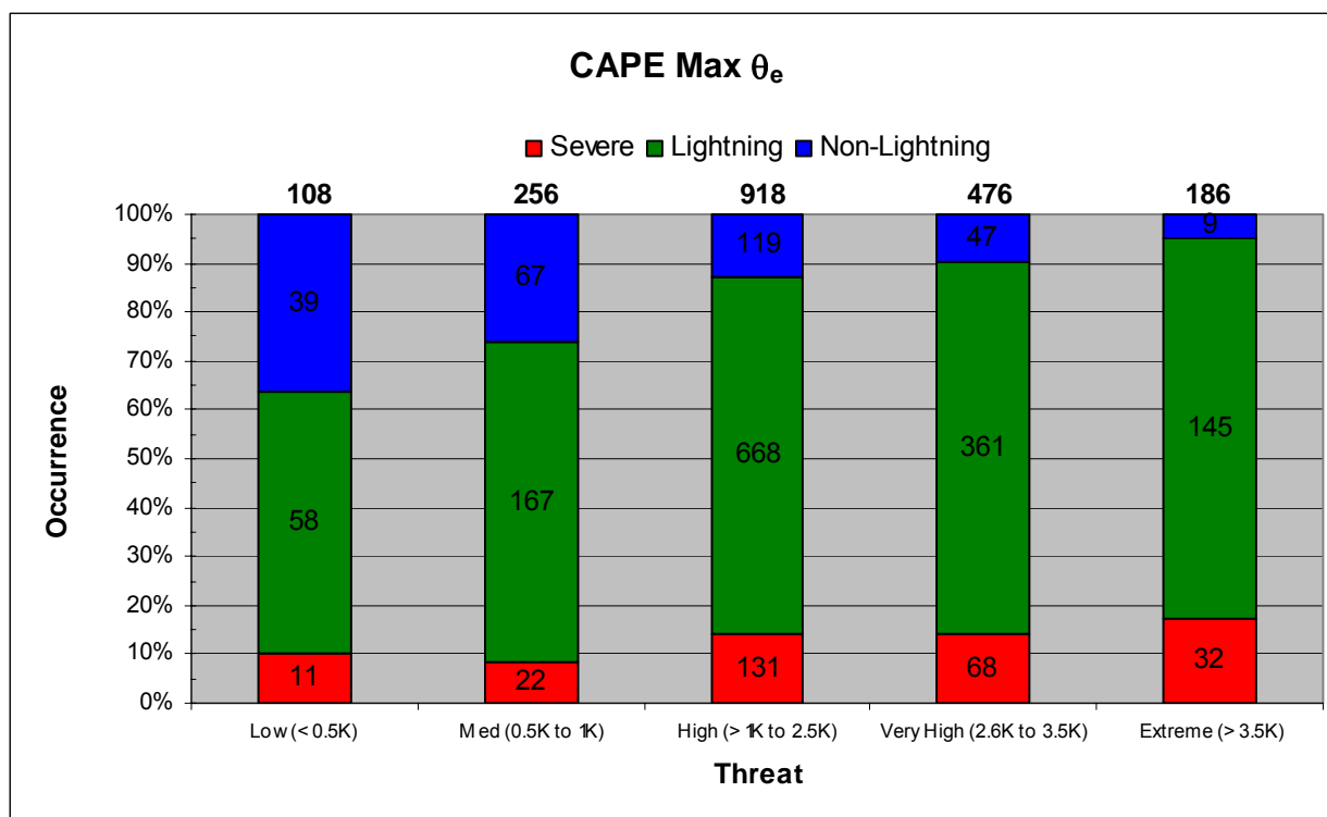
Figure 21. Stacked column graph of CAPE Max \theta_e value thresholds. The numbers of severe days are in red, lightning days without severe weather in green, and non-lightning days in blue. The Jacksonville NWS threat criteria are on the x-axis. The cumulative frequency of occurrence of each type of day is shown on the y-axis. The bold numbers at the top of each column indicate the total number of days in that threat range and the numbers within each colored portion of a column indicate the number of days of that type.
