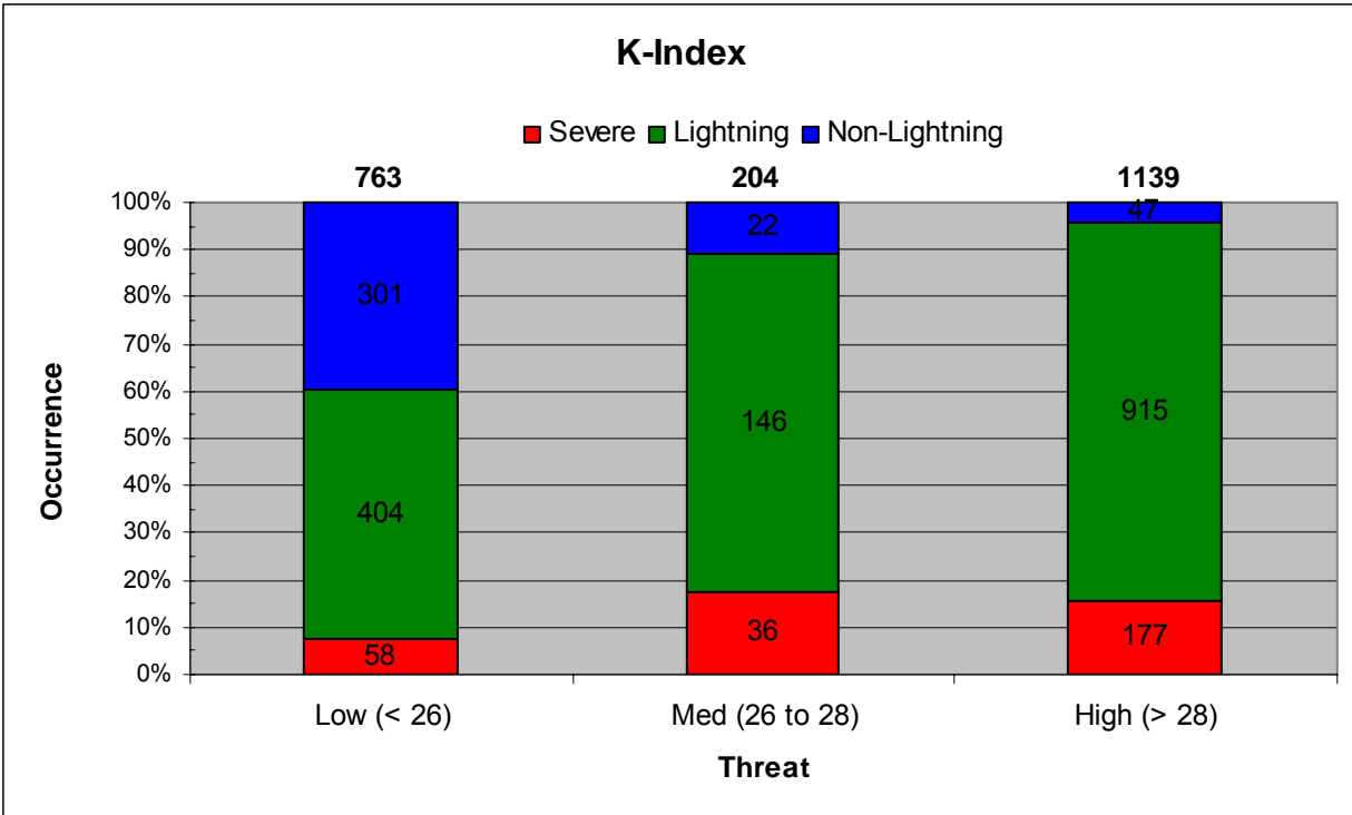
Figure 13. Stacked column graph of KI value thresholds. The numbers of severe days are in red, lightning days without severe weather in green, and non-lightning days in blue. The 45 WS threat criteria and thresholds are on the x-axis. The cumulative frequency of occurrence of each type of day is shown on the y-axis. The bold numbers at the top of each column indicate the total number of days in that threat range and the numbers within each colored portion of a column indicate the number of days of that type.
