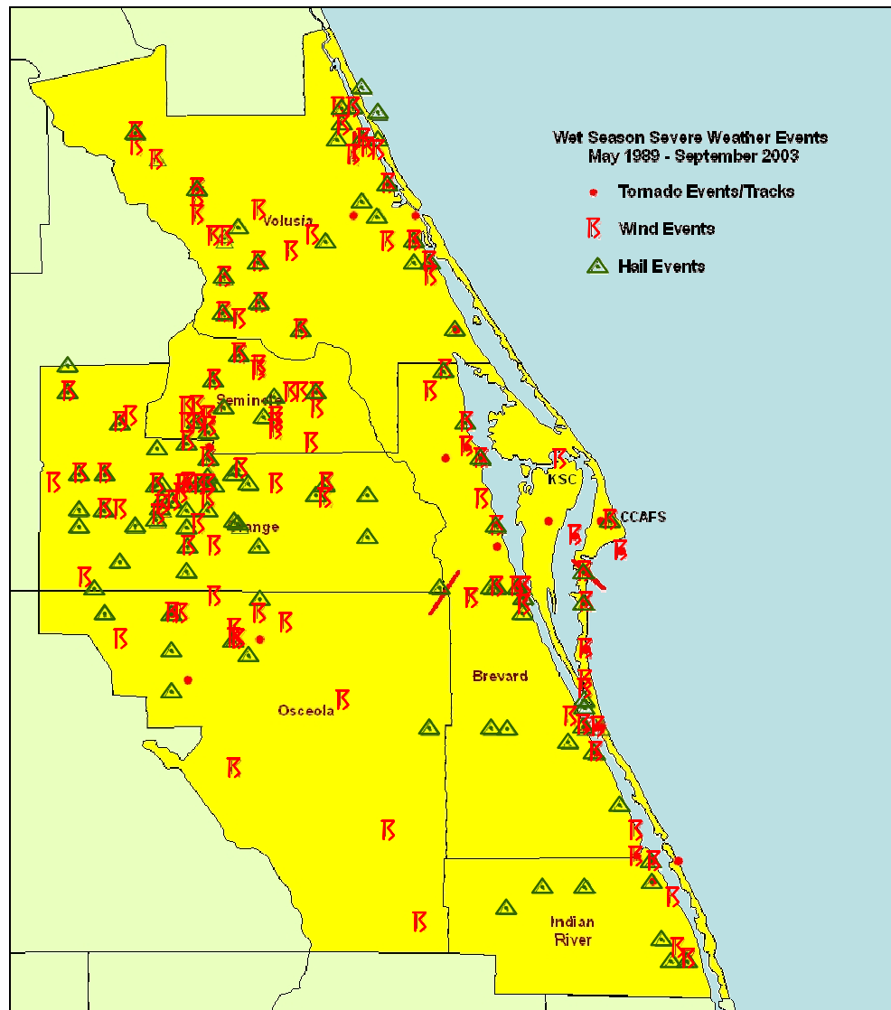
Figure 3. Locations of all tornado, wind, and hail events in the database used for this task. Tornadoes are represented by the red dots, tornado tracks by the red lines, hail by the green triangles, and wind events by the red severe thunderstorm symbols.
