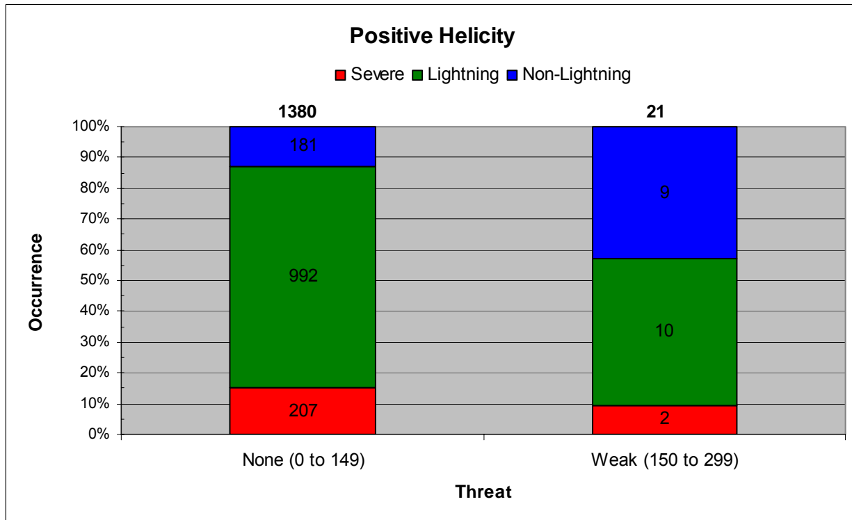
Figure 24. Stacked column graph of positive helicity value thresholds. The numbers of severe days are in red, lightning days without severe weather in green, and non-lightning days in blue. The Melbourne NWS threat criteria are on the x-axis. The cumulative frequency of occurrence of each type of day is shown on the y-axis. The bold numbers at the top of each column indicate the total number of days in that threat range and the numbers within each colored portion of a column indicate the number of days of that type.
