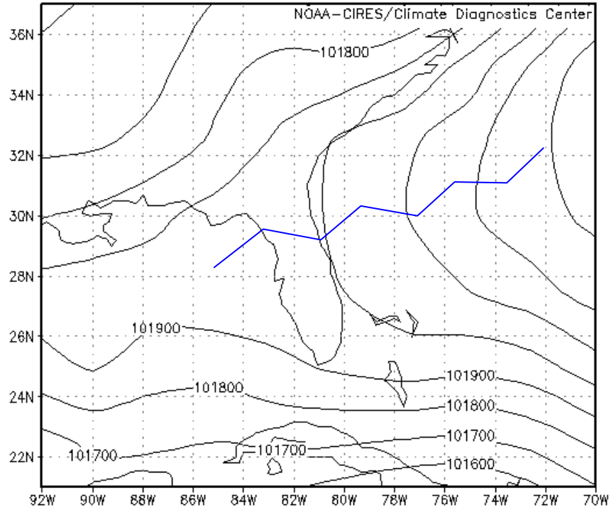
Figure 11. Example of a surface map used to determine the position of the surface ridge over east central Florida. The high pressure ridge axis is highlighted by the jagged blue line.
