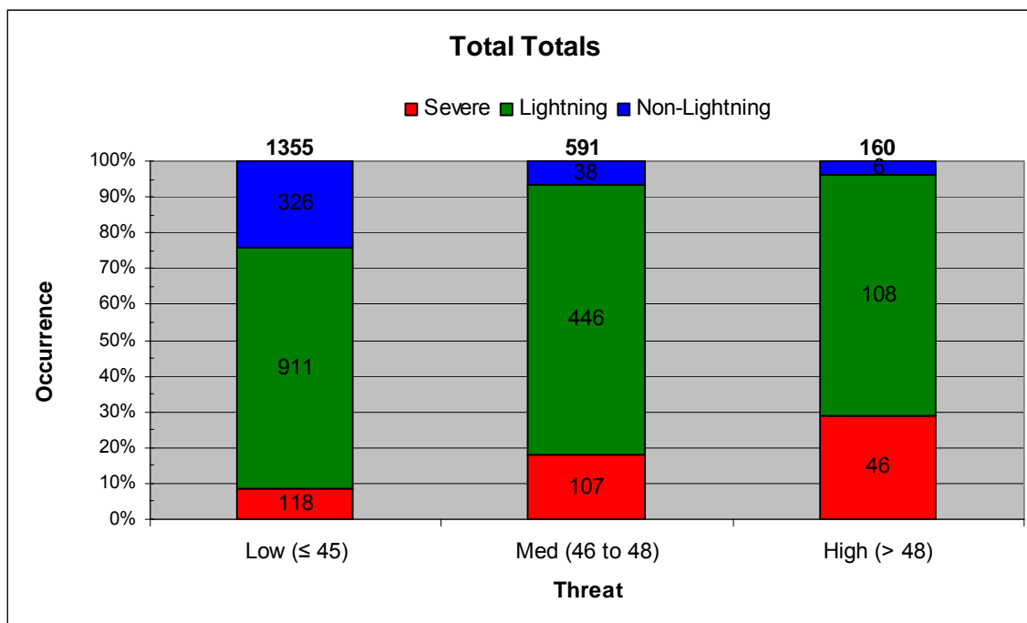
Figure 12. Stacked column graph of TT value thresholds. The numbers of severe days are in red, lightning days without severe weather in green, and non-lightning days in blue. The 45 WS threat criteria and thresholds are on the x-axis. The cumulative frequency of occurrence of each type of day is shown on the y-axis. The bold numbers at the top of each column indicate the total number of days in that threat range and the numbers within each colored portion of a column indicate the number of days of that type.
