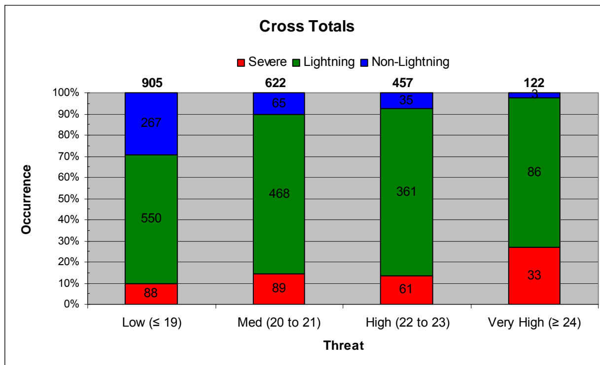
Figure 19. Stacked column graph of CT value thresholds. The numbers of severe days are in red, lightning days without severe weather in green, and non-lightning days in blue. The threat criteria are based on a modified version of the NWS SRH online glossary (NWS SRH 2005) and are on the x-axis. The cumulative frequency of occurrence of each type of day is shown on the y-axis. The bold numbers at the top of each column indicate the total number of days in that threat range and the numbers within each colored portion of a column indicate the number of days of that type.
