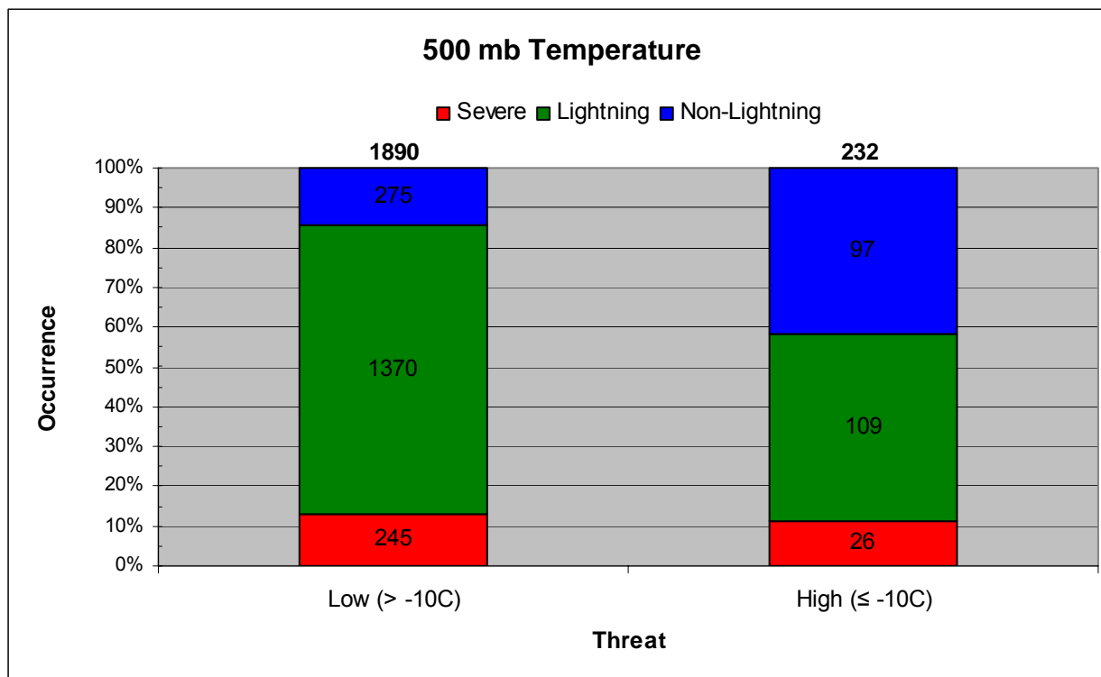
Figure 23. Stacked column graph of T_{500} value thresholds. The numbers of severe days are in red, lightning days without severe weather in green, and non-lightning days in blue. The 45 WS threat criteria are on the x-axis. The cumulative frequency of occurrence of each type of day is shown on the y-axis. The bold numbers at the top of each column indicate the total number of days in that threat range and the numbers within each colored portion of a column indicate the number of days of that type.
