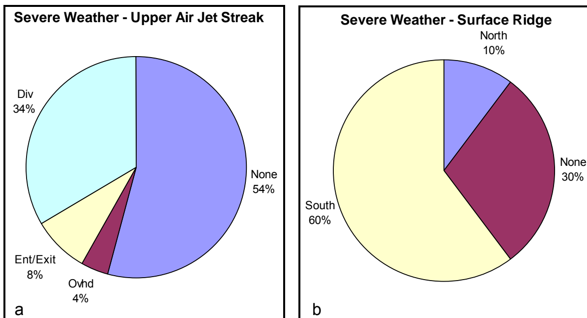
Figure 26. Pie charts showing the relationship between severe days and (a) the upper level jet streak position and (b) surface ridge position.
