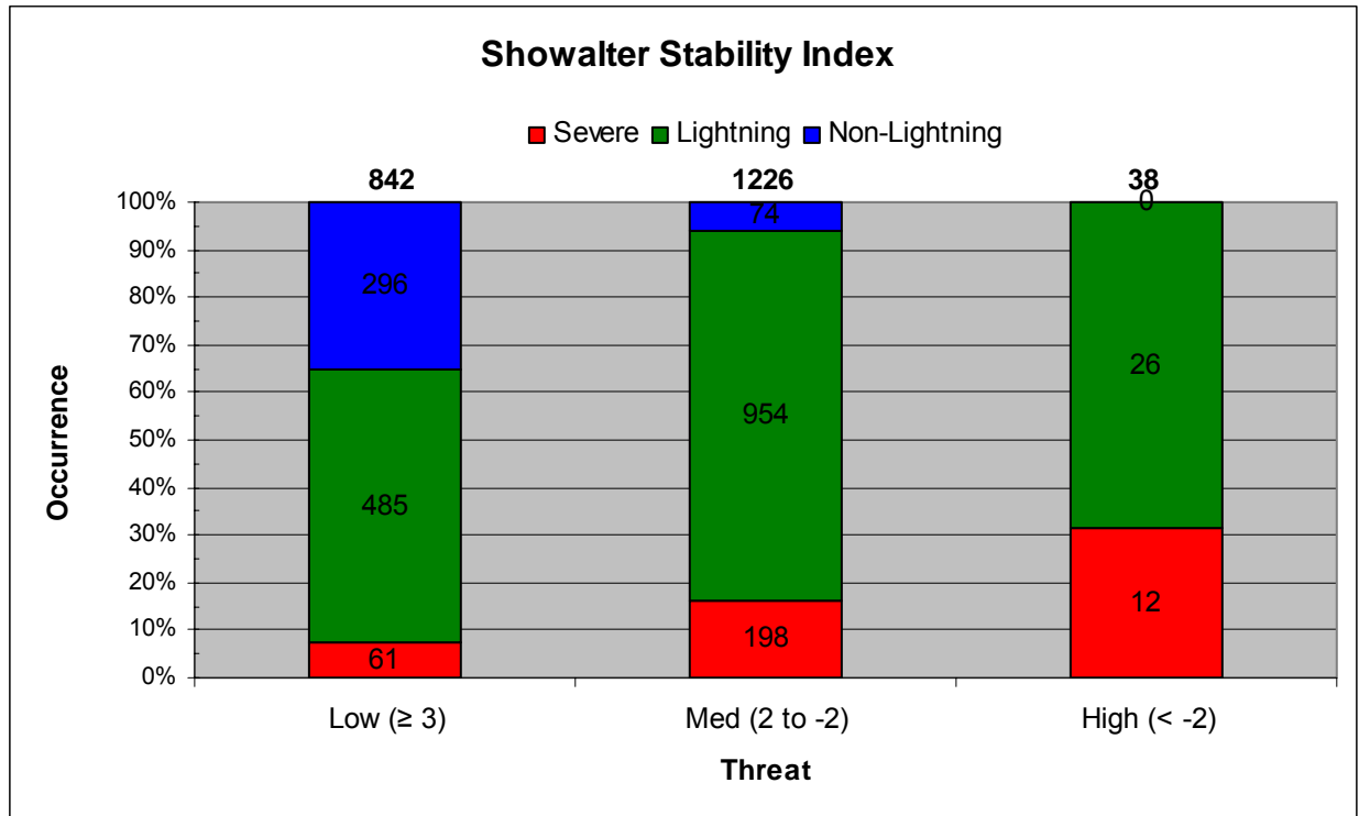
Figure 18. Stacked column graph of SSI value thresholds. The numbers of severe days are in red, lightning days without severe weather in green, and non-lightning days in blue. The 45 WS threat criteria are on the x-axis. The cumulative frequency of occurrence of each type of day is shown on the y-axis. The bold numbers at the top of each column indicate the total number of days in that threat range and the numbers within each colored portion of a column indicate the number of days of that type.
