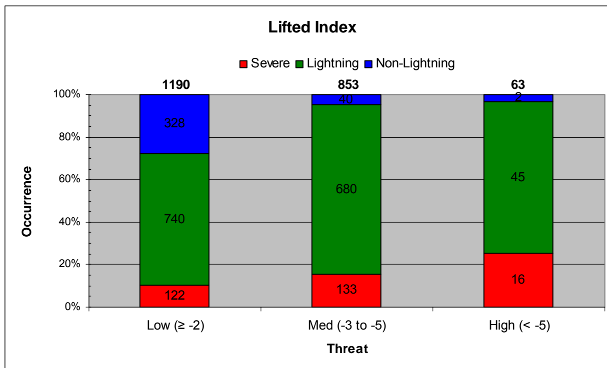
Figure 14. Stacked column graph of LI value thresholds. The numbers of severe days are in red, lightning days without severe weather in green, and non-lightning days in blue. The 45 WS threat criteria and thresholds are on the x-axis. The cumulative frequency of occurrence of each type of day is shown on the y-axis. The bold numbers at the top of each column indicate the total number of days in that threat range and the numbers within each colored portion of a column indicate the number of days of that type.
