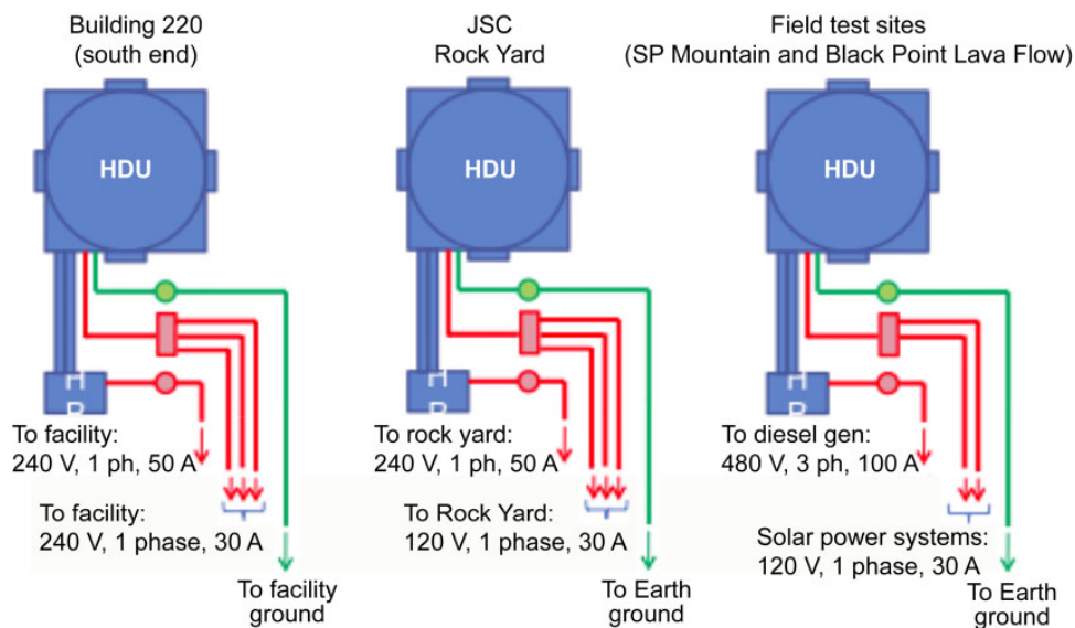
Figure 13.—HDU power sources for different operational locations.
