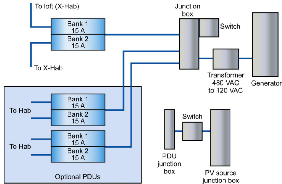
Figure 30.—Additional power conditioning components to support the X-Hab.
