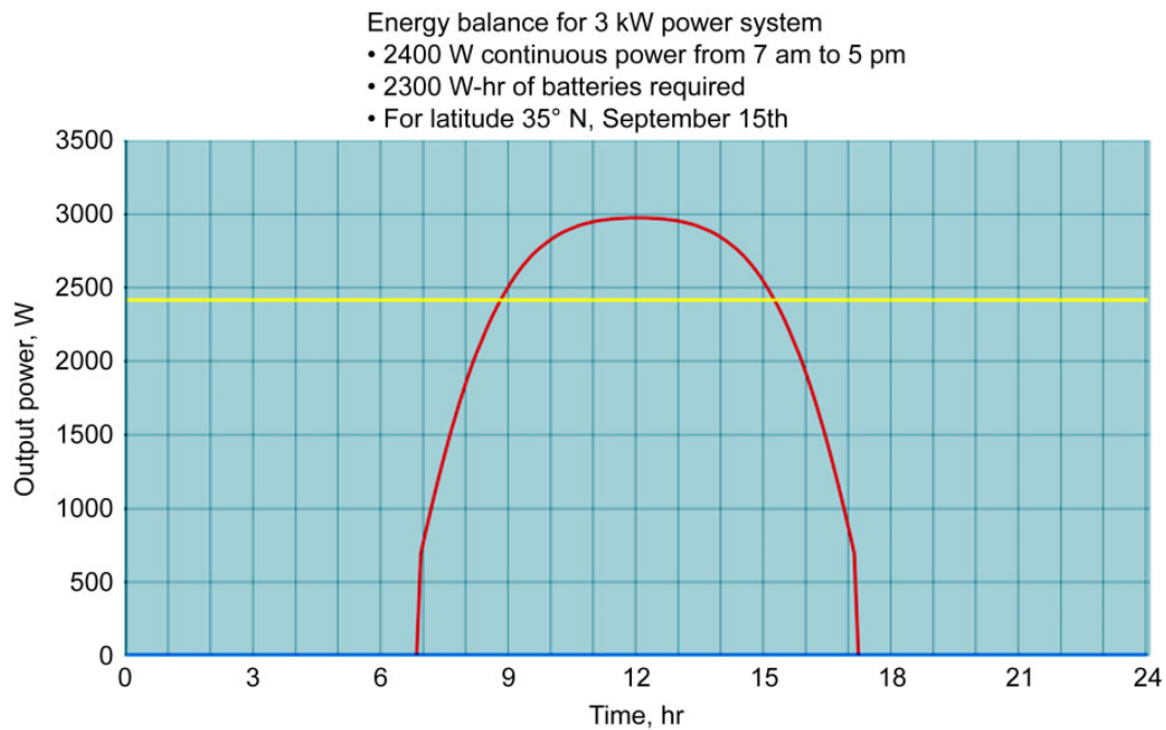
Figure 34.—Energy balance output for the 3 kW mobile power system.
