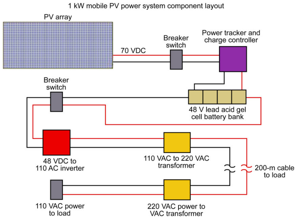
Figure 24.—Operational layout for the 1 kW mobile power system.
