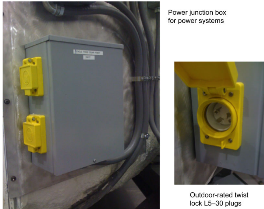
Figure 19.—Photovoltaic (PV) power systems junction box and plugs.
