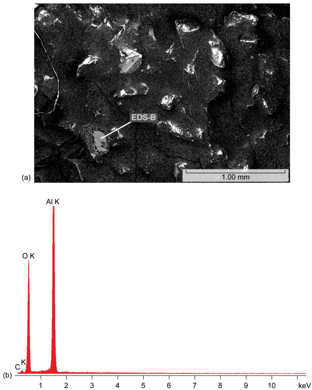
Figure 10.—(a) SEM photomicrograph of surface of flap wheel abrasive paper showing abrasive particles partially exposed and (b) the EDS spectrum of one such particle as indicated in the figure.
