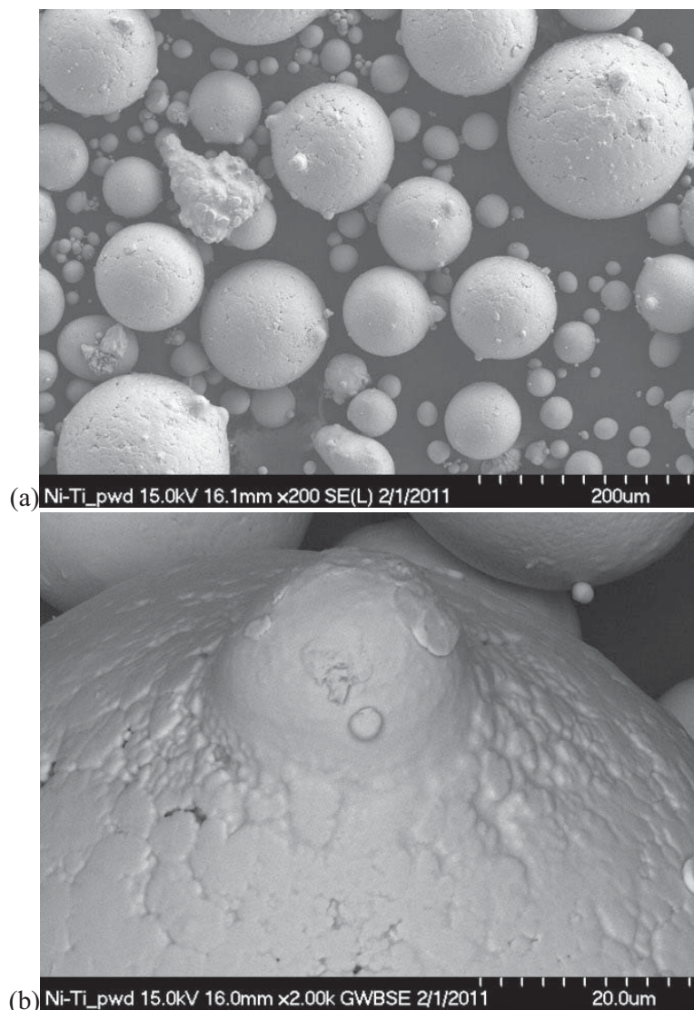
Figure 3.—Scanning electron photomicrograph of the 60-NITINOL powder characterized in Table I shown at (a) 200X original magnification and (b) 2,000X original magnification.
