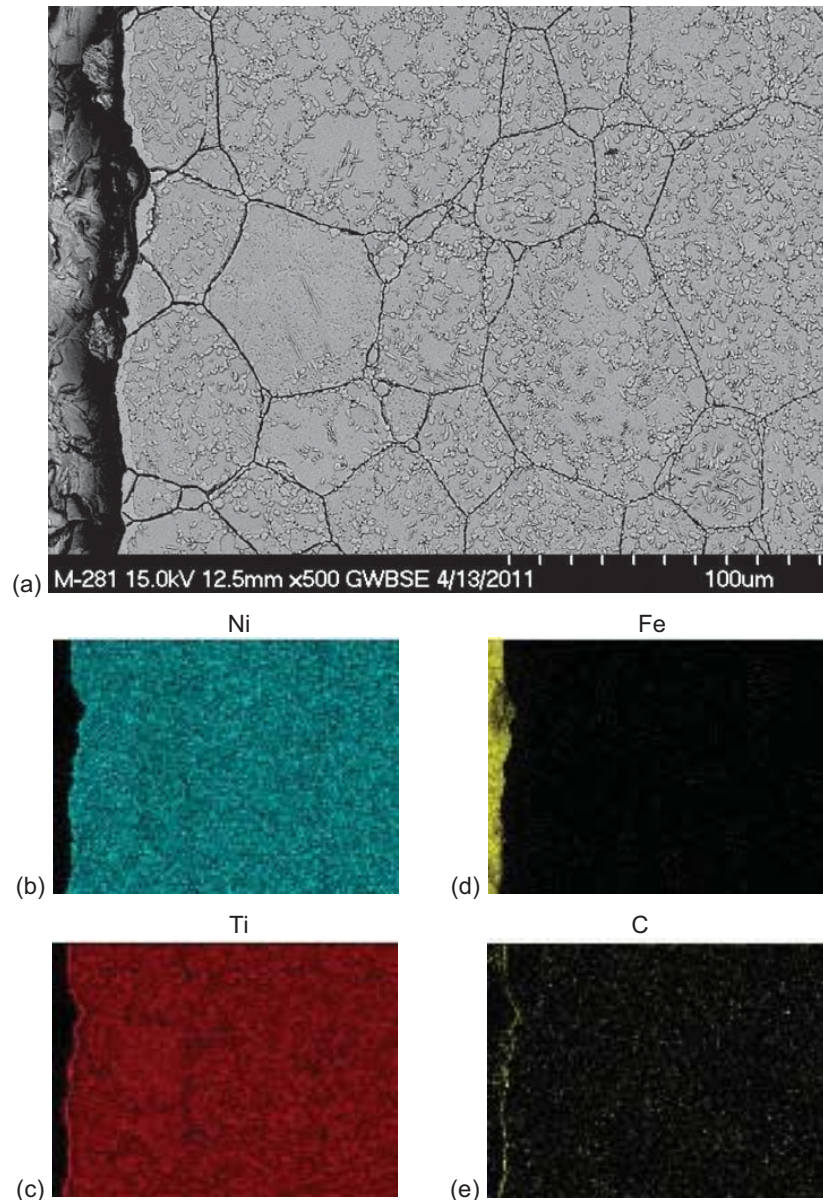
Figure 6.—(a) SEM photomicrograph of the 60-NITINOL compact near the stainless steel container (seen on the left of image) and (b) to (e) x-ray elemental dot maps from this image showing the major elements present.
