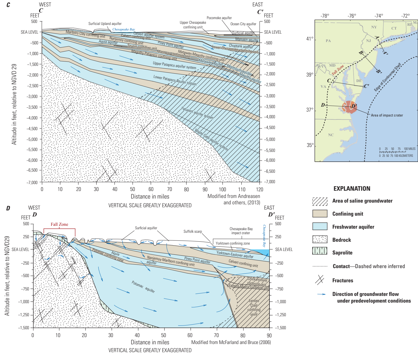
Figure 10. Cross-sections A, A–A' on Long Island, New York, B, B–B' in New Jersey, C, C–C' in Delaware and Maryland, and D, D–D' in Virginia, showing the regional variations in the hydrogeologic framework of the Northern Atlantic Coastal Plain aquifer system. Cross-section D–D' includes the impact crater in the Chesapeake Bay.
