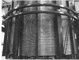
An 800-meter sample toroidal field conductor was delivered to the EU in June 2014. Photo: U.S. ITER
