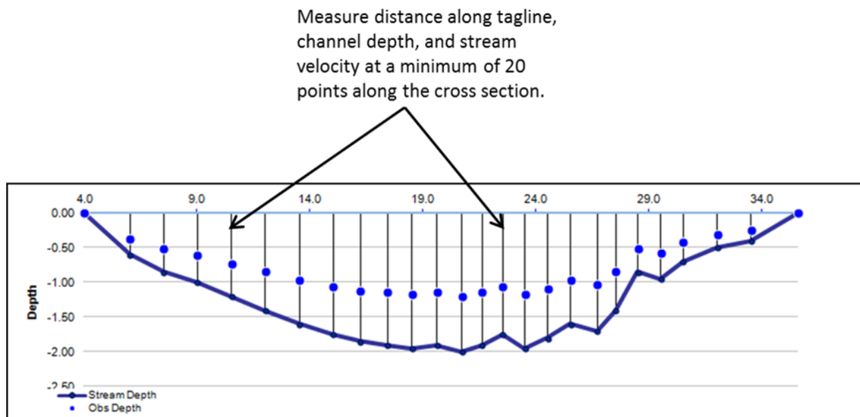
Figure 35. Layout of a channel cross-section for obtaining discharge data, using the velocity-area procedure.
