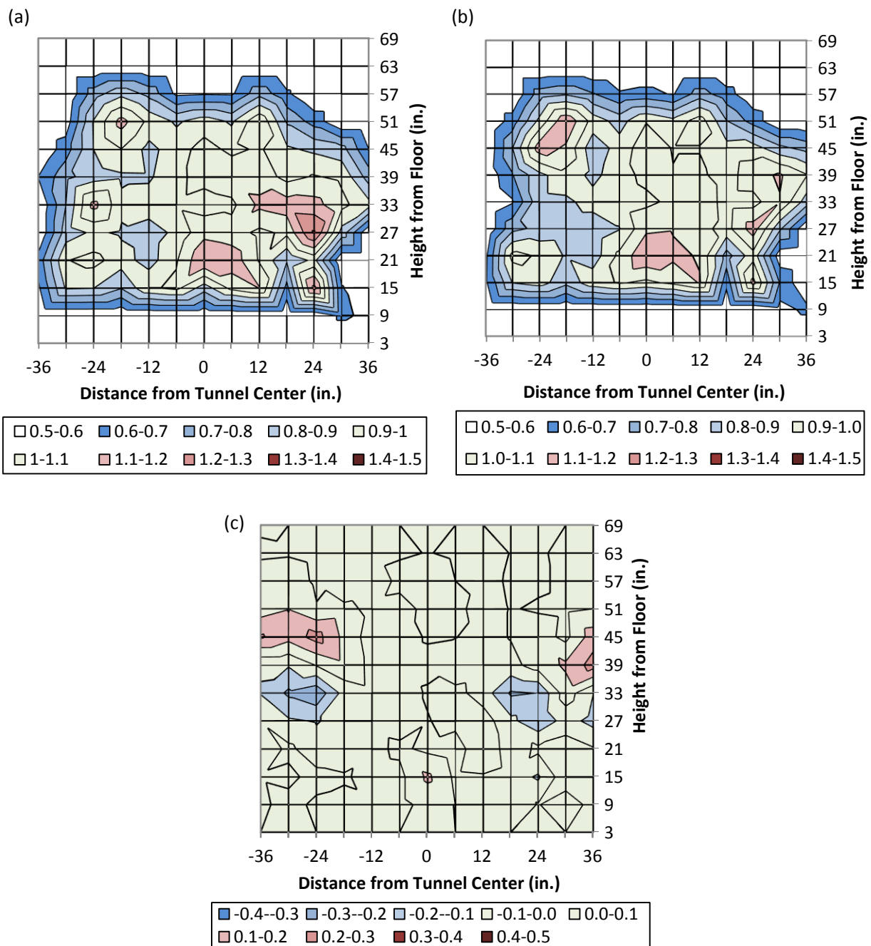
Figure 6.—LWC uniformity contour plot for a large-drop case, V = 150 kn, MVD = 100 \mu m, Pair = 3 psig, plotted as a ratio of the average thickness of the central 12 elements. (a) Ice thickness measured Feb. 2014. (b) Ice thickness measured Jan. 2015. (c) Differences between Figure 6(a) and Figure 6(b) (as a ratio of the central 12 elements in Figure 6(a)). Note that this plot has a different scale than the prior difference plots.
