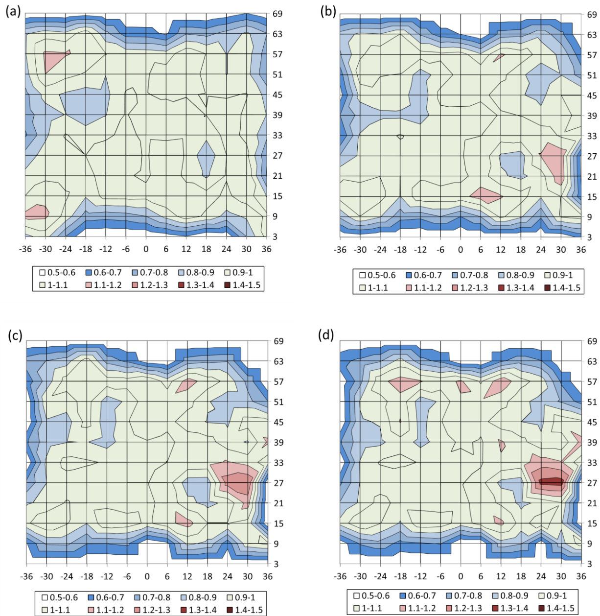
Figure 4.—Mod1 nozzle LWC uniformity plots measured in February 2014 at several airspeeds, MVD = 20 \mu\text{m} , Pair = 20 psig, V = (a) 100 kn, (b) 150 kn, (c) 200 kn, and (d) 250 kn. (Axes same as Figure 3). The values are plotted as a ratio of the average thickness of the central 12 elements.
