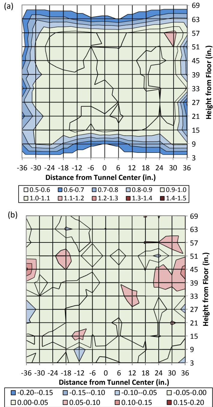
Figure 3.—Standard nozzle LWC uniformity for MVD = 20 \mu\text{m} , Pair = 20 psig, V = 150 kn, measured Jan. 2015. Note the two plots have different scales. (a) Ice thickness, plotted as a ratio of the average thickness of the central 12 elements. (b) Differences between Figure 3(a) (Jan. 2015) and Figure 3 of Ref. 2 (Feb. 2014), normalized by the average thickness of the central 12 elements from the Feb. 2014 measurement.
