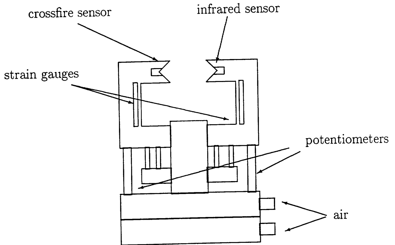
Figure 2.1: CIRSE Gripper
