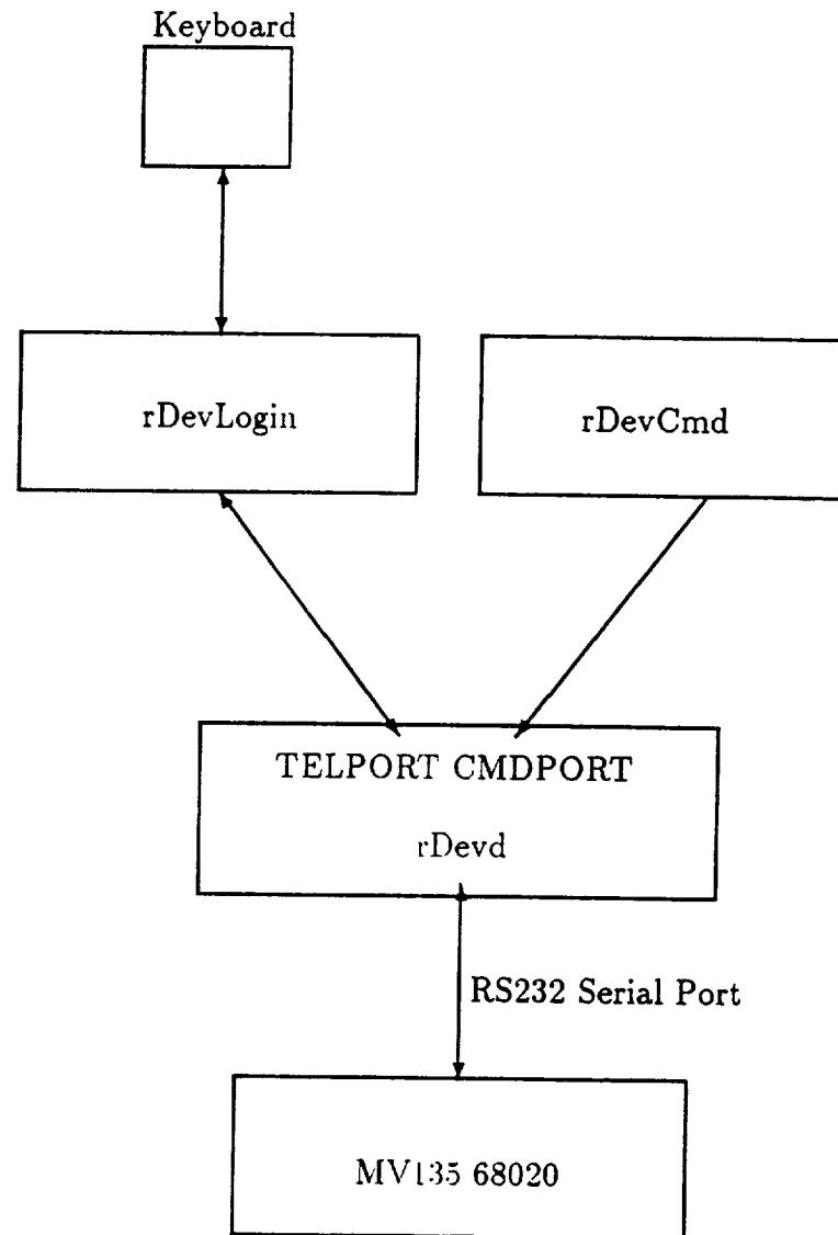
Figure 6.1: Network Connections
