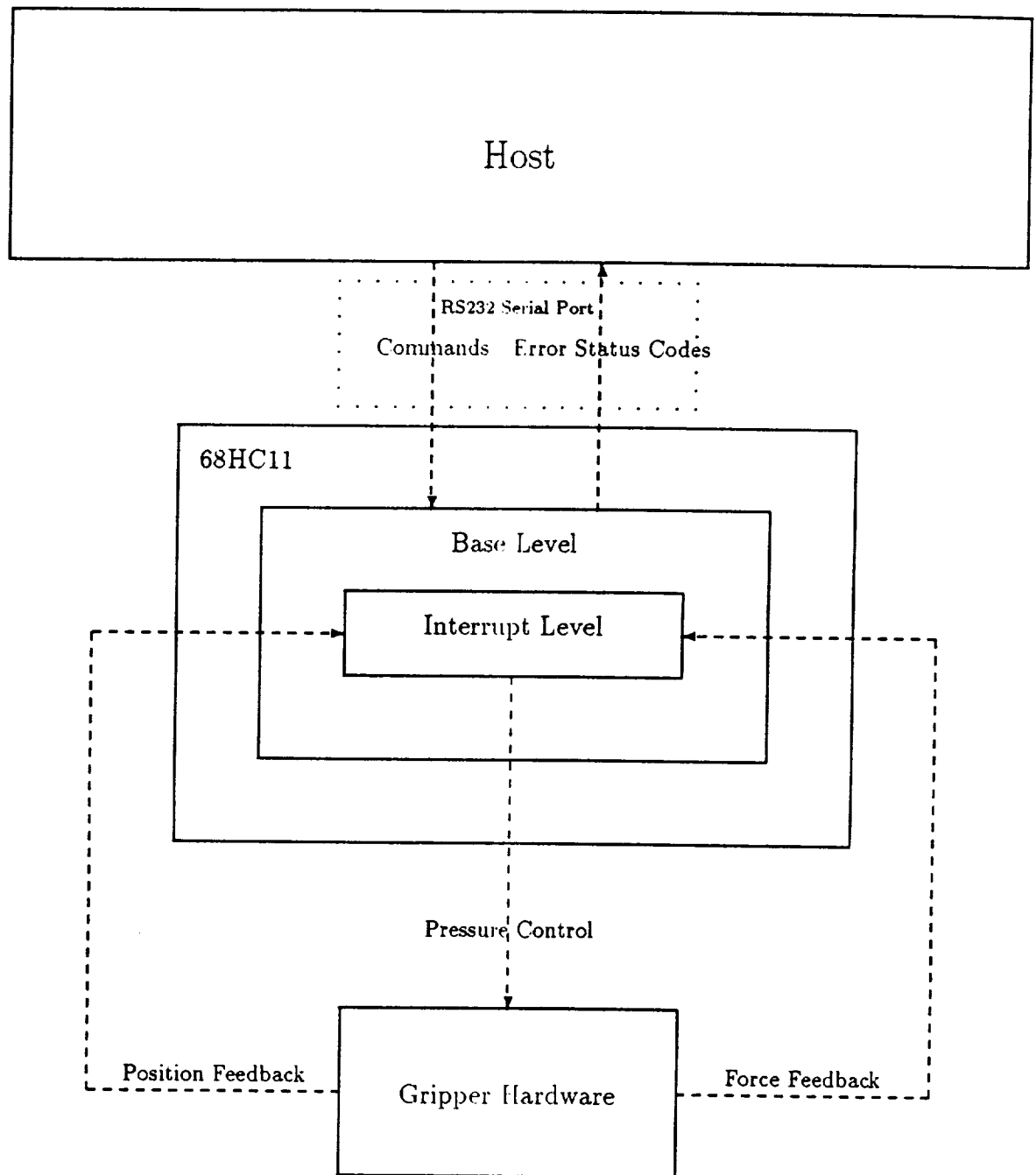
Figure 4.1: Software Architecture
