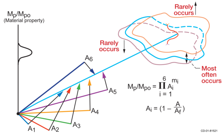
Figure 2.—Multifactor interaction model with substructuring.
