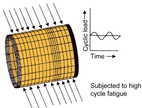
Figure 10.—Finite element model of engine hot section ceramic-matrix-composite component.
