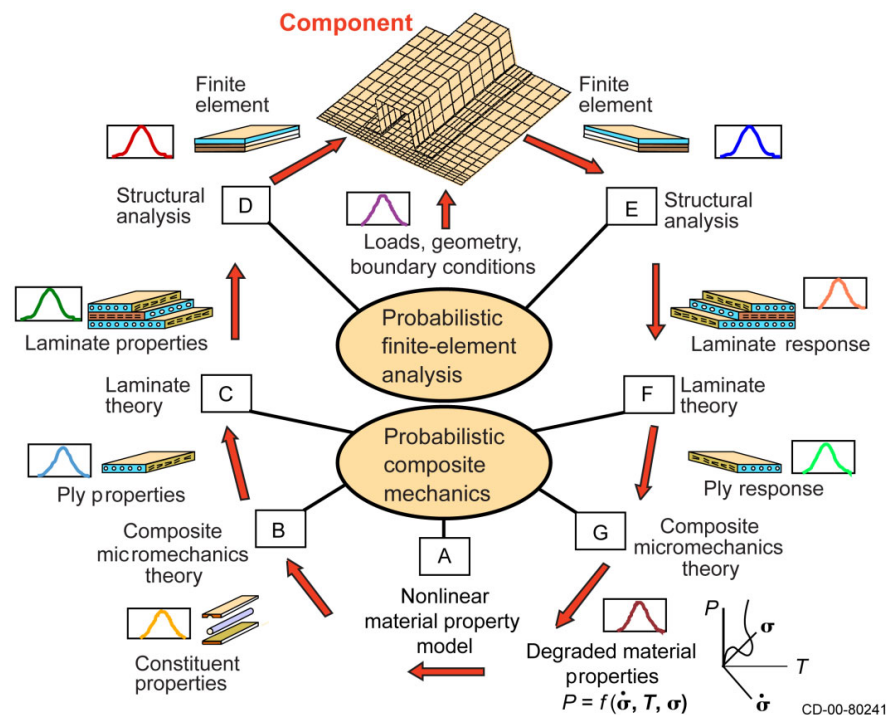
Figure 7.—Probabilistic assessment of composite structures computational simulation cycle.
