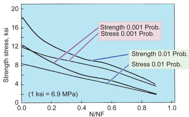
Figure 11.—Probabilistic evaluations of local strength and stress evolution in engine hot section components subjected to high cycle fatigue environment.
