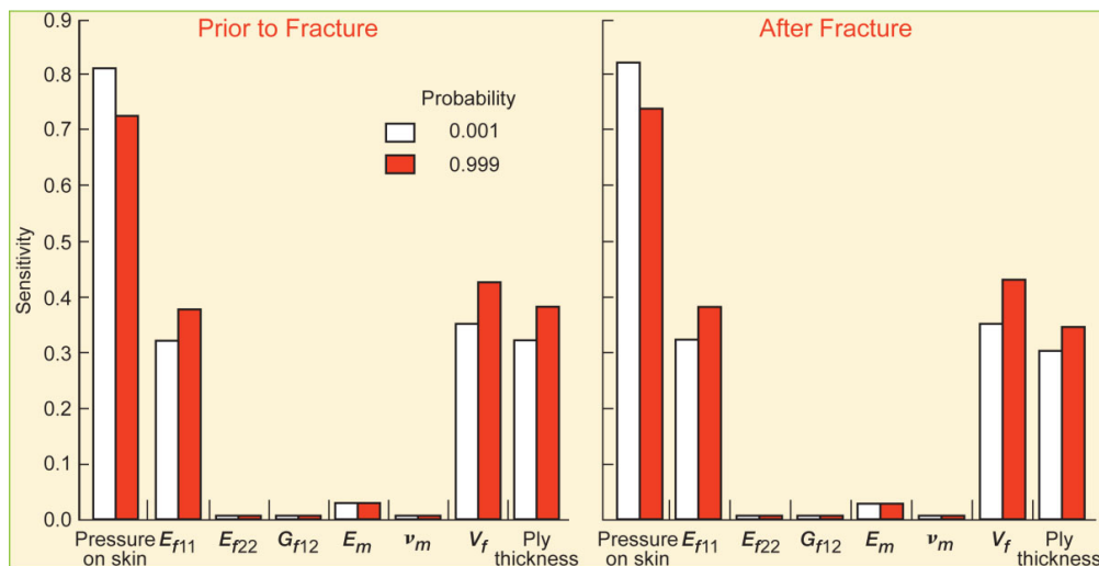
Figure 15.—Composite stiffened panel displacement sensitivity factors.
