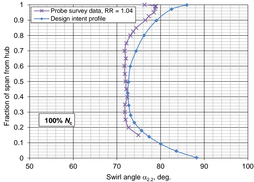
Figure 12.—Comparison of measured flow angle from 3-hole probe at Station 2.2 and pre-test CFD at design point (100 percent N_c , \dot{m}_{c,ex} = 3 lb m /s).
