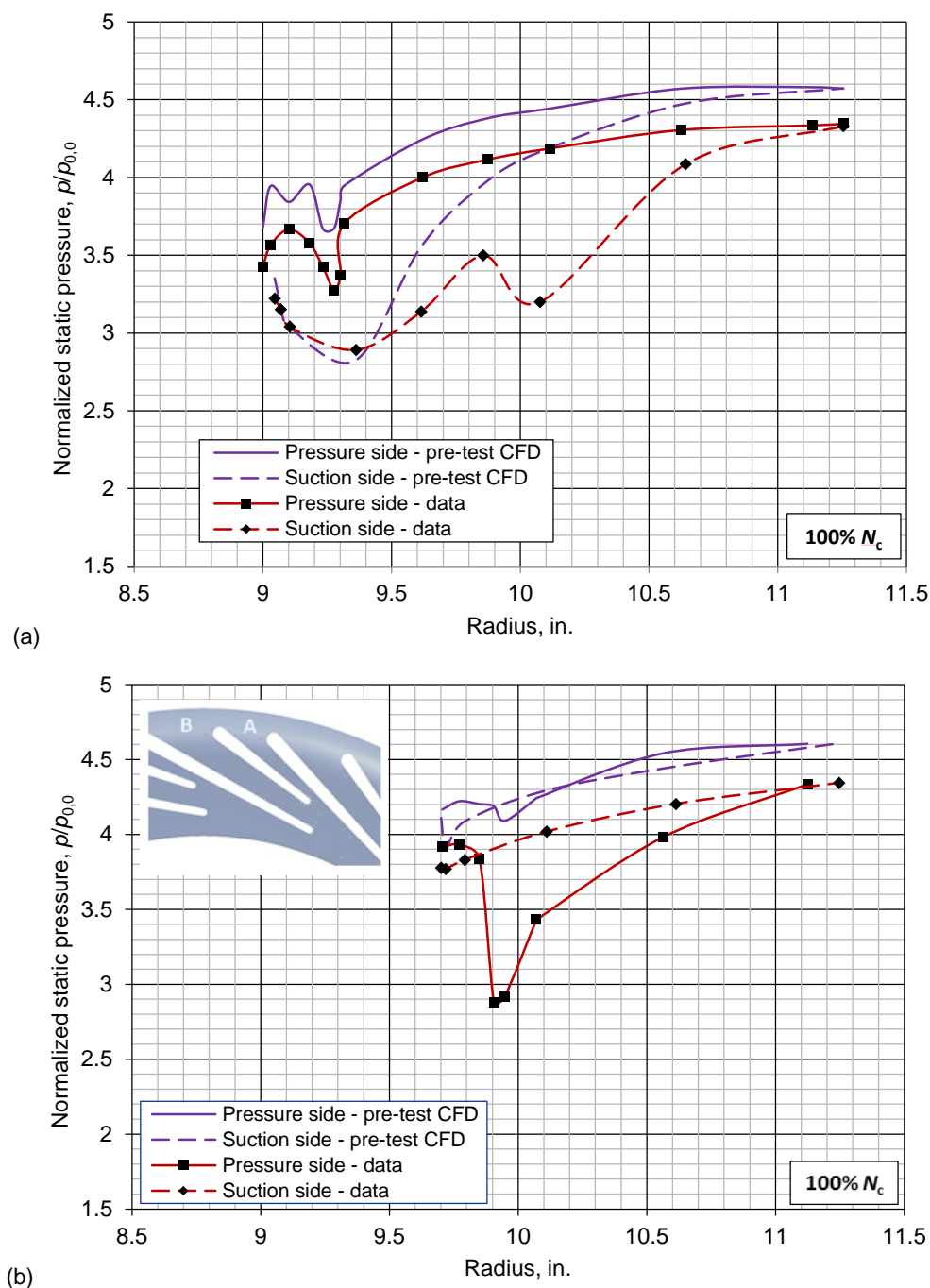
Figure 17.—Comparison of predicted and measured loading diagrams (normalized static pressure versus radius) at the shroud on (a) diffuser main vane and (b) splitter vane, at near design-point operation (11 lb m /s, 100 percent N_c ).
