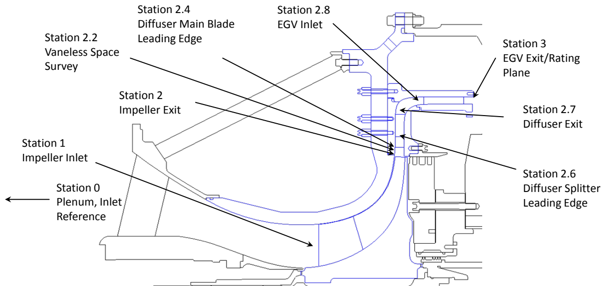
Figure 4.—Compressor Measurement Stations
