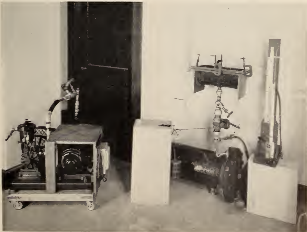
FIGURE 2.—Vacuum-concussion apparatus.
