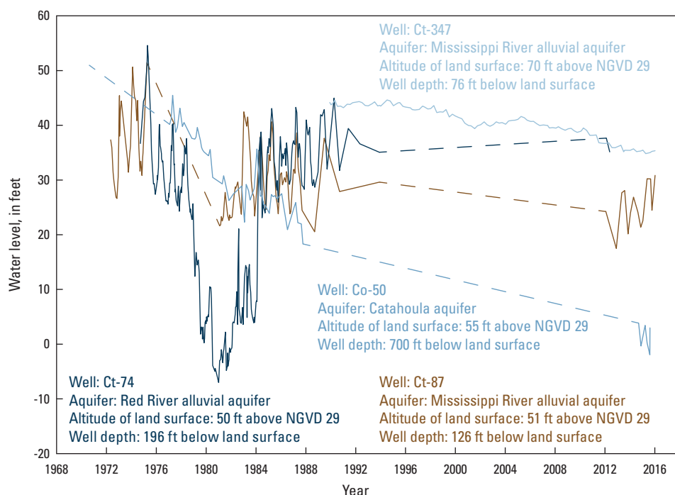
Figure 4. Water levels in well Ct-87 and Ct-347 screened in the Mississippi River alluvial aquifer, well Ct-74 screened in the Red River alluvial aquifer, and well Co-50 screened in the Catahoula aquifer in Catahoula and Concordia Parishes, Louisiana (see fig. 1 for well locations; U.S. Geological Survey, 2016). Land surface and water levels are in feet (ft) relative to the National Geodetic Vertical Datum of 1929 (NGVD 29). Dashed lines indicate gaps in available data.
