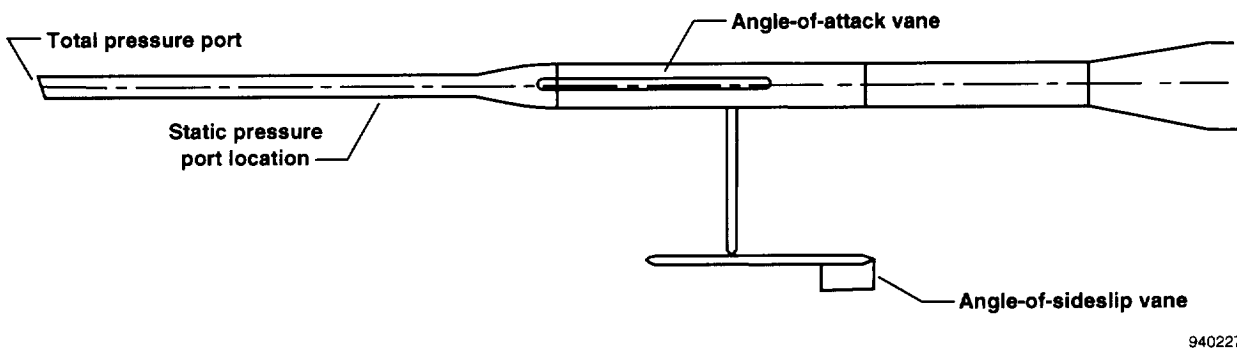
Figure 2. Noseboom for measuring pitot and flow angles.
