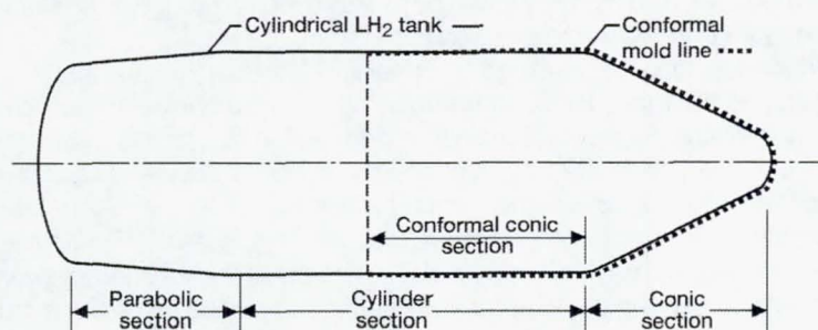
Figure 4.—Liquid hydrogen tank.
