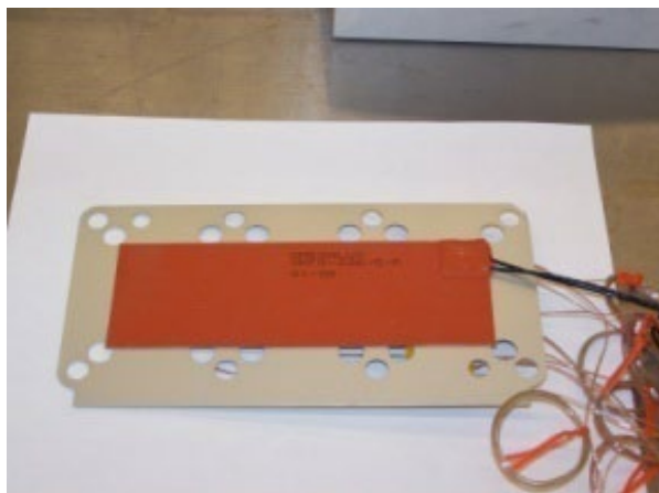
Figure 12.—Fuel cell cooling plate with pad heater.
