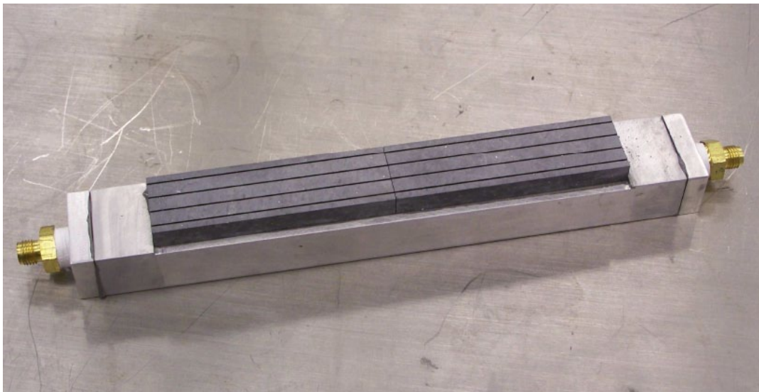
Figure 11.—Single-sided plastic/aluminum heat exchanger.
