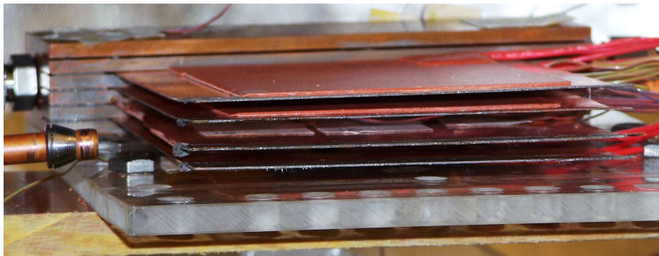
Figure 6.—Heat exchanger with inserted cooling plates.
