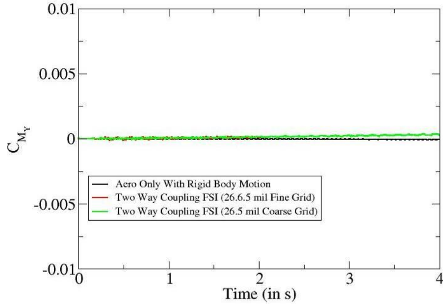
Figure 59. History of side moment coefficient in the y-direction during the aeroelastic dynamic simulation for coarse and fine grids
