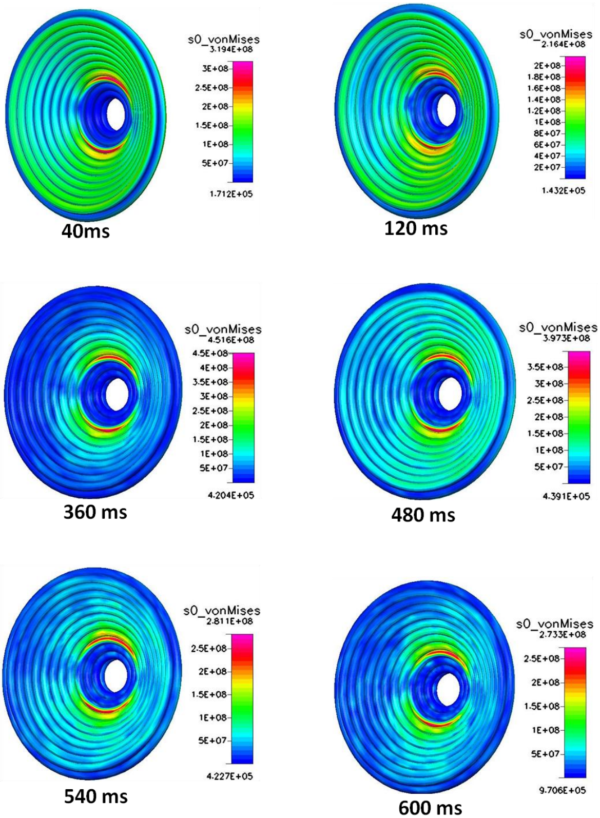
Figure 49. Snapshots of von Mises stresses on the back surface of the toroids
