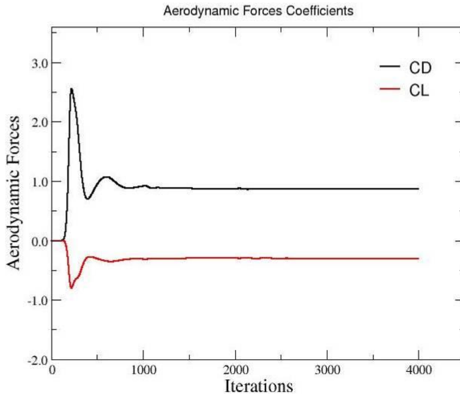
Figure 21. History of lift and drag coefficients
