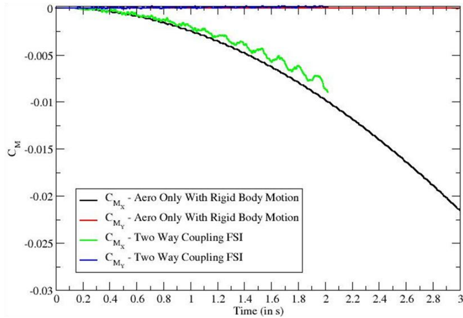
Figure 40. History of side moment coefficients during the aeroelastic dynamic simulation
