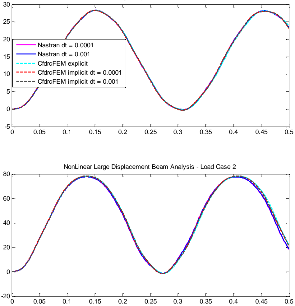
Figure A.2 Dynamic Large Displacement Analysis Results, Beam
