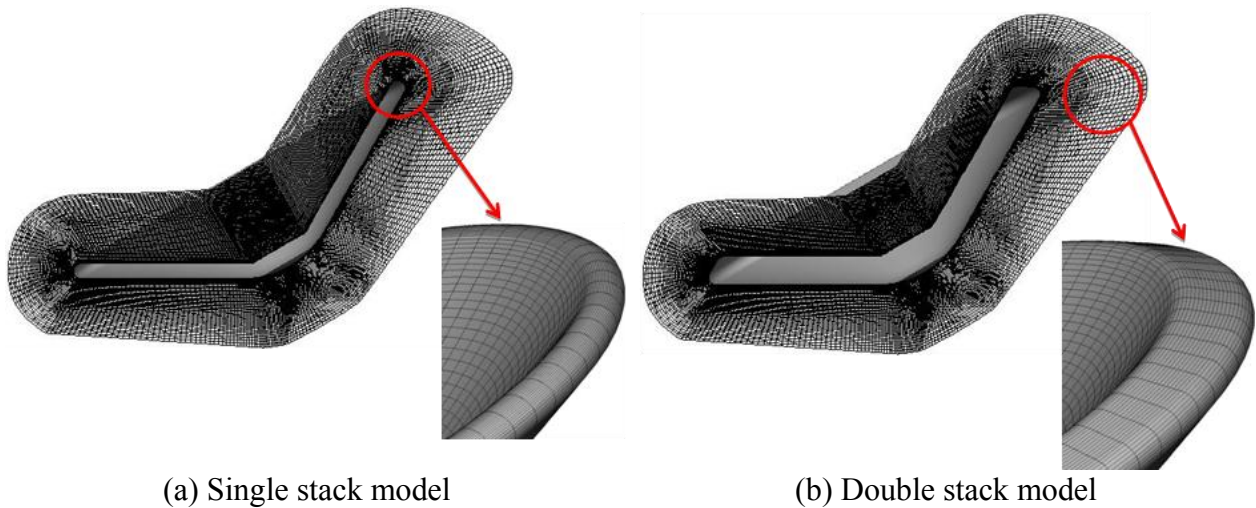
Figure 84 Single and double stack CFD models
