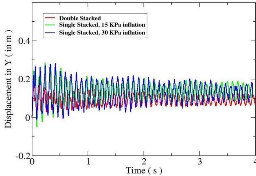
Figure 90 Comparison of y-component of structural deformation for double and single stack configurations with two different inflation pressures.
