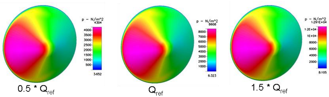
Figure 116 Pressure contours on the front surface of the single stack IAD model
