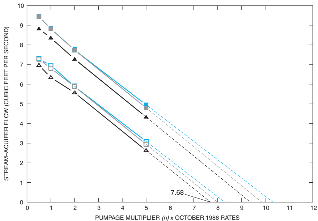
Figure B6. Stream-aquifer flow for simulated pumpage scenarios, groundwater boundary conditions, and stream stage at October 1986, Q_{90} , and Q_{50} levels for reach 6, Mill Creek, Georgia (see fig. 8 for location).
