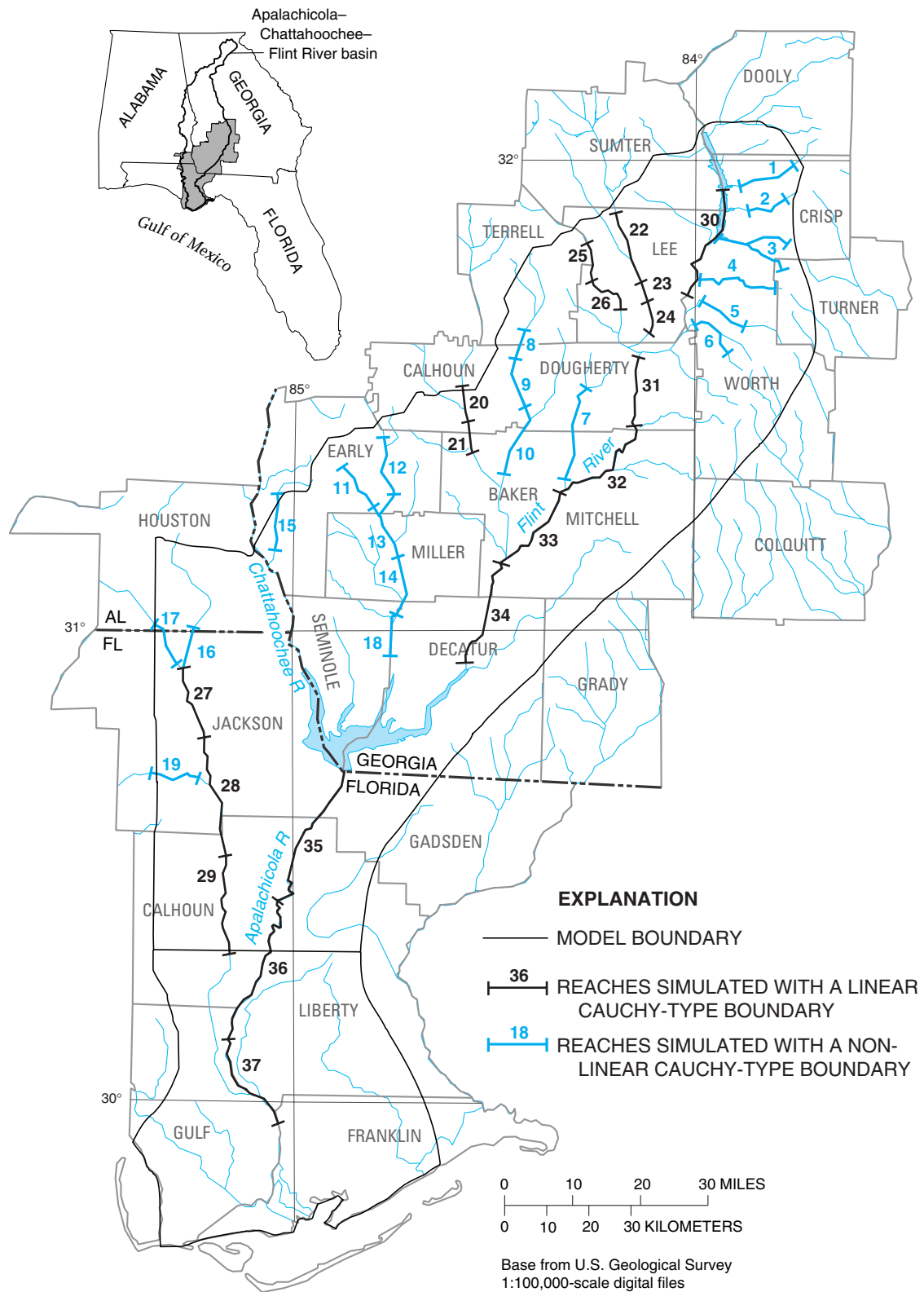
Figure 8. Model boundary and simulated stream reaches for Subarea 4, lower Apalachicola–Chattahoochee–Flint River basin (modified from Torak and McDowell, 1996).
