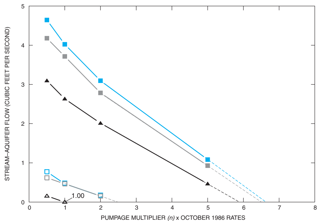
Figure B7. Stream-aquifer flow for simulated pumpage scenarios, groundwater boundary conditions, and stream stage at October 1986, Q_{90} , and Q_{50} levels for reach 7, Coolewahee Creek, Georgia (see fig. 8 for location).
