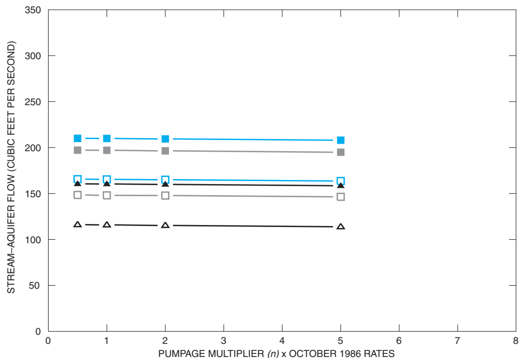
Figure B36. Stream-aquifer flow for simulated pumpage scenarios, ground-water boundary conditions, and stream stage at October 1986, Q_{90} , and Q_{50} levels for reach 36, Apalachicola River, Florida (see fig. 8 for location).
