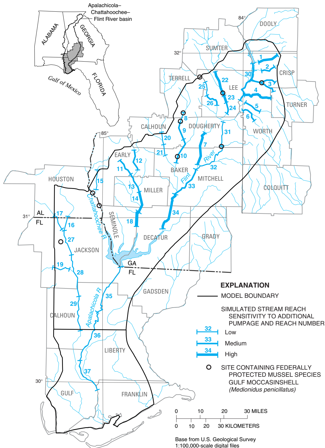
Figure 11. Model boundary and simulated stream reach sensitivities for the lower Apalachicola–Chattoahoochee–Flint River basin (modified from Torak and McDowell, 1996) and sites containing federally protected mussel species Gulf moccasinshell ( Medionidus penicillatus ) (Amy J. Benson, U.S. Geological Survey, written commun., 2000; Paul M. Johnson, Joseph W. Jones Ecological Research Center, written commun., 1999).
