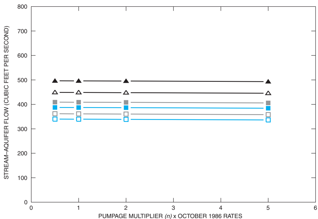
Figure B29. Stream-aquifer flow for simulated pumpage scenarios, groundwater boundary conditions, and stream stage at October 1986, Q_{90} , and Q_{50} levels for reach 29, Chipola River, Florida (see fig. 8 for location).
