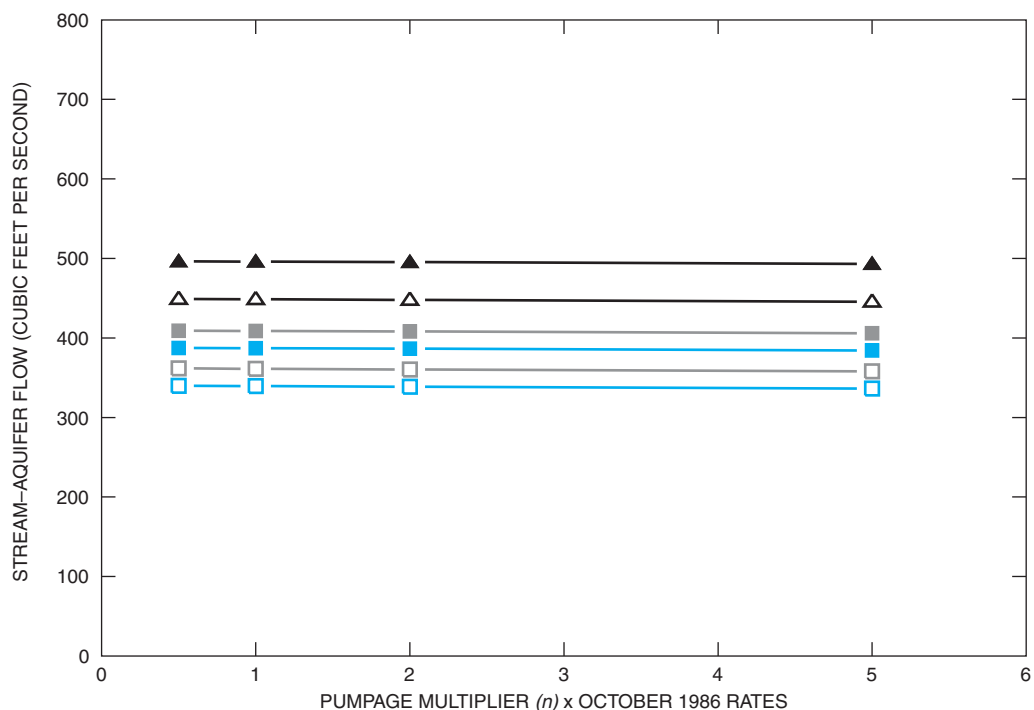
Figure B28. Stream-aquifer flow for simulated pumpage scenarios, groundwater boundary conditions, and stream stage at October 1986, Q_{90} , and Q_{50} levels for reach 28, Chipola River, Florida (see fig. 8 for location).
