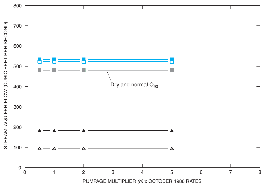
Figure B37. Stream-aquifer flow for simulated pumpage scenarios, ground-water boundary conditions, and stream stage at October 1986, Q_{90} , and Q_{50} levels for reach 37, Apalachicola River, Florida (see fig. 8 for location).
