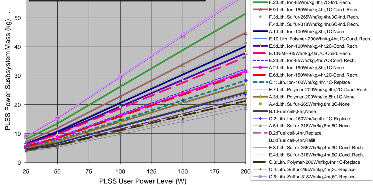
Figure 4: PLSS Power Subsystem Power vs Mass
