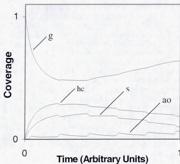
Fig. 4 – Evolution of fractional coverage for species.
