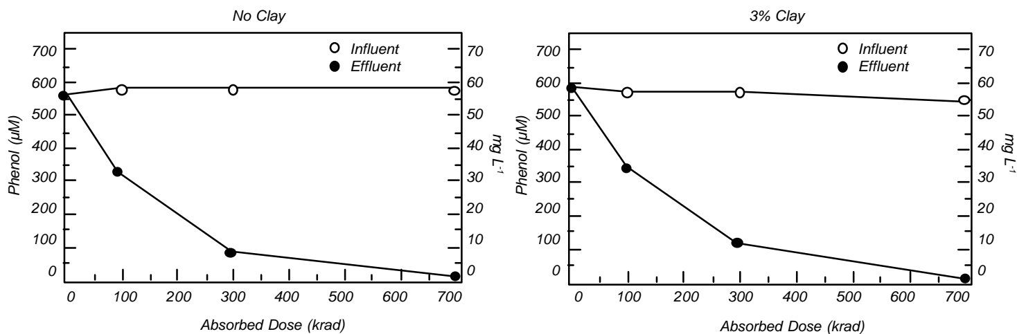
Figure 1. Removal of phenol in the presence and absence of inert solids ( 3% clay) using the electron beam treatment process.
