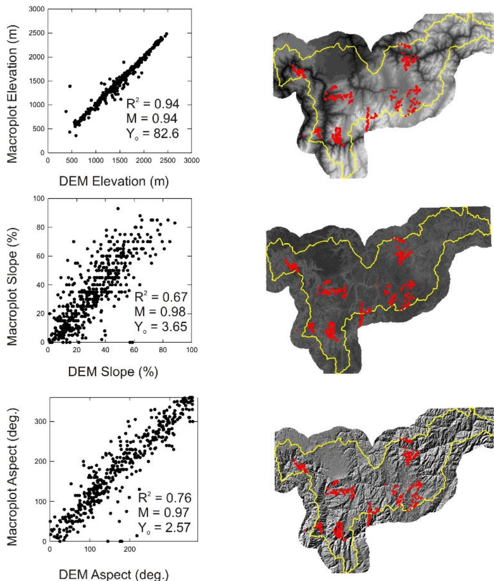
Figure 14— Topographic parameters measured at each macroplot on the SRSA compared with values extracted from the DEM and DEM derivatives. See caption for figure 9 for description of R^2 , M , and Y_o .
