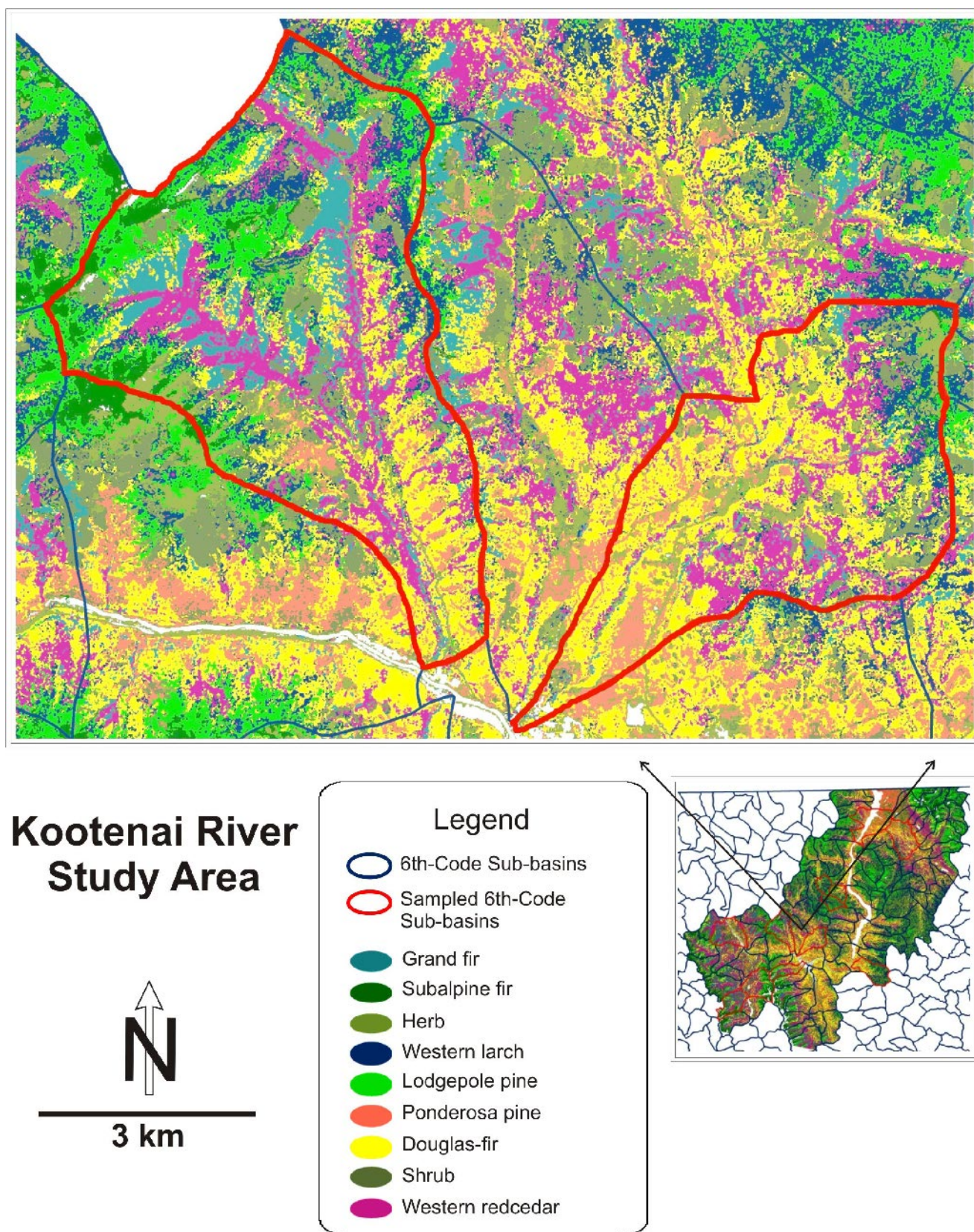
Figure 6 —A closeup of landscape polygons in the KRSA. Landscape polygons represent ecologically distinct units within the study areas. Wall-to-wall coverage of landscape polygons was used to extrapolate simulated weather and ecophysiological variables over the entire extent of each study area. The inset shows the distribution of landscape polygons over the entire KRSA.
