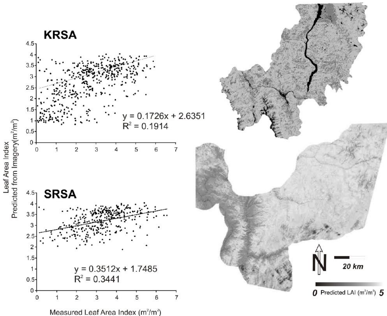
Figure 15 —Predicted versus measured leaf area index ( \text{m}^2 leaf area per \text{m}^2 ground area). Maps are of LAI predicted using satellite imagery along with the modified normalized vegetation index method from Nemani and others (1993). Both models underpredicted LAI.
