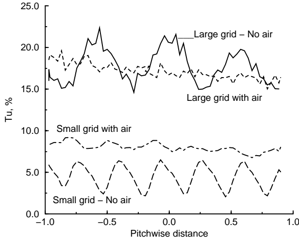
Fig. 11 Turbulence intensity upstream of vane row.
