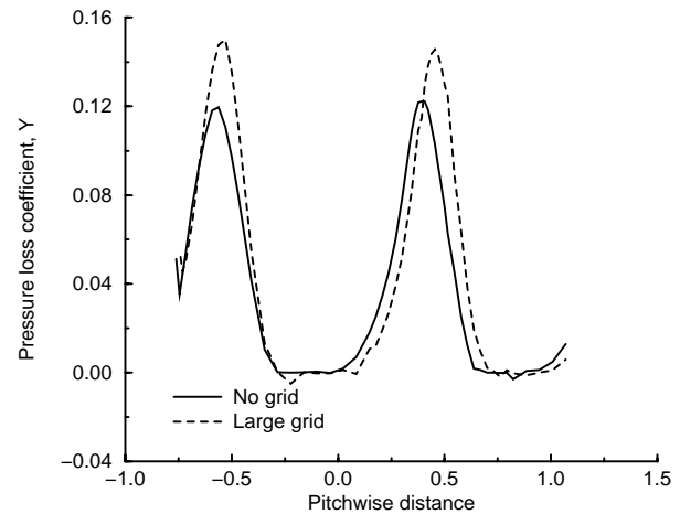
Fig. 5 Wake profile at M_2=0.9 , P_i=0.68 atm.
