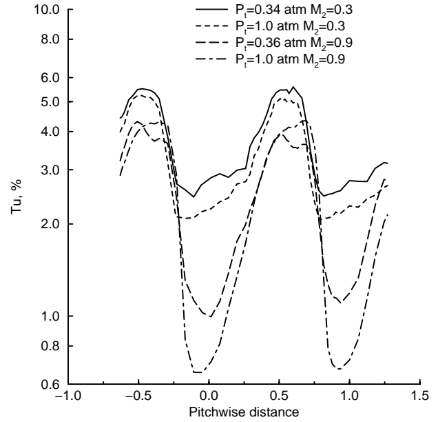
Fig. 12 Turbulence intensity downstream of vane row.
