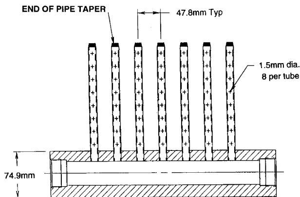
Fig. 2 Turbulence generator.
