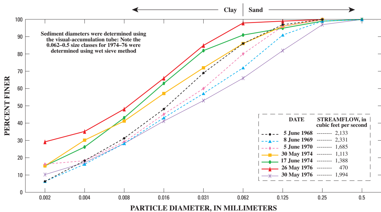
Figure 15. Distribution of particle size in suspended-sediment samples collected at U.S. Geological Survey streamflow-gaging station 12318500 on the Kootenai River at Copeland, Idaho, 1968–76.
