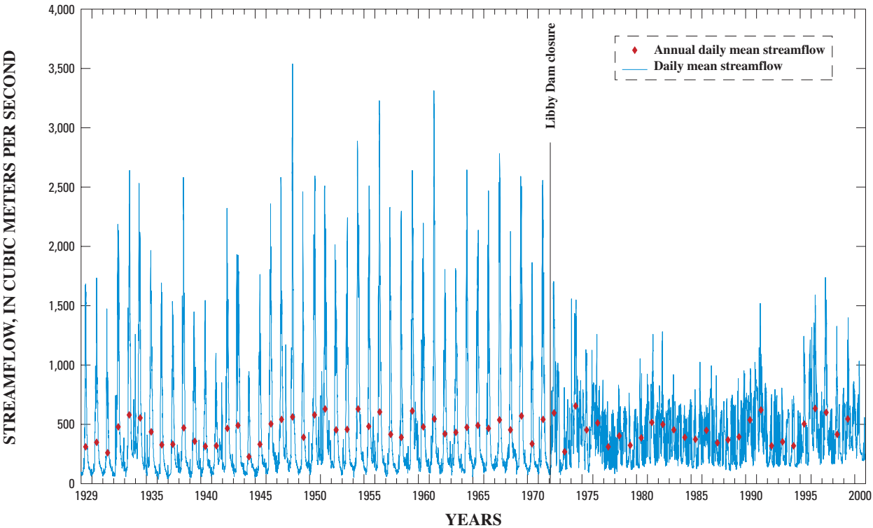
Figure 10. Streamflow at U.S. Geological Survey streamflow-gaging station 12322000 on the Kootenai River at Porthill, Idaho, 1929–2000.
