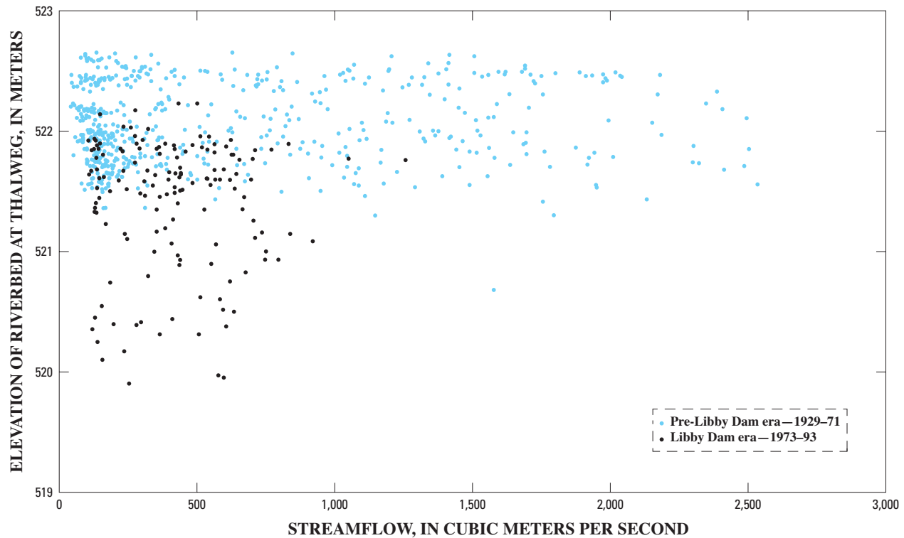
Figure 17. Fluctuation of minimum riverbed elevation with streamflow for the pre-Libby Dam and Libby Dam eras on the Kootenai River beneath the stationary cableway at U.S. Geological Survey streamflow-gaging station 12318500 at Copeland, Idaho, 1929–93.
