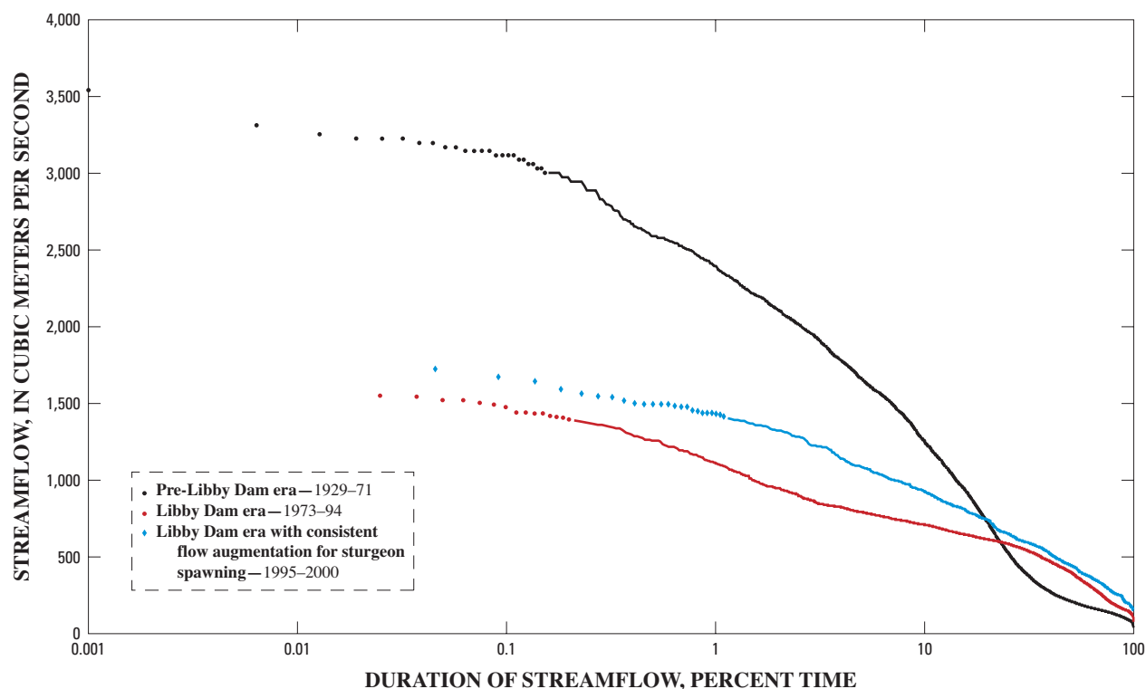
Figure 13. Comparison of the duration for daily mean flows during the pre-Libby Dam era and Libby Dam era at U.S. Geological Survey streamflow-gaging station 12322000 on the Kootenai River at Porthill, Idaho, 1929–2000.
