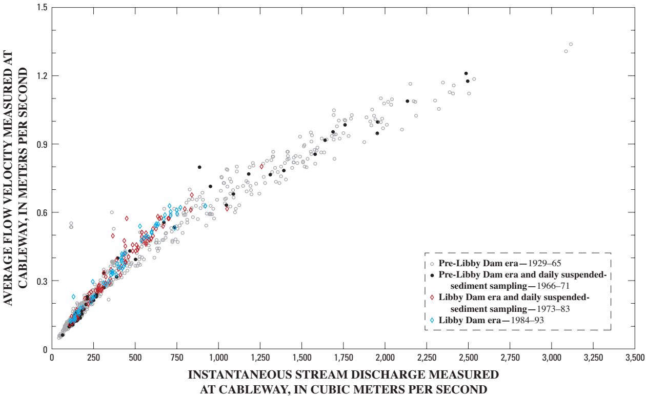
Figure 11. Relation between stream discharge and streamflow velocity at U.S. Geological Survey streamflow-gaging station 12318500 on the Kootenai River at Copeland, Idaho, 1929–93.
