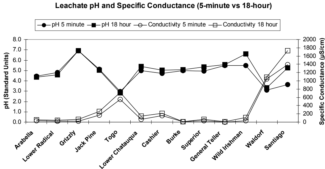
Figure 2. Comparison of leachate pH and specific conductance data (5 minute and 18 hour) for 13 mine-wastes included in this study.
