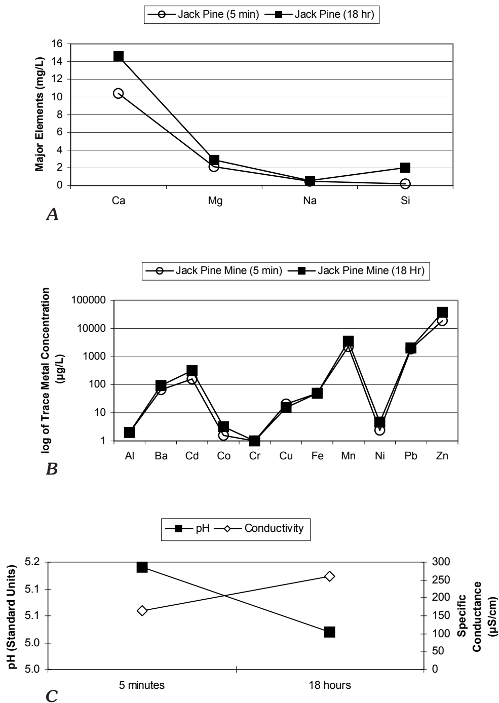
Figure 14. Jack Pine mine-waste leachate geochemistry trends (5 minutes vs. 18 hours) for A , selected major elements (ICP-AES); B , selected trace metals (ICP-MS); and C , pH and specific conductance .
