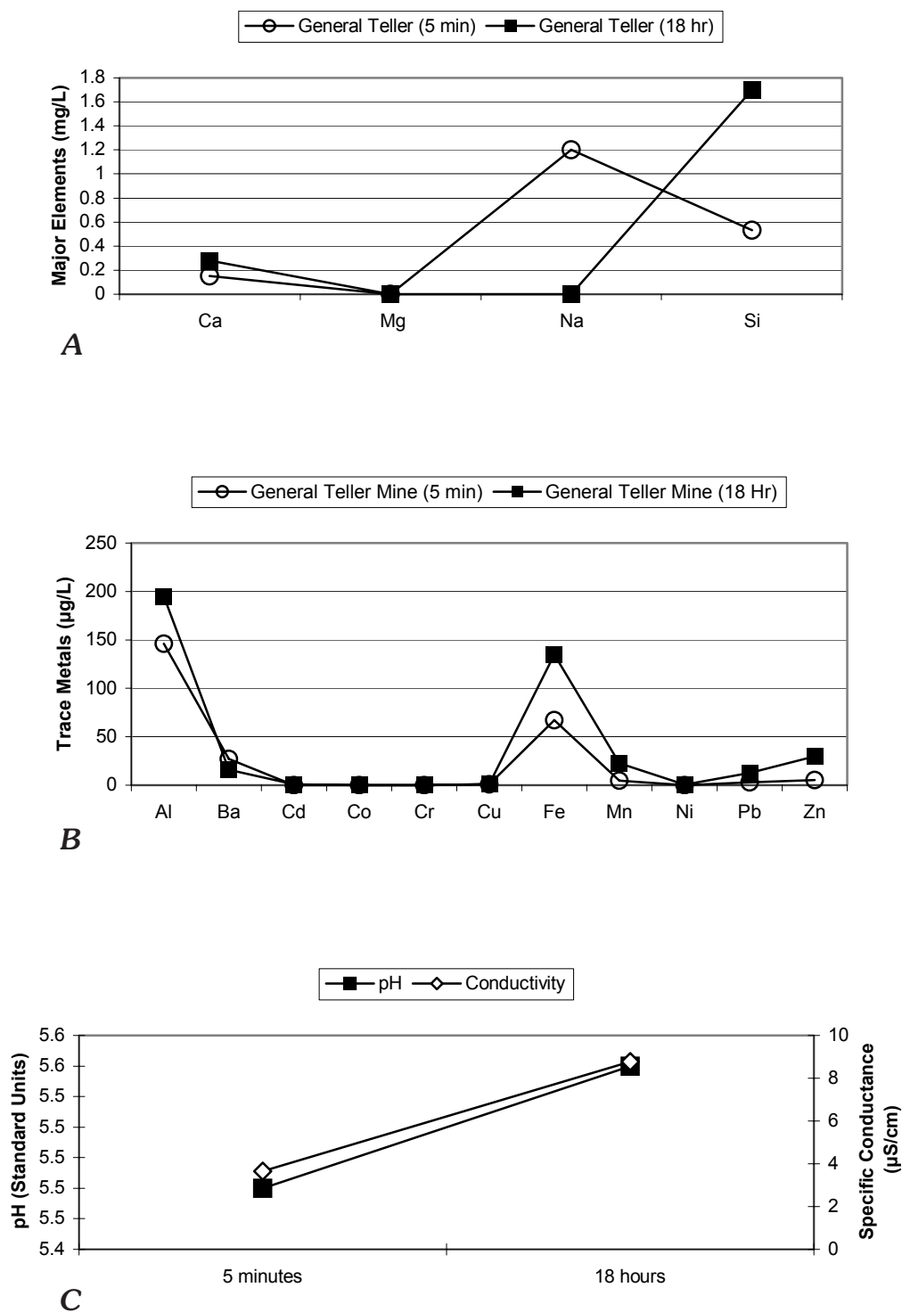
Figure 7. General Teller mine-waste leachate geochemistry trends (5 minutes vs. 18 hours) for A , selected major elements (ICP-AES); B , selected trace metals (ICP-MS); and C , pH and specific conductance.
