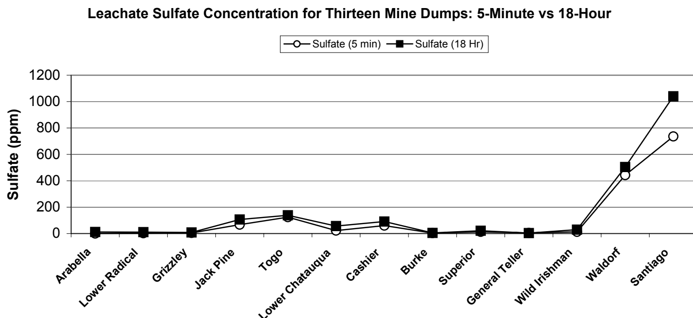
Figure 3. Comparison of leachate sulfate data (5 minute and 18 hour) for 13 mine-wastes included in this study.
