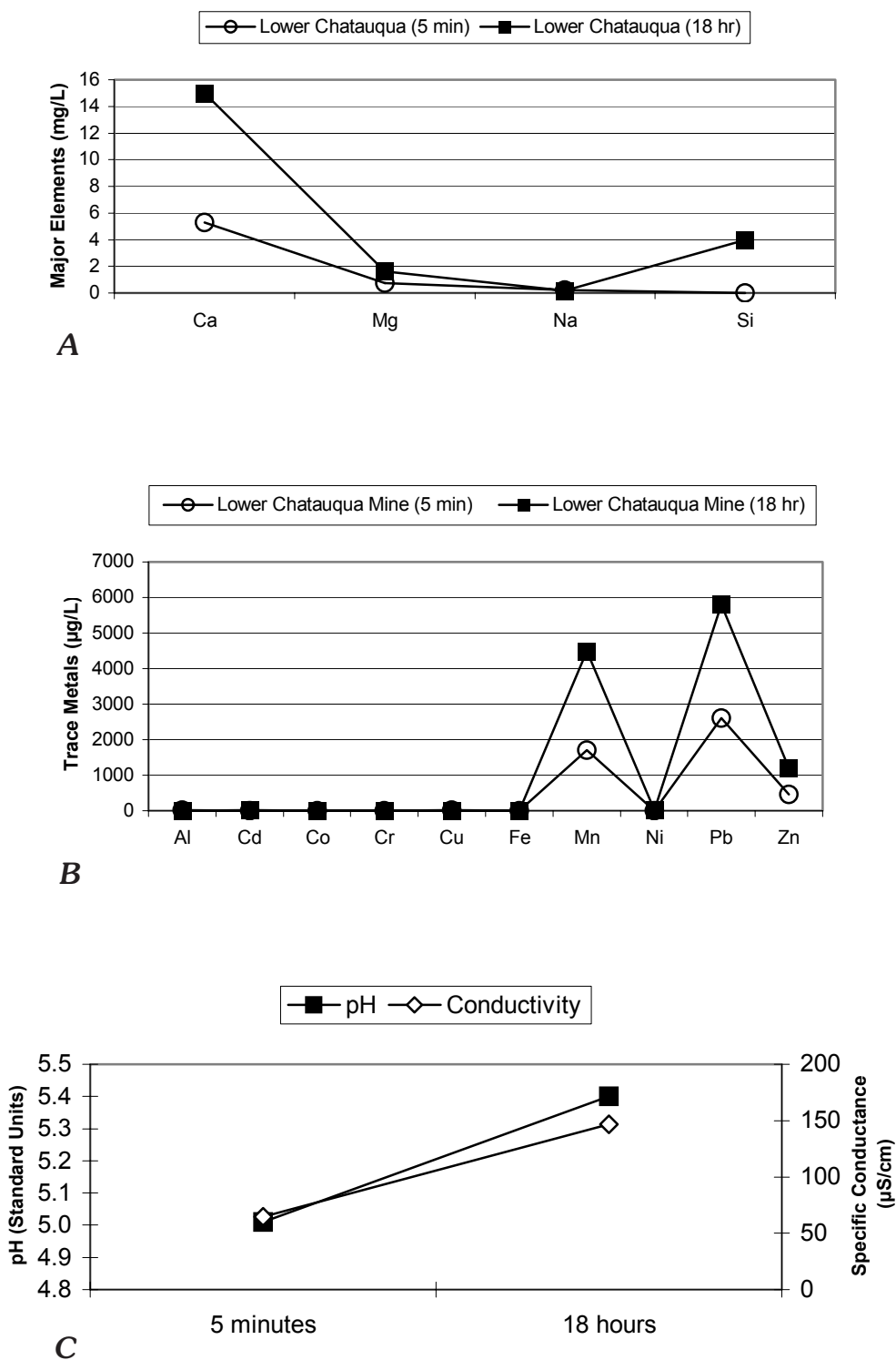
Figure 6. Lower Chatauqua mine-waste leachate geochemistry trends (5 minutes vs. 18 hours) for A , selected major elements (ICP-AES); B , selected trace metals (ICP-MS); and C , pH and specific conductance.
