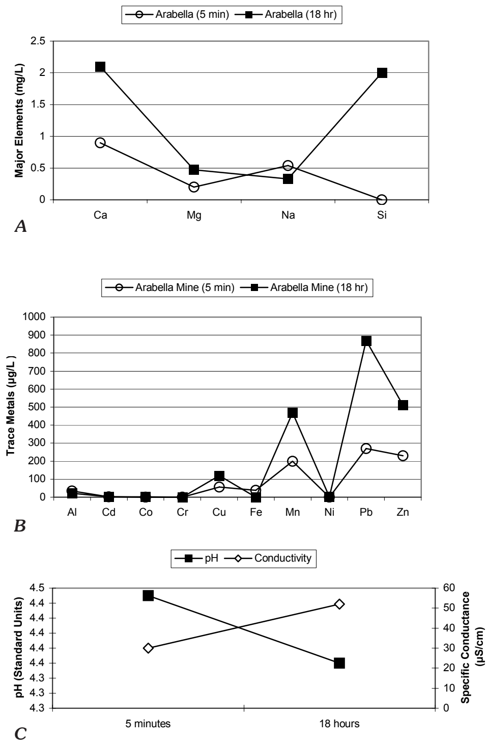
Figure 4. Arabella mine-waste leachate geochemistry trends (5 minutes vs. 18 hours) for A , selected major elements (ICP-AES); B , selected trace metals (ICP-MS); and C , pH and specific conductance.
