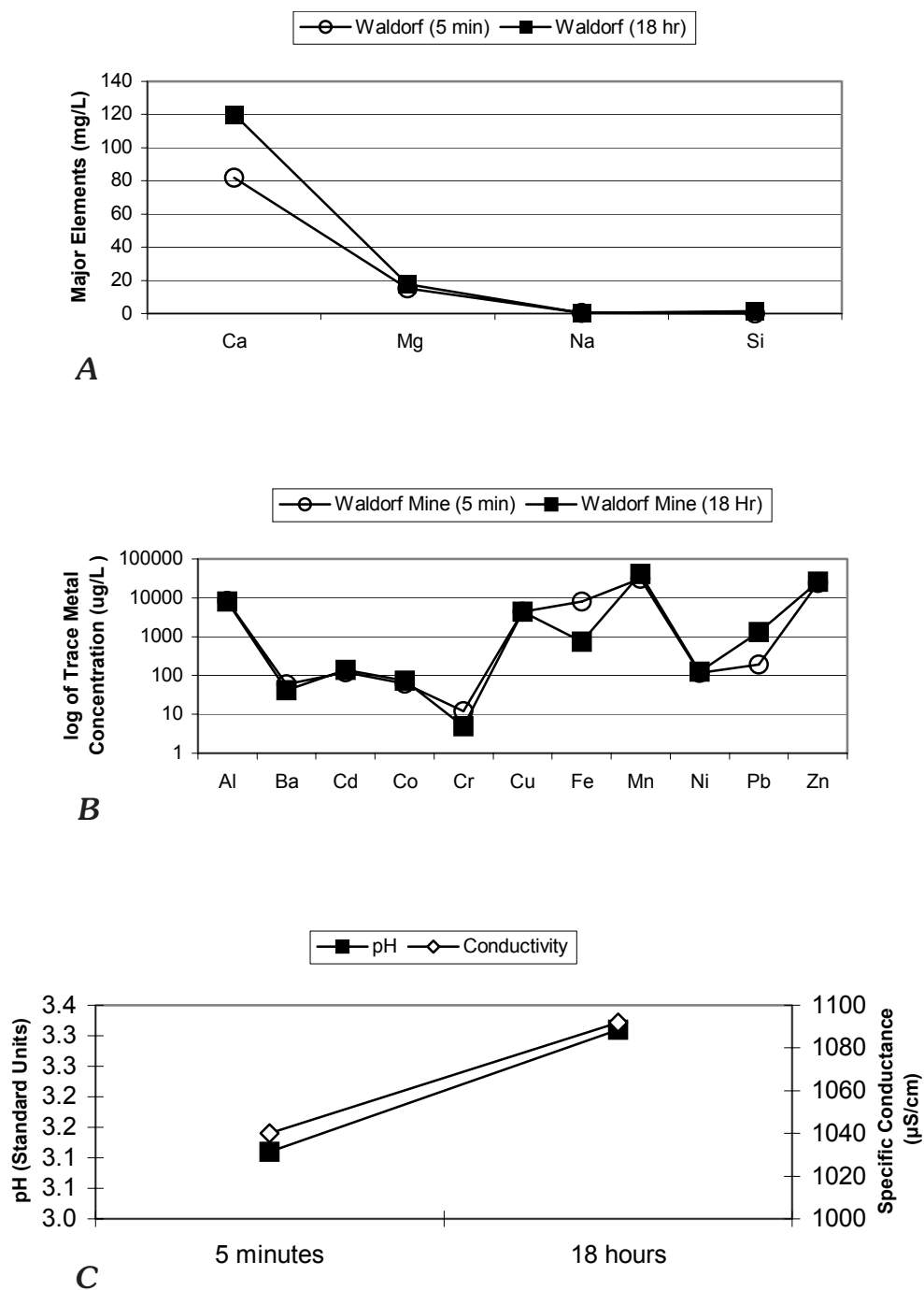
Figure 15. Waldorf mine-waste leachate geochemistry trends (5 minutes vs. 18 hours) for A , selected major elements (ICP-AES); B , selected trace metals (ICP-MS); and C , pH and specific conductance .
