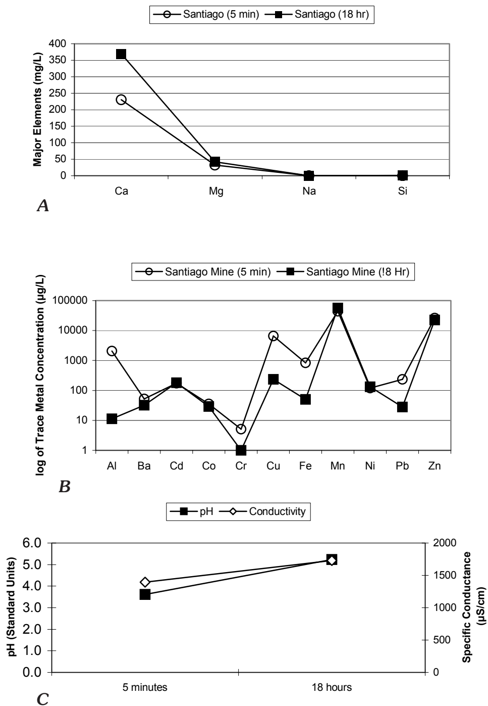
Figure 16. Santiago mine-waste leachate geochemistry trends (5 minutes vs. 18 hours) for A , selected major elements (ICP-AES); B , selected trace metals (ICP-MS); and C , pH and specific conductance.
