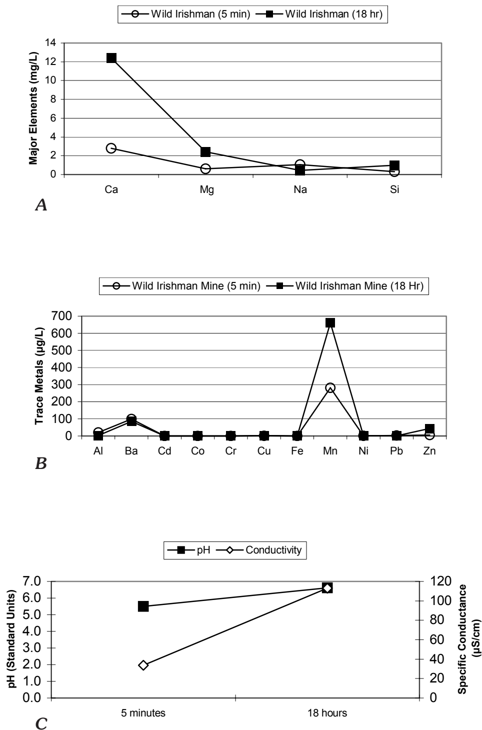
Figure 12. Wild Irishman mine-waste leachate geochemistry trends (5 minutes vs. 18 hours) for A. selected major elements (ICP-AES); B. selected trace metals (ICP-MS); and C. pH and specific conductance .
