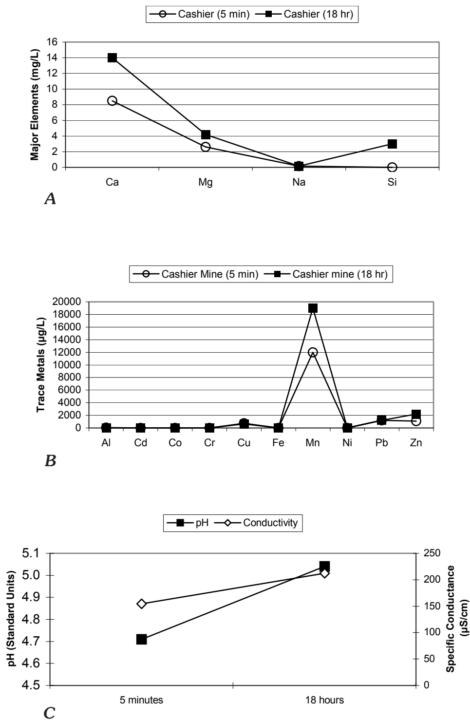
Figure 8. Cashier mine-waste leachate geochemistry trends (5 minutes vs. 18 hours) for A , selected major elements (ICP-AES); B , selected trace metals (ICP-MS); and C , pH and specific conductance.
