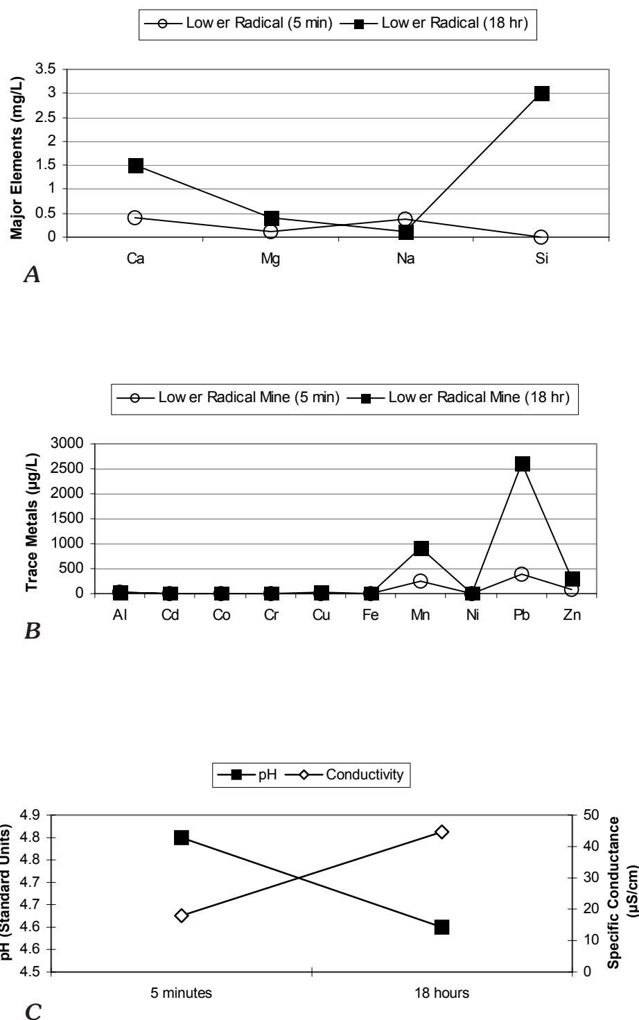
Figure 5. Lower Radical mine-waste leachate geochemistry trends (5 minutes vs. 18 hours) for A , selected major elements (ICP-AES); B , selected trace metals (ICP-MS); and C , pH and specific conductance.
