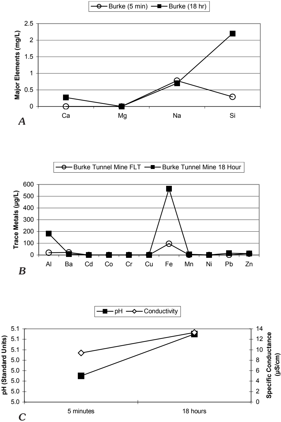
Figure 10. Burke mine-waste leachate geochemistry trends (5 minutes vs. 18 hours) for A , selected major elements (ICP-AES); B , selected trace metals (ICP-MS); and C , pH and specific conductance .
