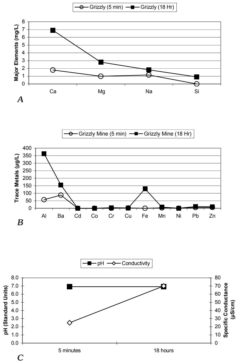
Figure 13. Grizzly mine-waste leachate geochemistry trends (5 minutes vs. 18 hours) for A , selected major elements (ICP-AES); B , selected trace metals (ICP-MS); and C , pH and specific conductance.
