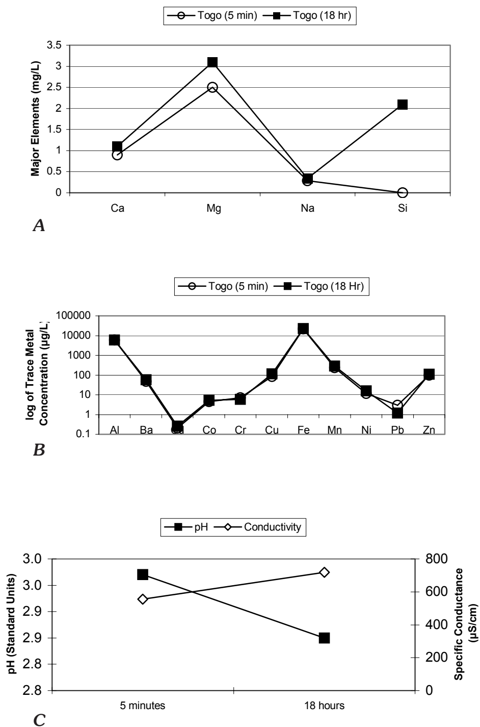
Figure 9. Togo mine-waste leachate geochemistry trends (5 minutes vs. 18 hours) for A , selected major elements (ICP-AES); B , selected trace metals (ICP-MS); and C , pH and specific conductance.
