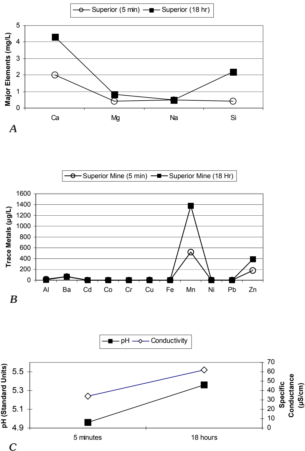
Figure 11. Superior mine-waste leachate geochemistry trends (5 minutes vs. 18 hours) for A , selected major elements (ICP-AES); B , selected trace metals (ICP-MS); and C , pH and specific conductance.
