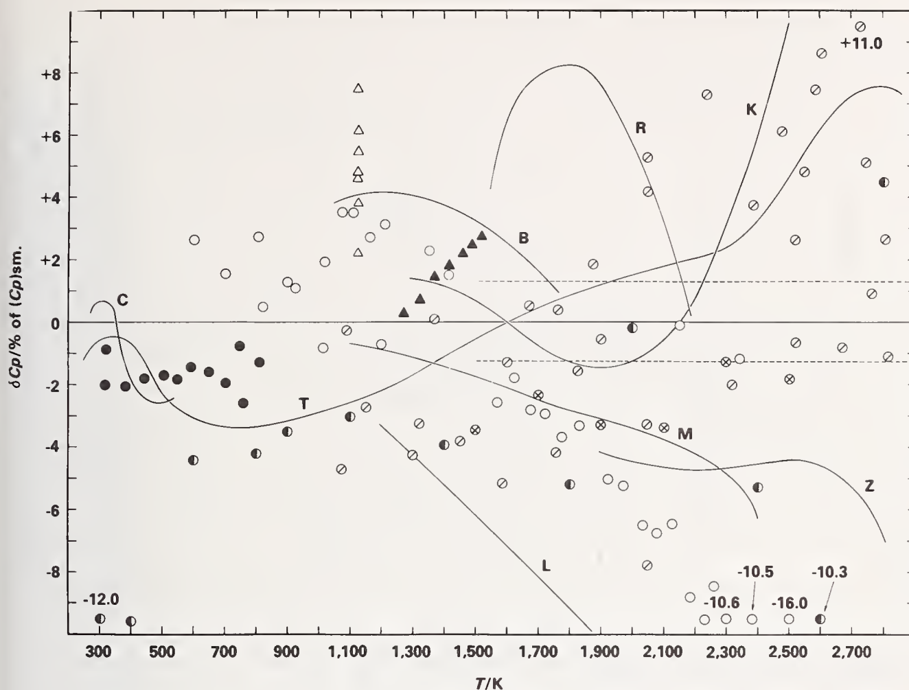
Figure 7. Deviation of directly-measured molybdenum heat-capacity data appearing in the literature from unified spline representation of present NBS data for SRM-781 molybdenum. Baseline is equation (7). Dotted lines indicate limits of dispersion of NBS pulse-calorimetric, heat capacity data. See table 16 for explanation of symbols.
