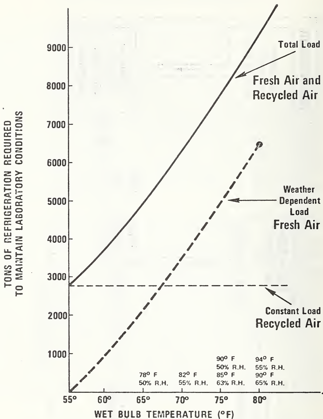
Figure 6. Cooling load (tons of refrigeration) vs wet bulb temperature. (NES, Gaithersburg)
