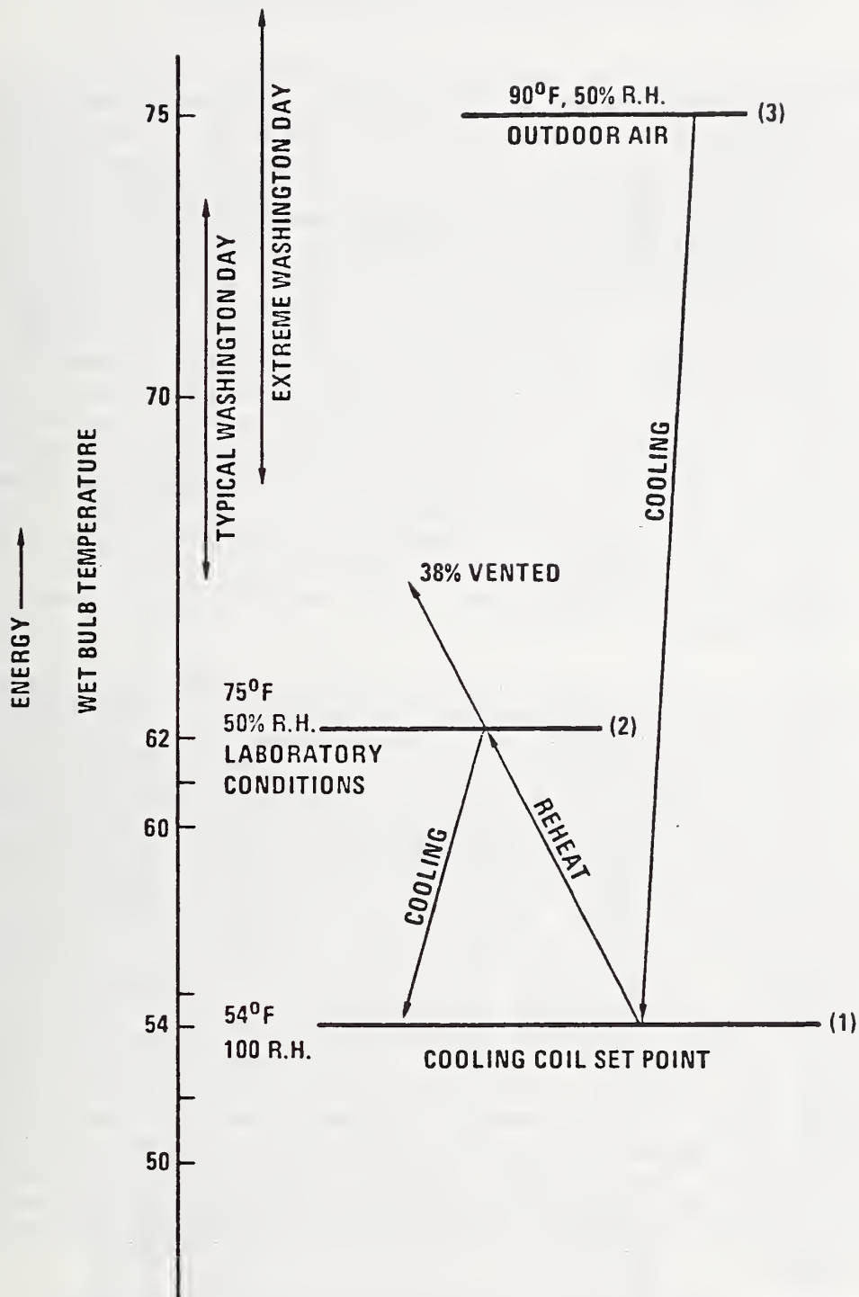
Figure 4. Schematic representation of energy use in humidity control in laboratories. (NBS, Gaithersburg)
