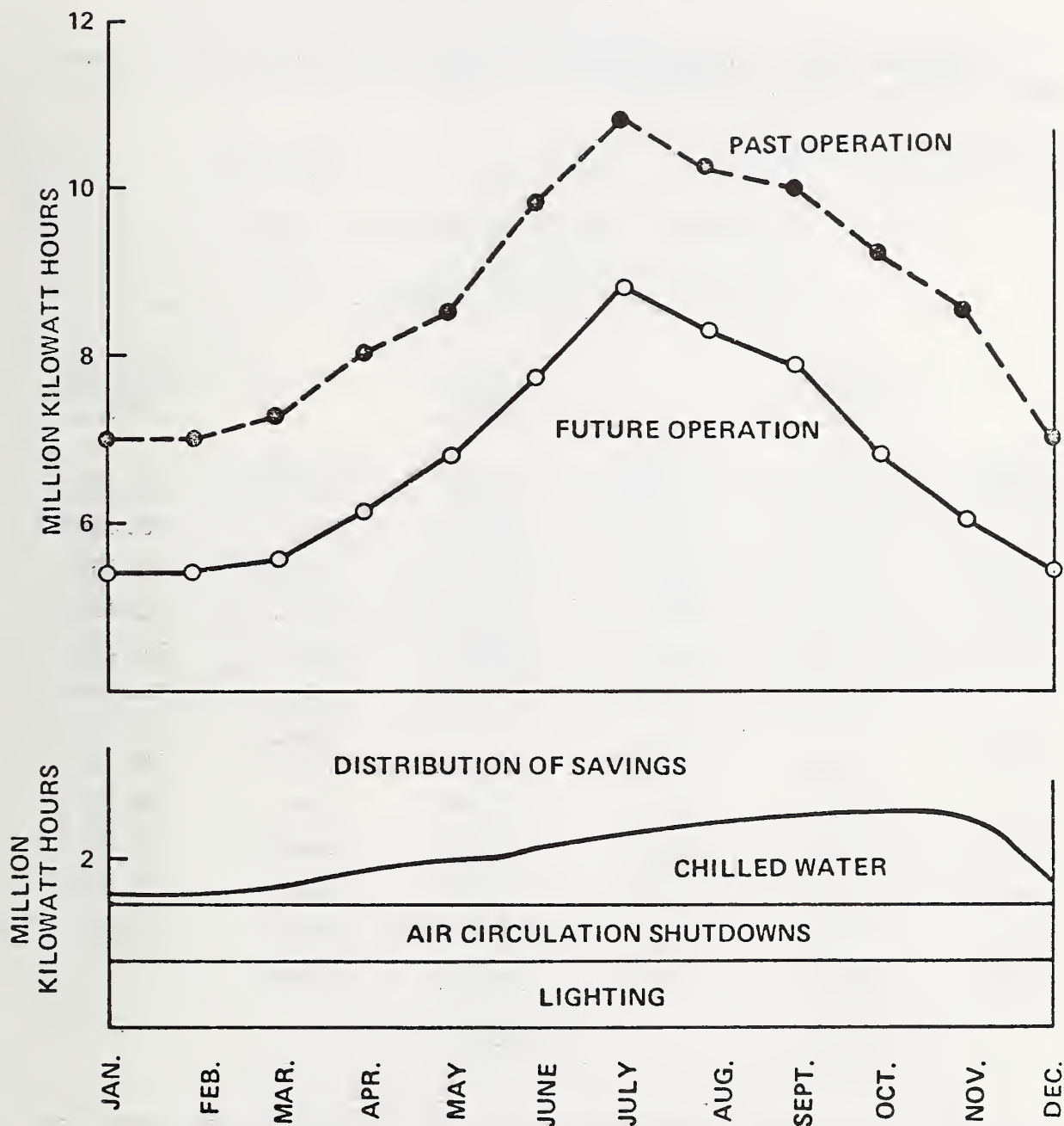
Figure 12. Electricity use: Schematic comparison of past and future operation. (NBS, Gaithersburg)
