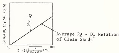
Fig. 27 Definition of DR_d
