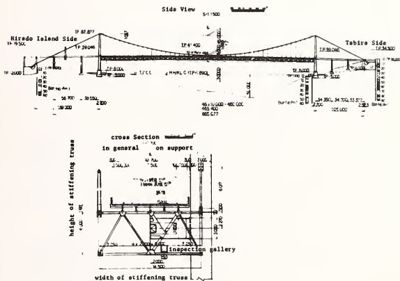
Fig.-2 General View of Hiredo-Ohashi Bridge
