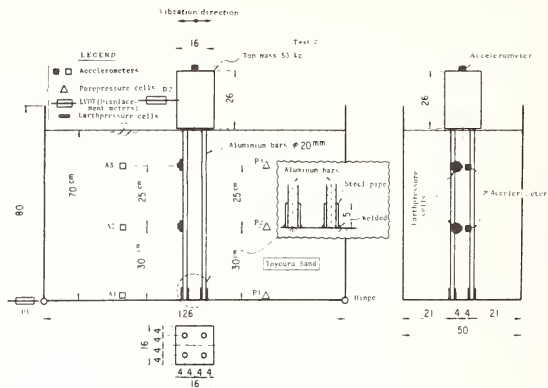
Fig. 2 Test Arrangements for Test 2
