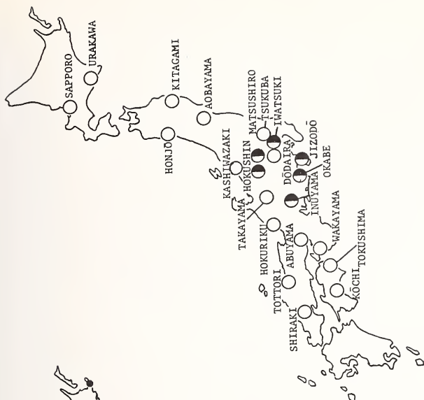
Fig. 10. Microearthquake observatories/stations.
