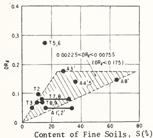
Fig. 28 S - D R_d Relationship
