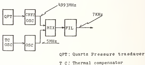
Figure 5-2. Tsunami-meter Block Diagram
