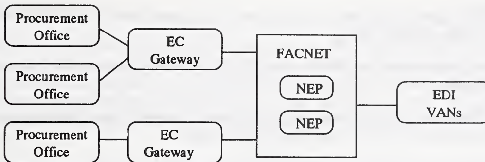
Figure 3: FACNET Architecture.
