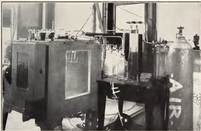
FIGURE 2.— Rear view of apparatus for exposure of paper to sulphur dioxide showing control accessories.
