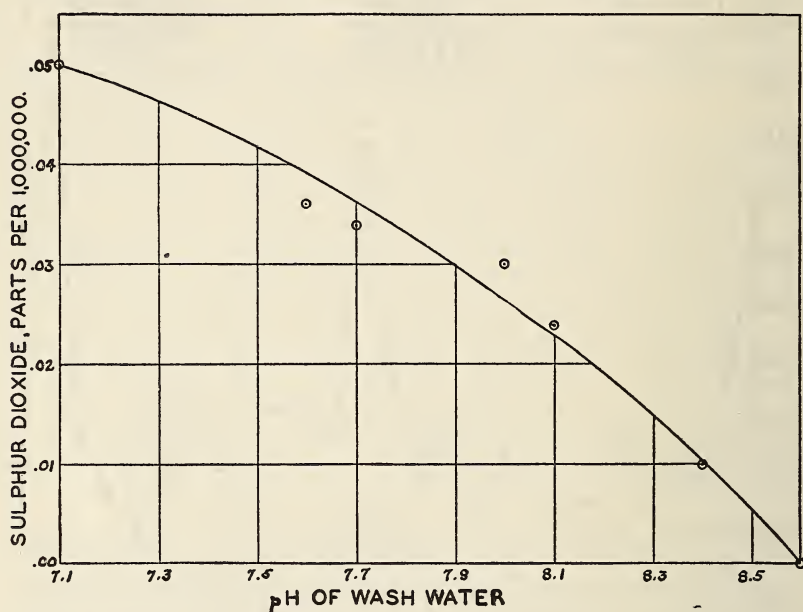
FIGURE 4.—Relationship of the sulphur dioxide content of washed air to the hydrogen-ion concentration of the wash water.
