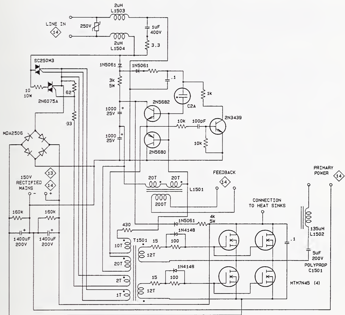
Schematic 15. Main Power Supply - Primary Side.
