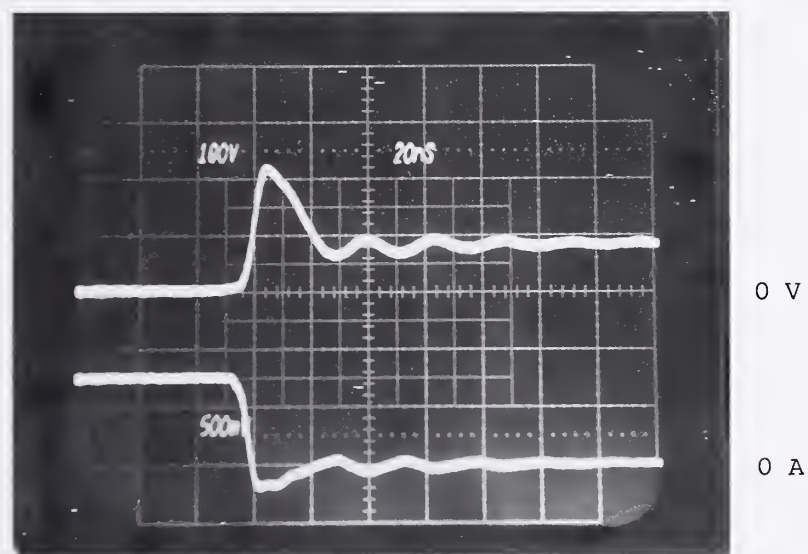
Figure 8. Clamp voltage overshoot (top trace) and current for high-speed device turn-off. The scale factors are 100 V per minor division and 5 A per minor division, vertical axis, and 20 ns per minor division, horizontal axis. The sub 10-ns device turn-off causes the device drain voltage to overshoot the clamp set point by about 280 V. The improved breakdown detection circuit for this tester is able to discriminate between this overshoot and actual breakdown, and does not issue a false trigger signal.
