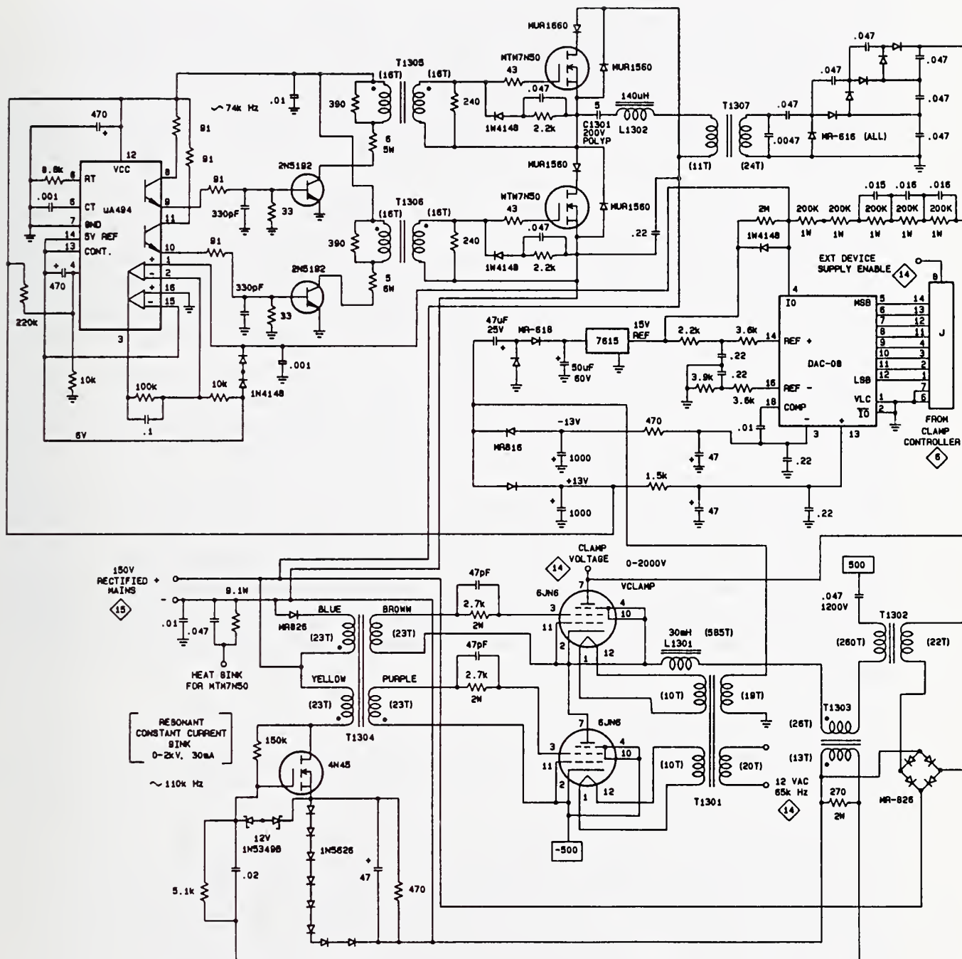
Schematic 13. Clamp Voltage Supply.
