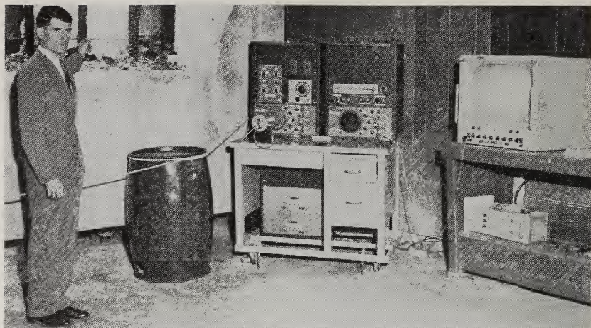
Transient heat-flow analyzer designed to eliminate costly large-scale fire tests by analyzing data about thermal properties of materials (p. 65).
