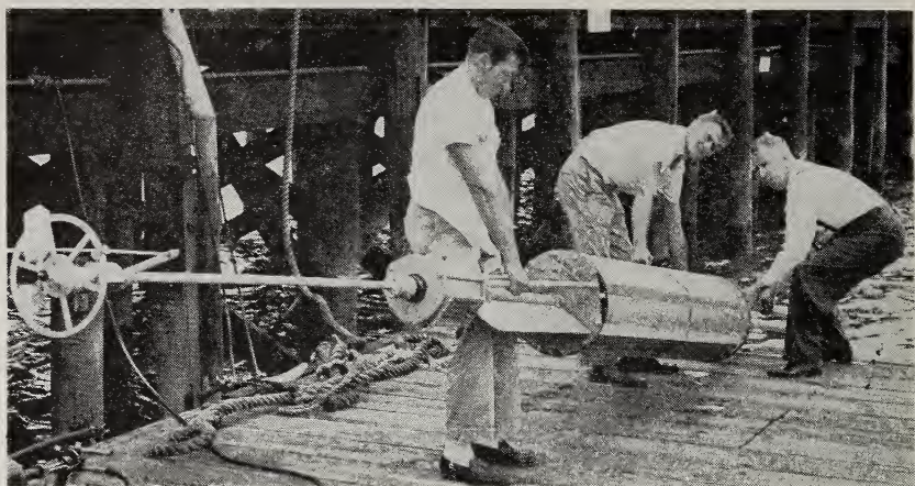
Free-floating weather buoy modified for use as a hurricane-tracking device. The buoy transmits information on weather conditions every 6 hours (p. 15).
