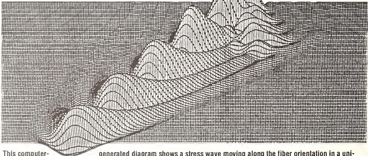
This computer-generated diagram shows a stress wave moving along the fiber orientation in a unidirectional graphite/epoxy composite. Each of the five humps represents one of the periods of the wave and the ripples coming off of these periods.
