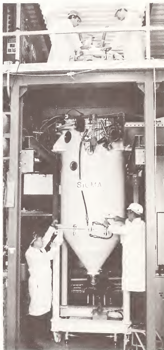
Researchers at NIST prepare for a test run using the supersonic inert gas metal atomizer (SIGMA). Clockwise from bottom left are John Manning, Frank Biancaniello, Stephen Ridder, and James Ingram, a research associate from Hoeganaes Corporation.
