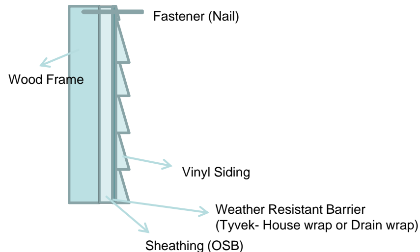
Vinyl siding
