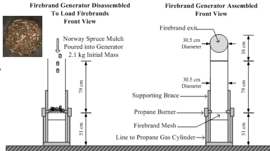
Firebrand Generator Front View
