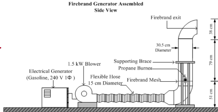
Firebrand Generator Side View
