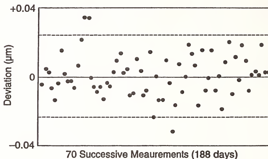
Figure 13. Control chart of feature 1-B. Vertical axis is variation ( \mu\text{m} ) from the mean (solid line); horizontal axis is successive measurements. The dotted lines mark the limits of the 95% confidence level. Future measurements are added to the chart.
