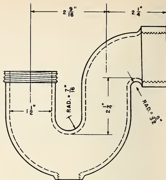
FIGURE 9. 1\frac{1}{2} -inch cast brass trap.
