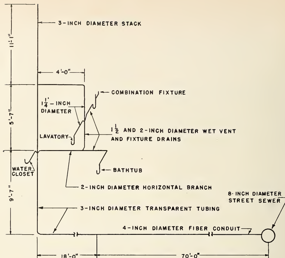
FIGURE 6. Single-story wet-vented system.
