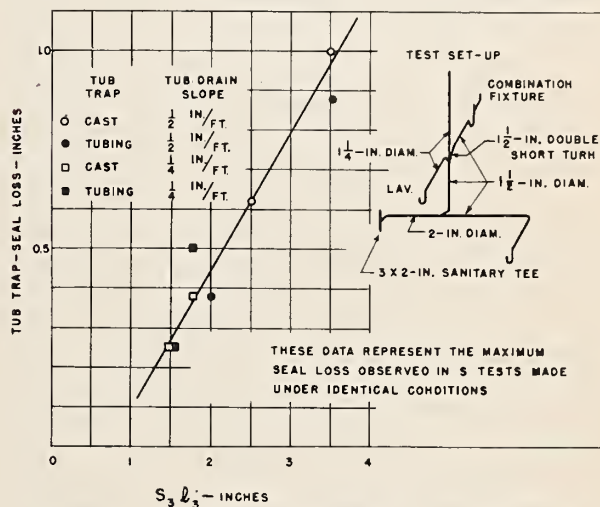
FIGURE 12. Tub trap-seal losses for a constant flow of 15 gpm through the wet vent.
