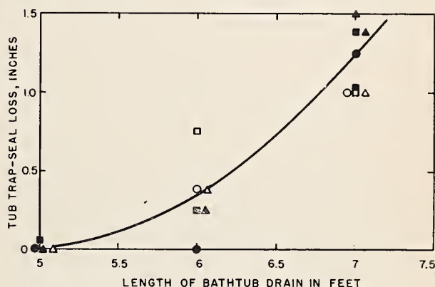
FIGURE 23. Trap-seal losses of a two-story, duplex, wet-vented system.
