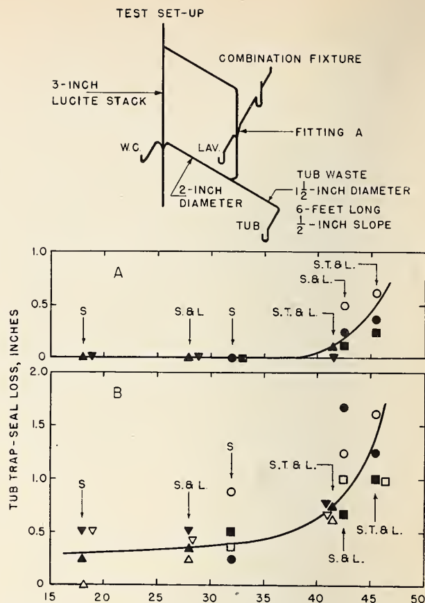
FIGURE 17. Effect of slope of horizontal branch on tub trap-seal reduction.
