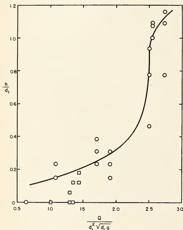
FIGURE 18. Dimensionless plot of wet venting data for test loadings not including the bathtub.
