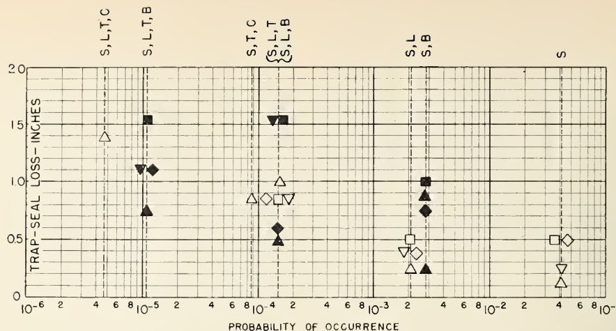
FIGURE 14. Probability of occurrence of various simultaneous discharges.
