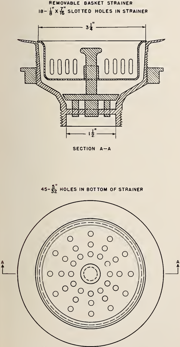
FIGURE 8. Removable basket-type strainer.
