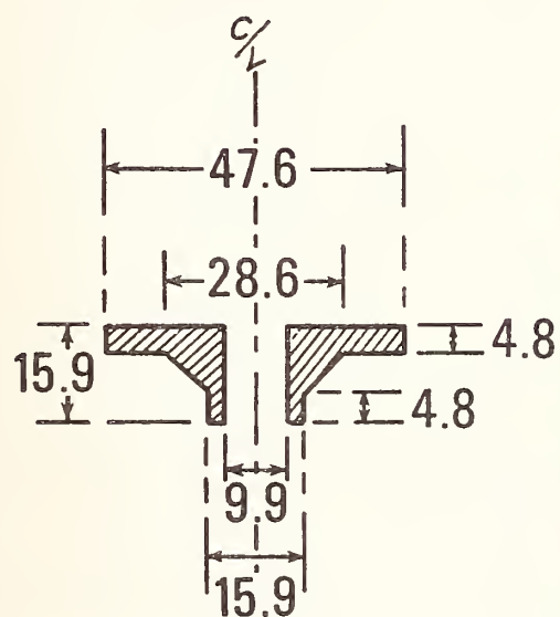
HEAT SHUNT
