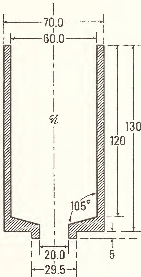
FUNNEL
